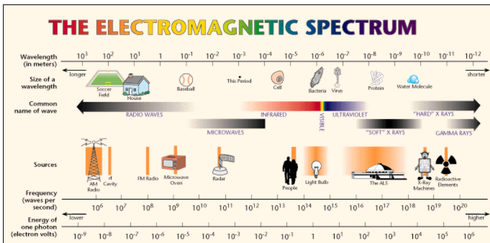
Figure 2. Electromagnetic Spectrum (From [3])
