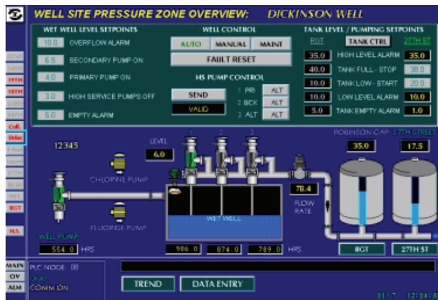
Figure 2. Sample SCADA display (From [5]).
