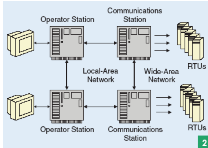
Figure 5. Second-generation SCADA architecture (From [8]).
