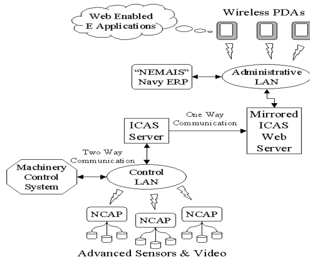
Figure 13. ICAS Incorporation of Wireless Networks (From [75]).
