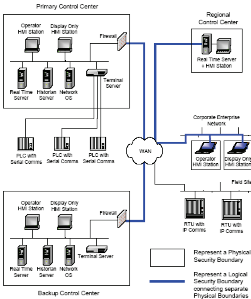
Figure 16. Cyber Security TOE and Security Perimeters for Control Center PP (From [83]).
