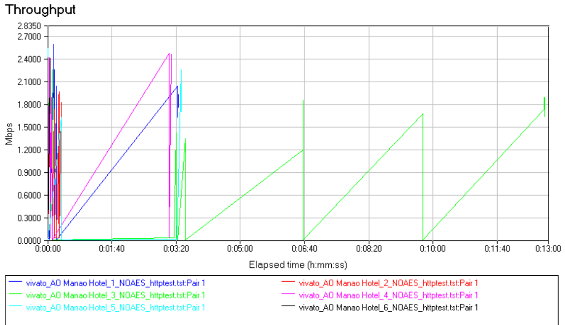
Figure 35. Ao Manao Hotel Throughput without GHOSTNet.
