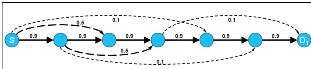
Figure 13. Opportunistic Routing From [40]
