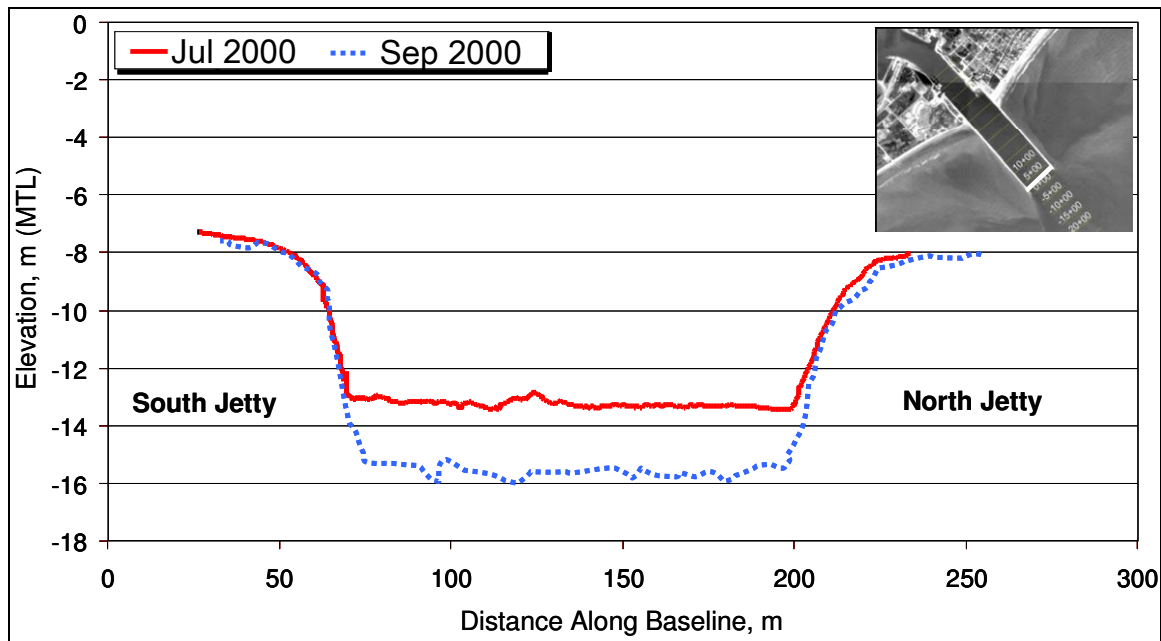
Figure 7. Freepoint Entrance Channel, TX, channel cross-section at jetty tips.
