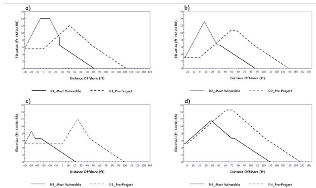
Figure 6. Most vulnerable without-project morphology: (a) Reach 1; (b) Reach 2; (c) Reach 3; and (d) Reach 4.
