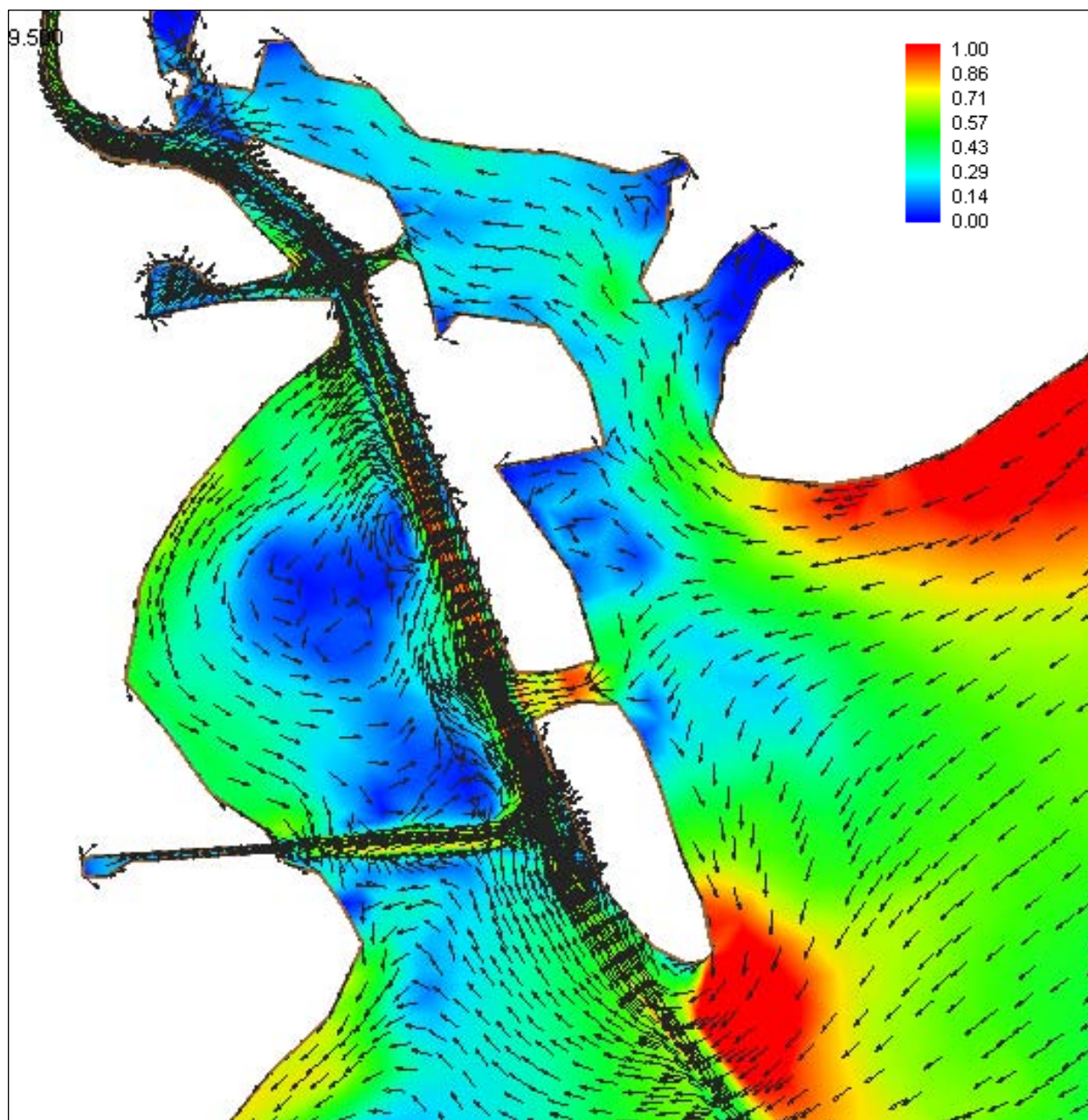
Figure 42. Velocity magnitude and direction at hour 10709.5 for extension 2 (ft/s).
