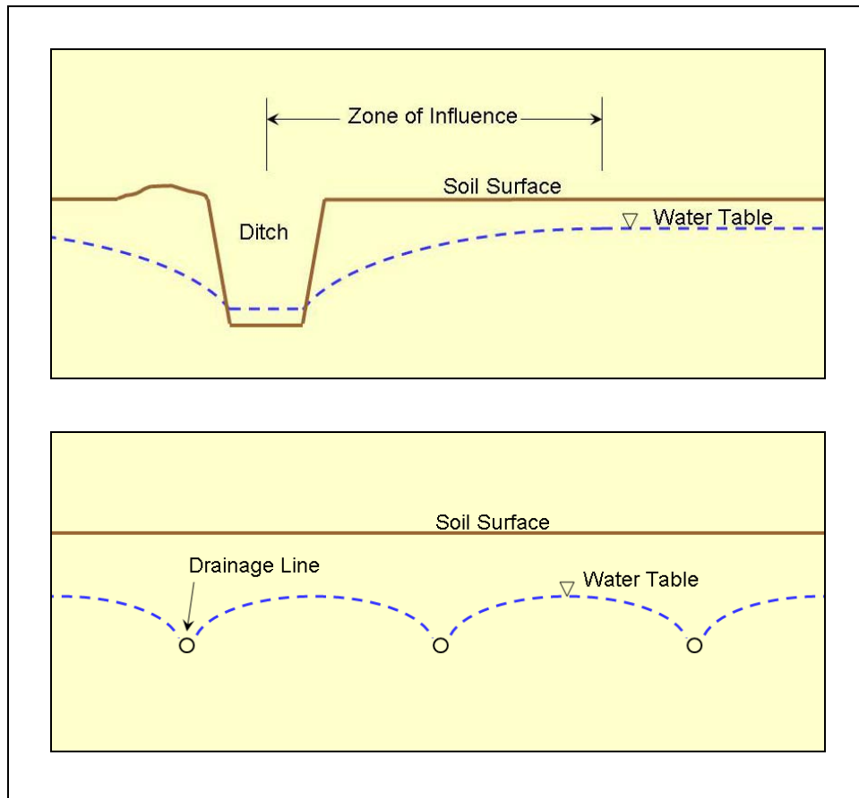
Figure 51. Effects of ditches (upper) and parallel subsurface drainage lines (lower) on the water table.
