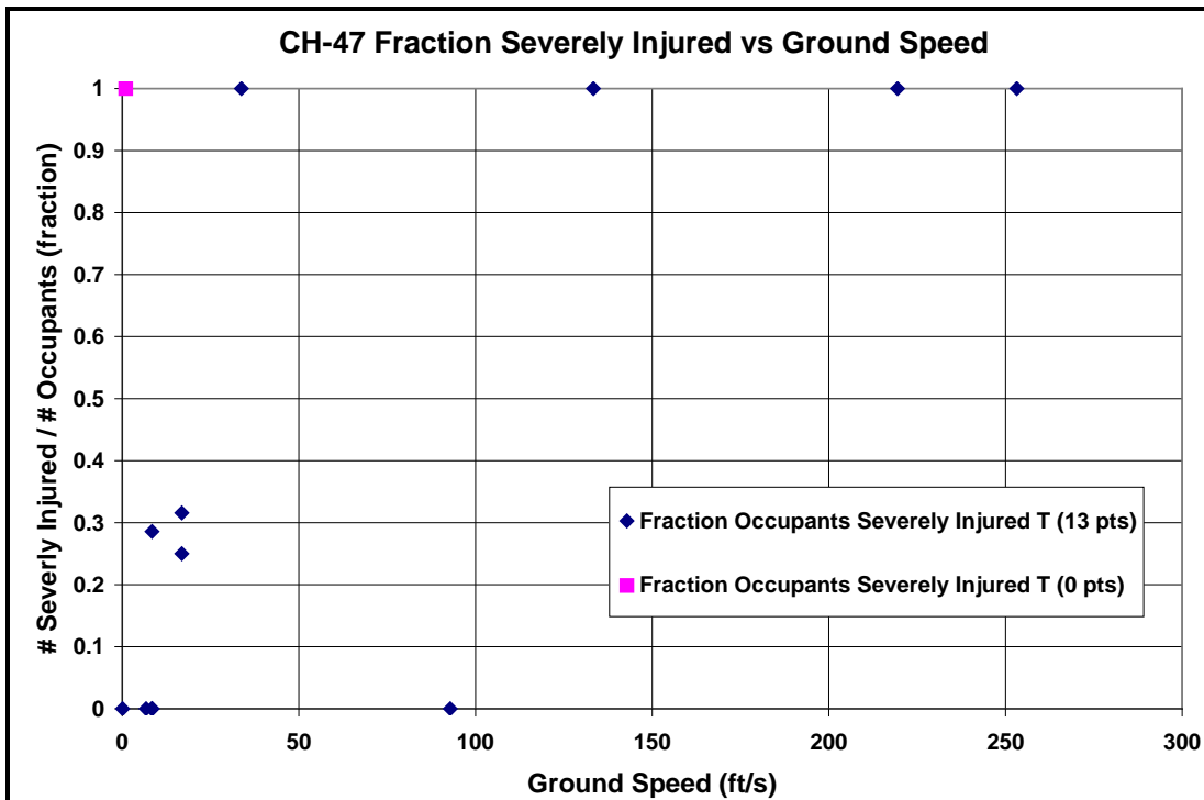
Figure I-6 – CH-47 Fraction Severely Injured vs. Ground Speed
