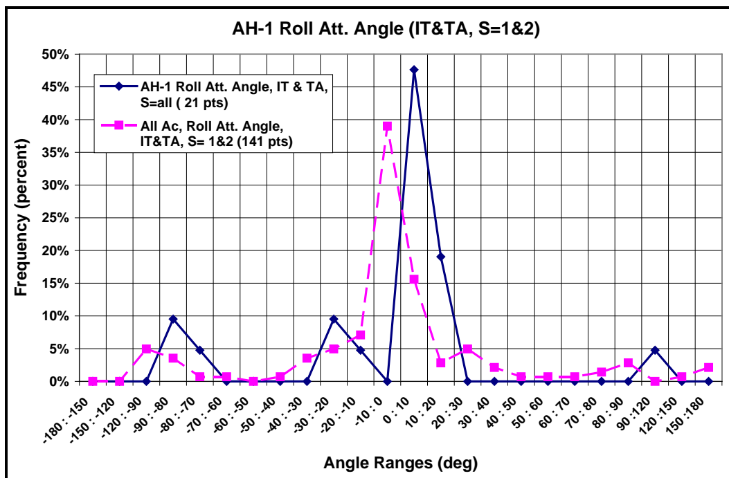
Figure D-6 – AH-1 Roll Attitude Angle (IT&TA, S=1&2)
