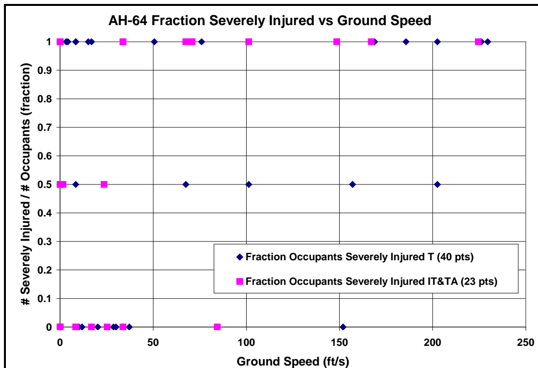
Figure I-4 – AH-64 Fraction Severely Injured vs. Ground Speed
