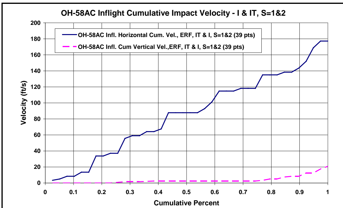
Figure L-6 – Inflight Cumulative Impact Velocity, OH-58AC
