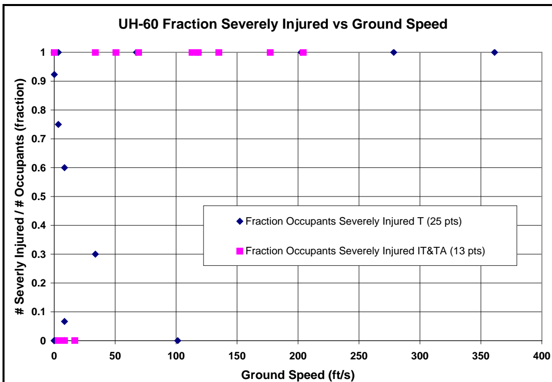
Figure I-16 – UH-60 Fraction Severely Injured vs. Ground Speed
