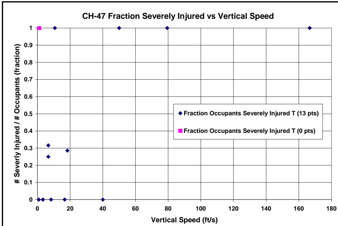
Figure I-5 – CH-47 Fraction Severely Injured vs. Vertical Speed
