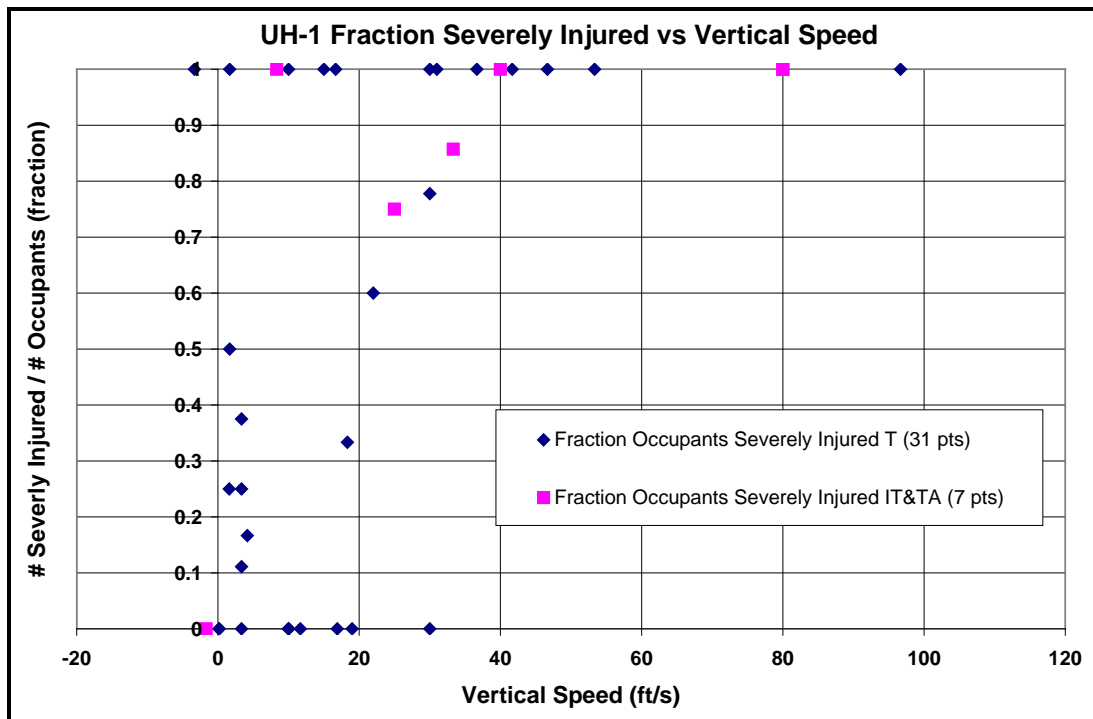
Figure I-13 – UH-1 Fraction Severely Injured vs. Vertical Speed
