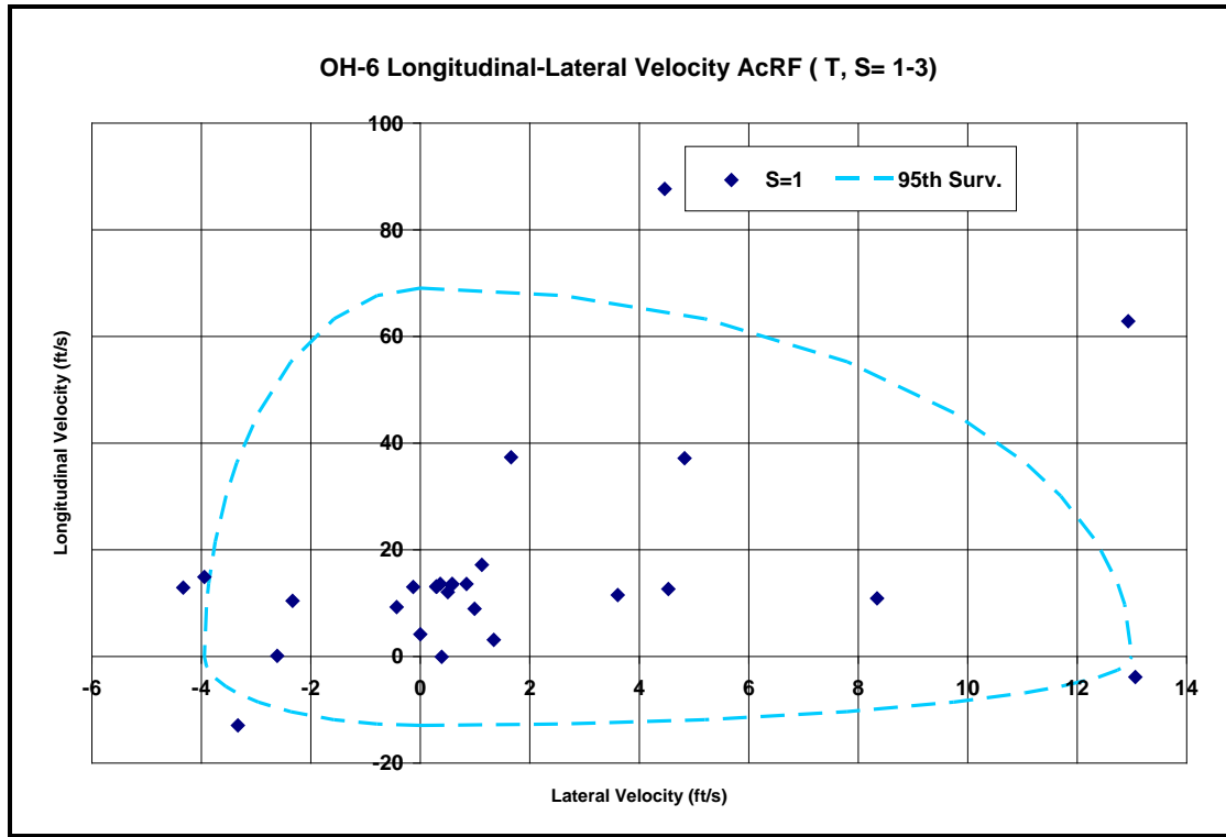
Figure C-21 – OH-6 Longitudinal-Lateral Velocity AcRF (T, S= 1-3)
