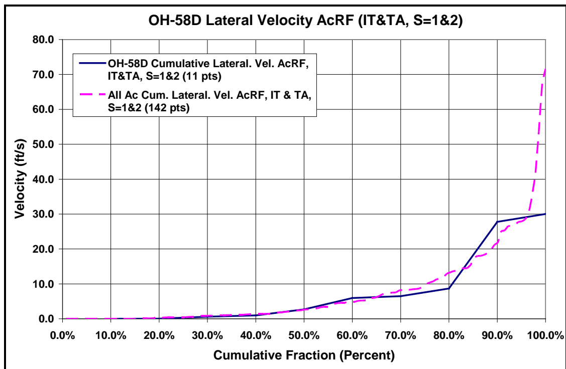
Figure A-60 – OH-58D Lateral Velocity AcRF (IT&TA, S=1&2)
