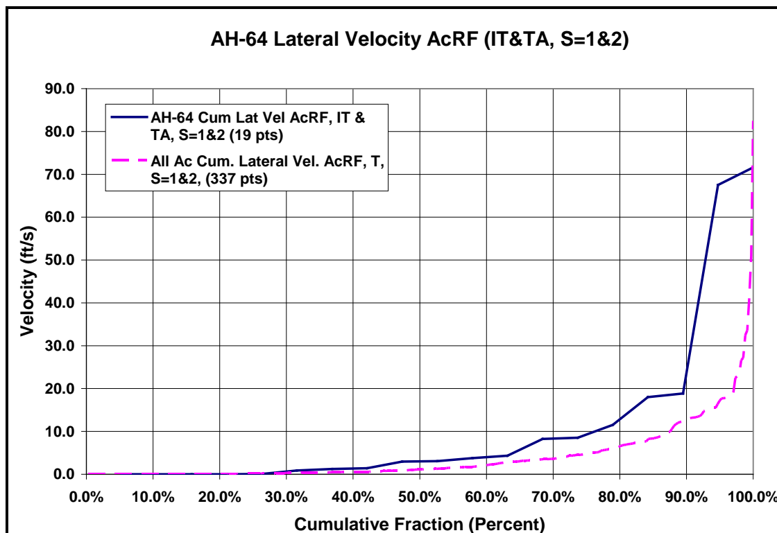
Figure A-20 – AH-64 Lateral Velocity AcRF (IT&TA, S=1&2)
