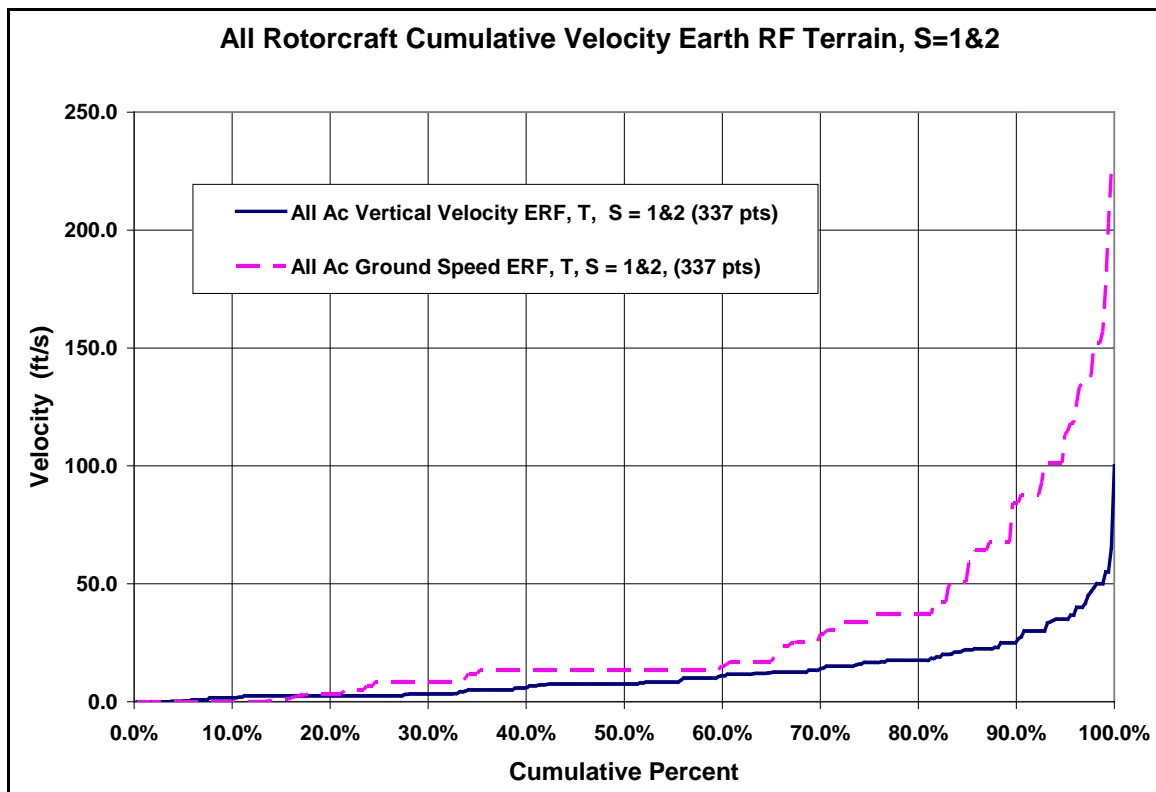
Figure 3 – Cumulative Velocity for T Crashes in ERF
