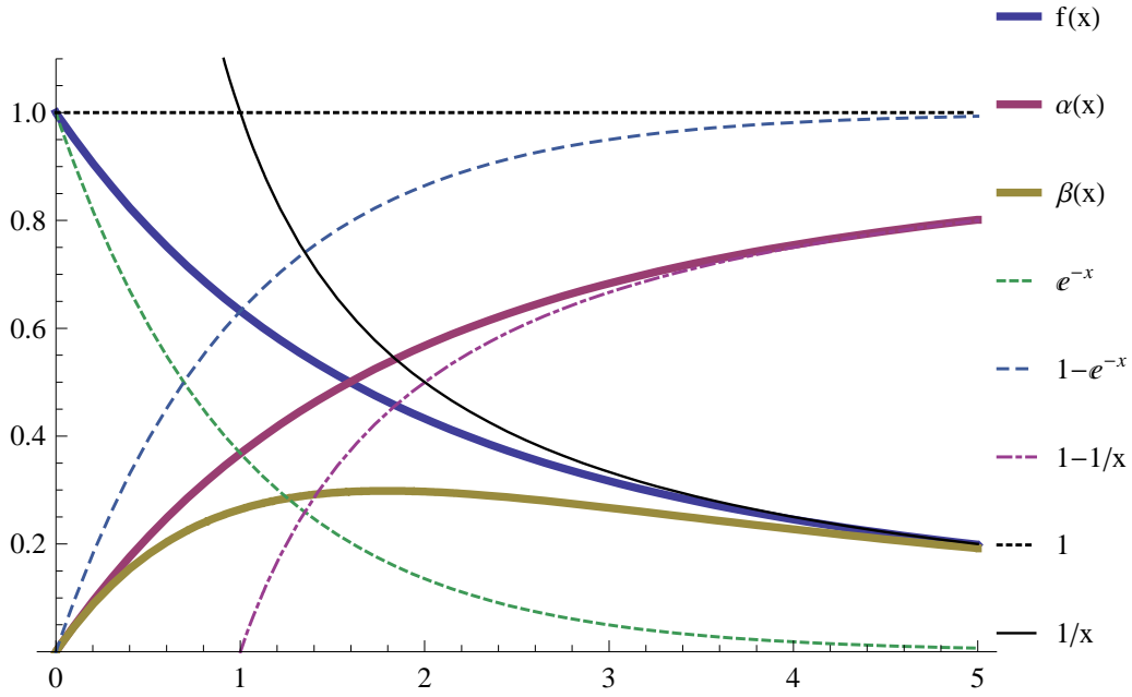
Figure 2. f(x) , \alpha(x) , and \beta(x) for 0 \leq x \leq 5 , with other functions shown for comparison.
