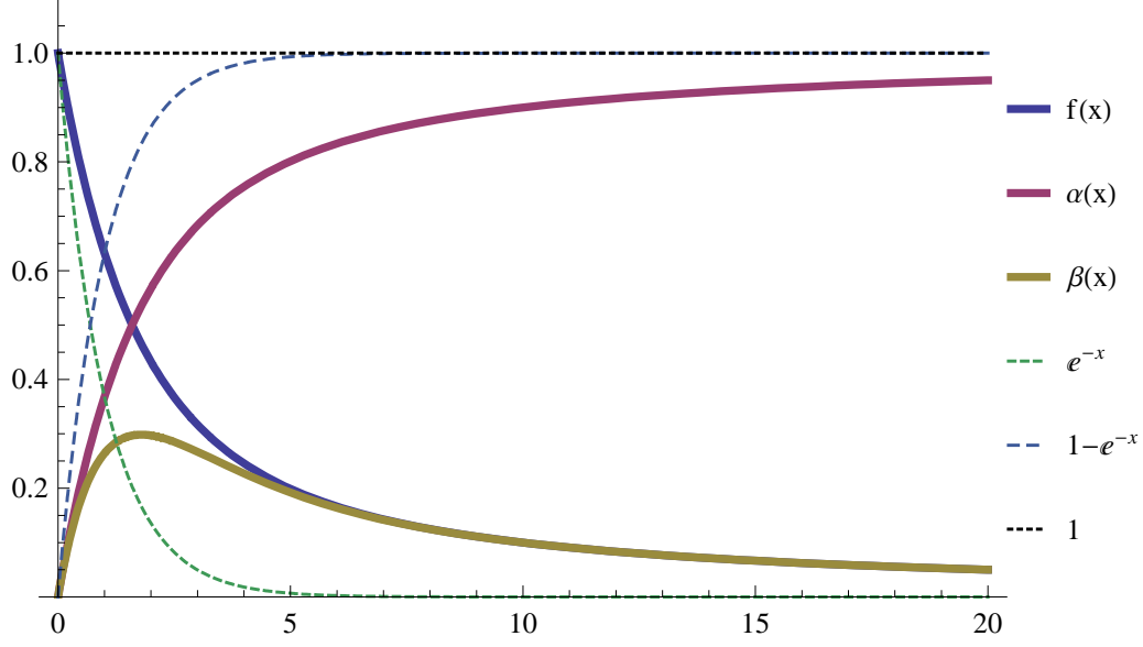
Figure 1. f(x) , \alpha(x) , and \beta(x) for 0 \leq x \leq 20 , with other functions shown for comparison.
