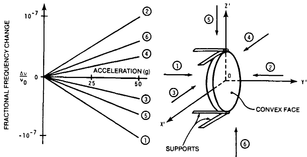
Fig. 9. Typical sensitivity of an AT-cut resonator to acceleration as a function of direction. From [19].
