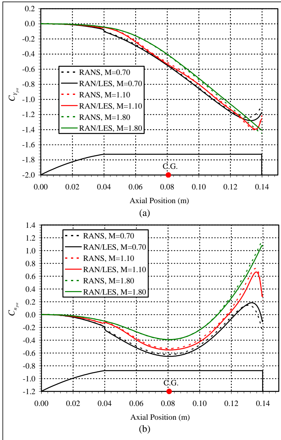
Figure 11. Distribution of Magnus (a) force and (b) moment coefficient (at \alpha = 2^\circ ) on standard-base ANSR: comparison of RANS and RANS/LES computations.
