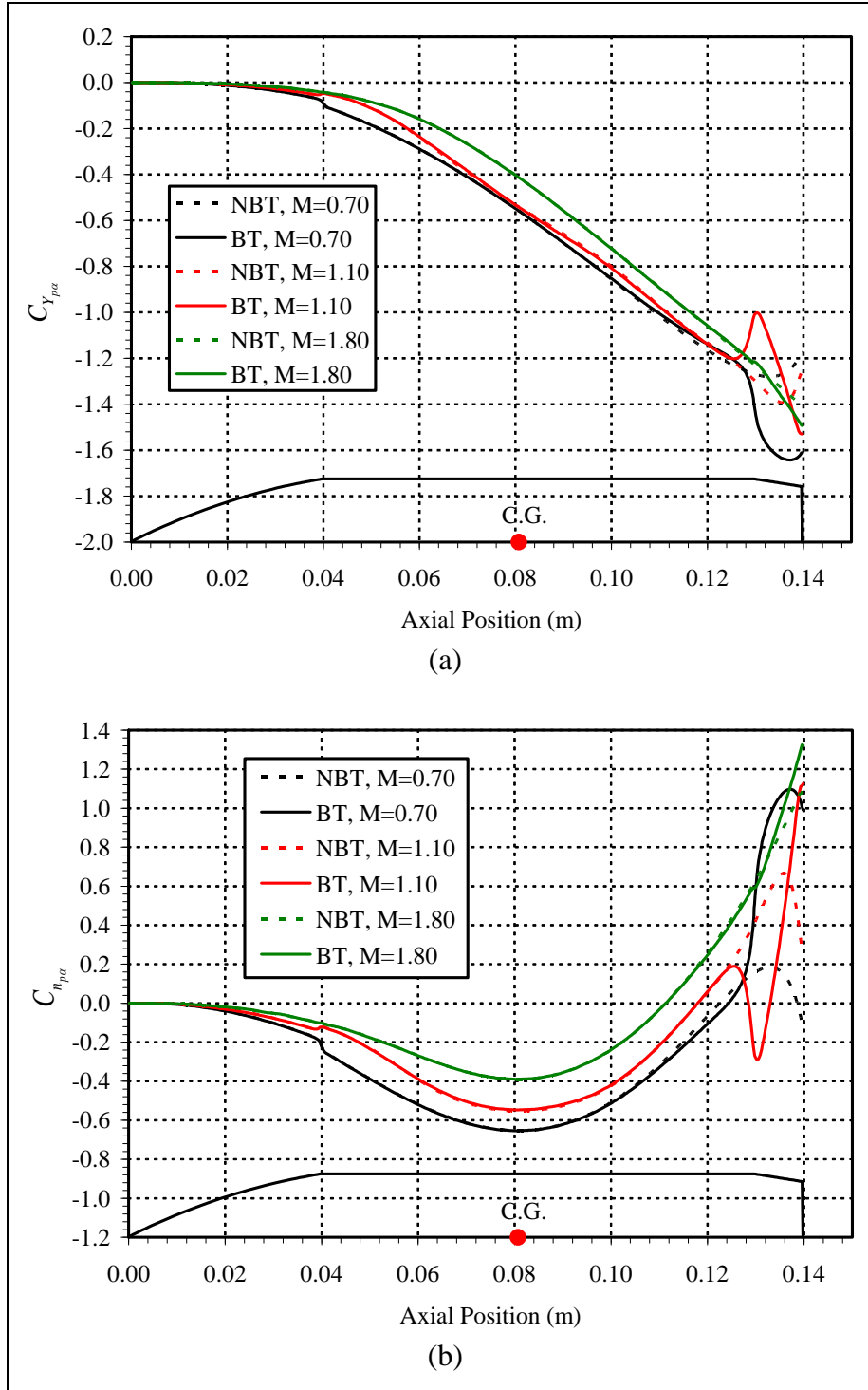
Figure 13. Distribution of Magnus (a) force and (b) moment coefficient (at \alpha = 2^\circ ): comparison of effect of ANSR base shape for steady-state RANS computations.
