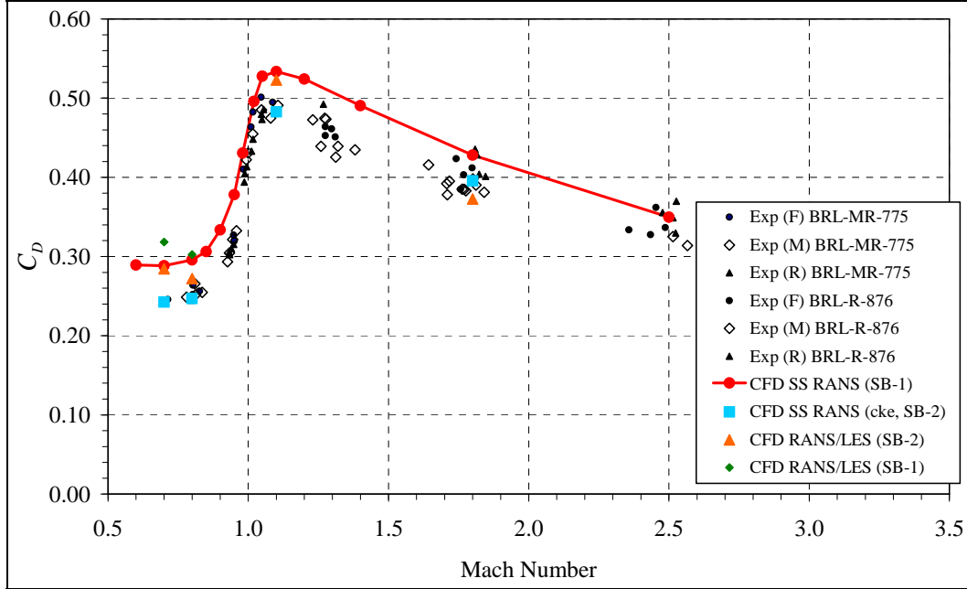
Figure 3. Drag coefficient (at \alpha = 2^\circ ) vs. Mach number: standard-base ANSR.
