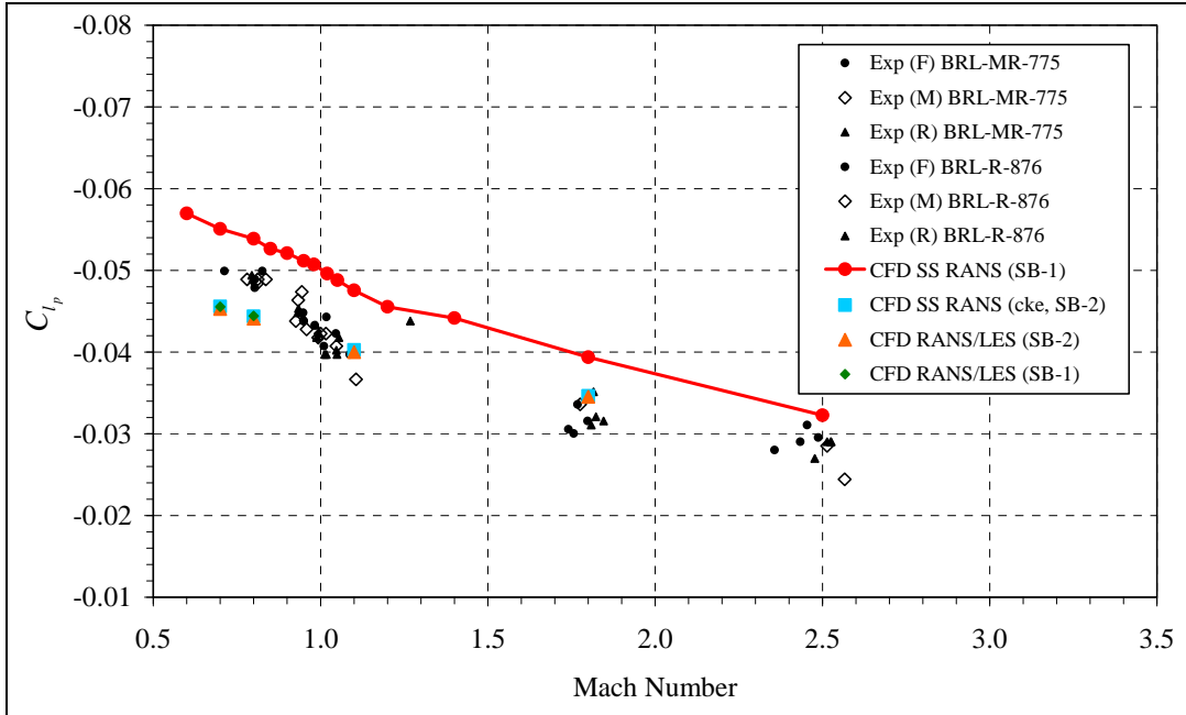
Figure 4. Roll-damping coefficient vs. Mach number: standard-base ANSR.
