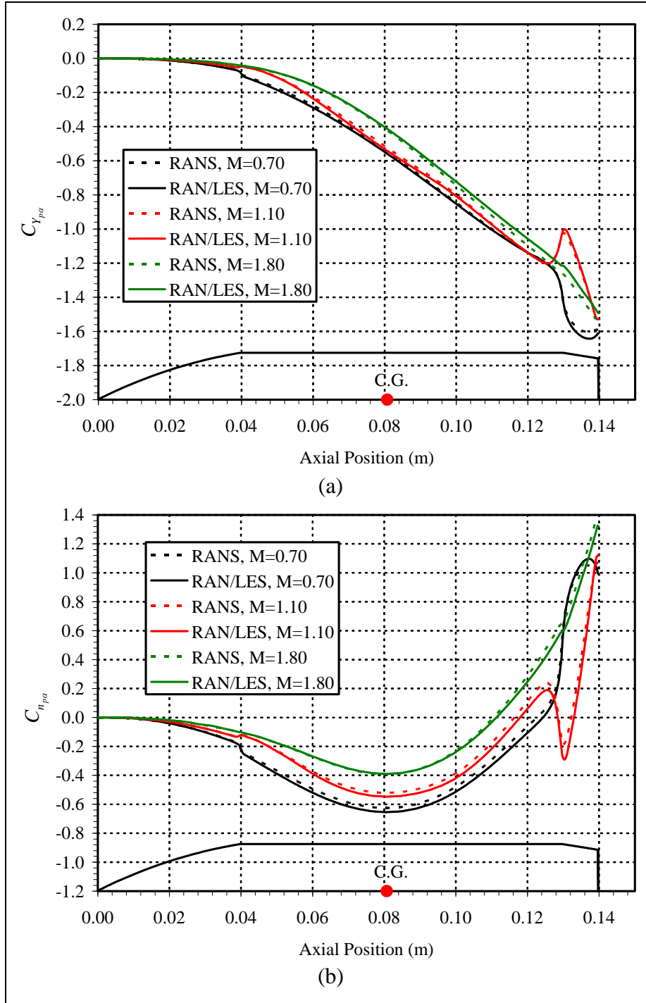
Figure 12. Distribution of Magnus (a) force and (b) moment coefficient (at \alpha = 2^\circ ) on boattail ANSR: comparison of RANS and RANS/LES computations.
