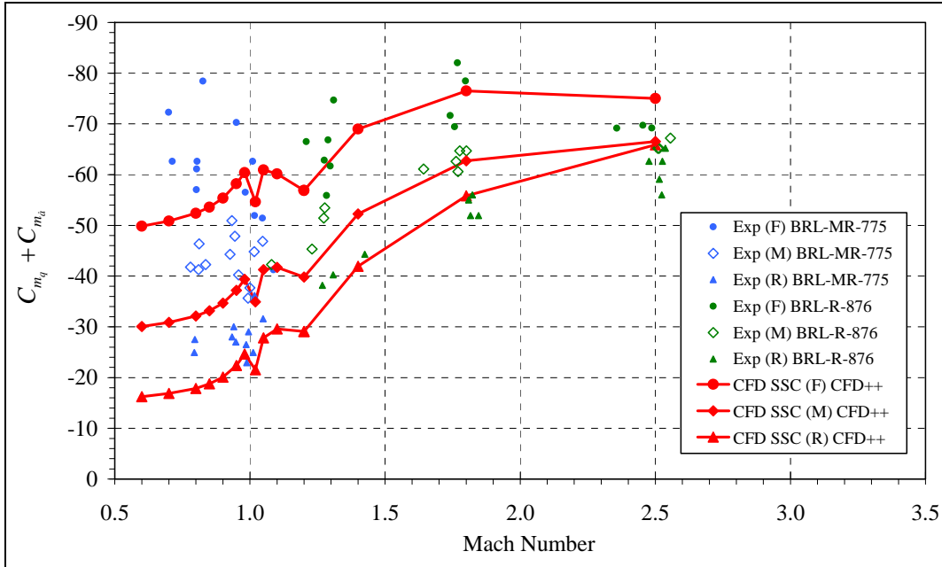
Figure 8. Pitch-damping moment coefficient vs. Mach number: standard-base ANSR.
