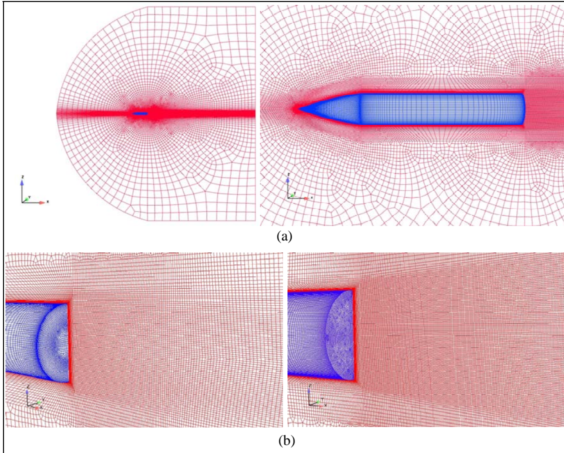
Figure 2. Computational mesh used for standard-base ANSR model: (a) RANS mesh (SB-1) and (b) close-up of the high-density mesh in the wake region of meshes SB-1 (left) and SB-2 (right).
