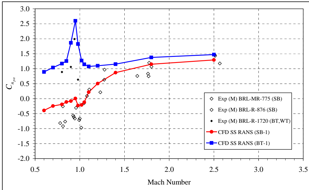
Figure 10. Magnus moment coefficient vs. Mach number: comparison of standard-base and boattail ANSR.
