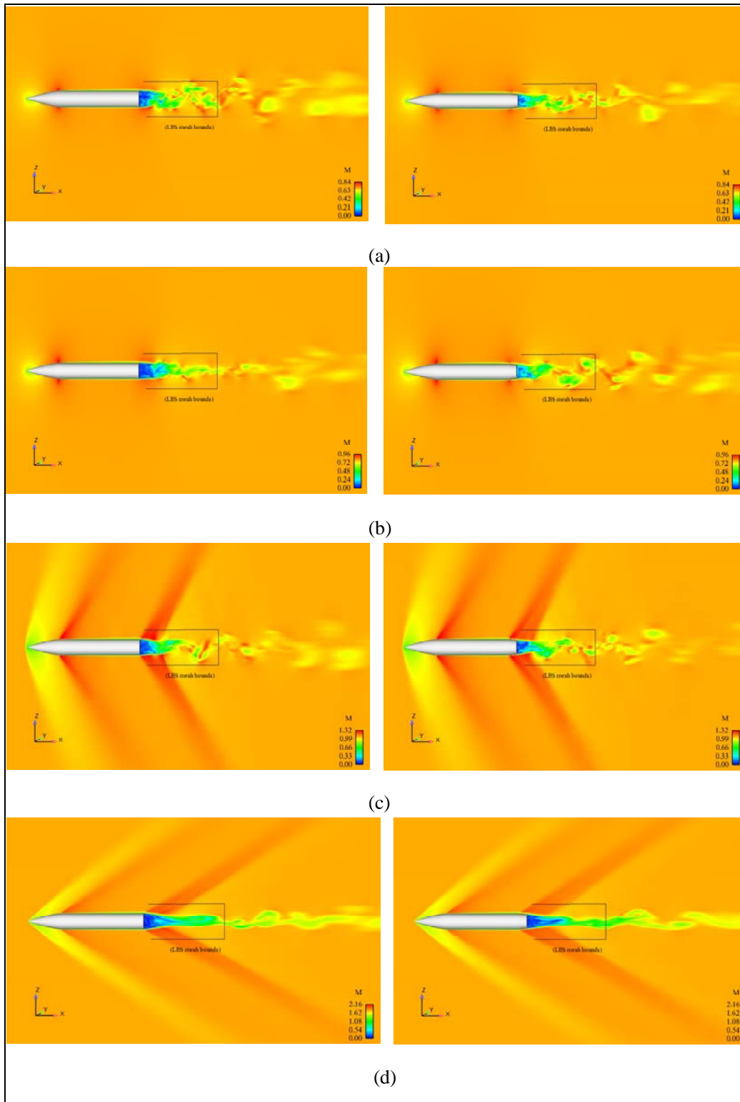
Figure 14. Instantaneous Mach number contours from unsteady RANS/LES calculations: standard-base and boattail ANSR at \alpha = 2^\circ and (a) Mach 0.7; (b) Mach 0.8; (c) Mach 1.1; and (d) Mach 1.8.
