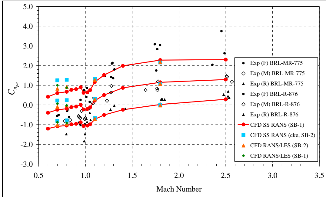
Figure 9. Magnus moment coefficient (at \alpha = 2^\circ ) vs. Mach number: standard-base ANSR.
