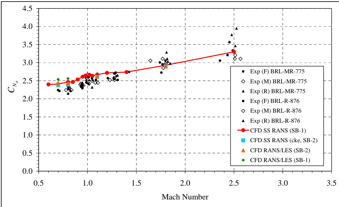
Figure 5. Normal force coefficient vs. Mach number: standard-base ANSR.
