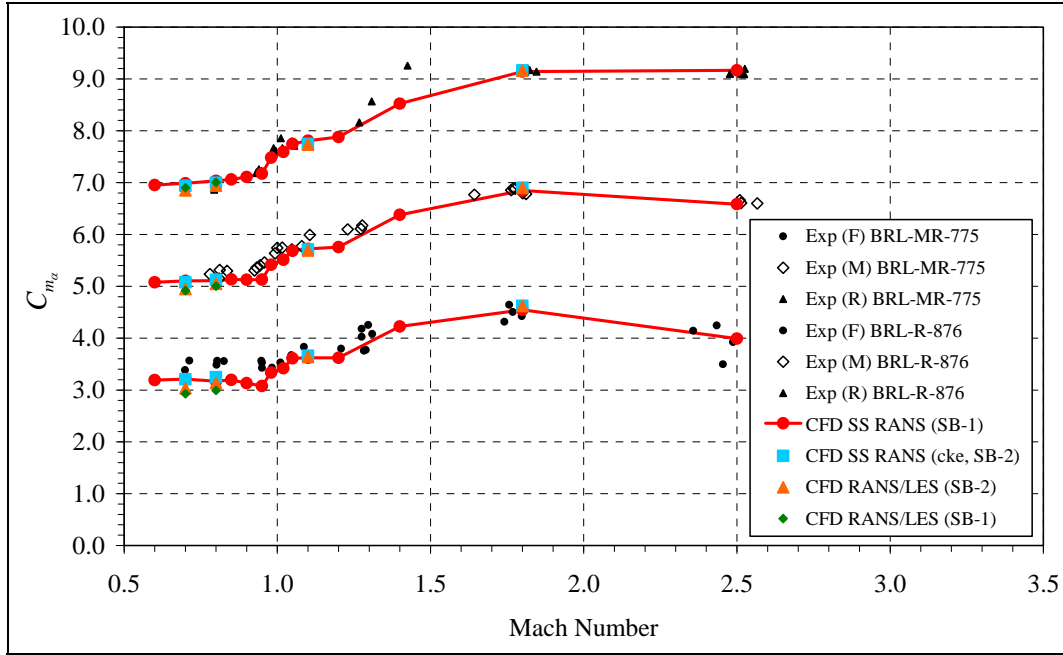
Figure 6. Pitching moment coefficient vs. Mach number: standard-base ANSR.
