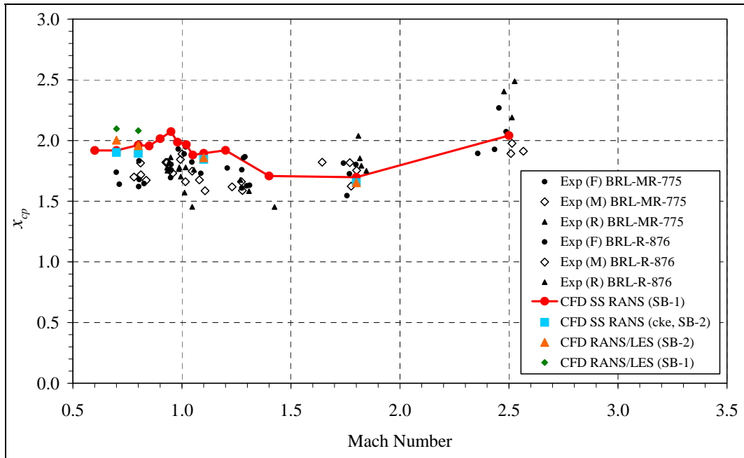
Figure 7. Normal force center-of-pressure location vs. Mach number: standard-base ANSR.
