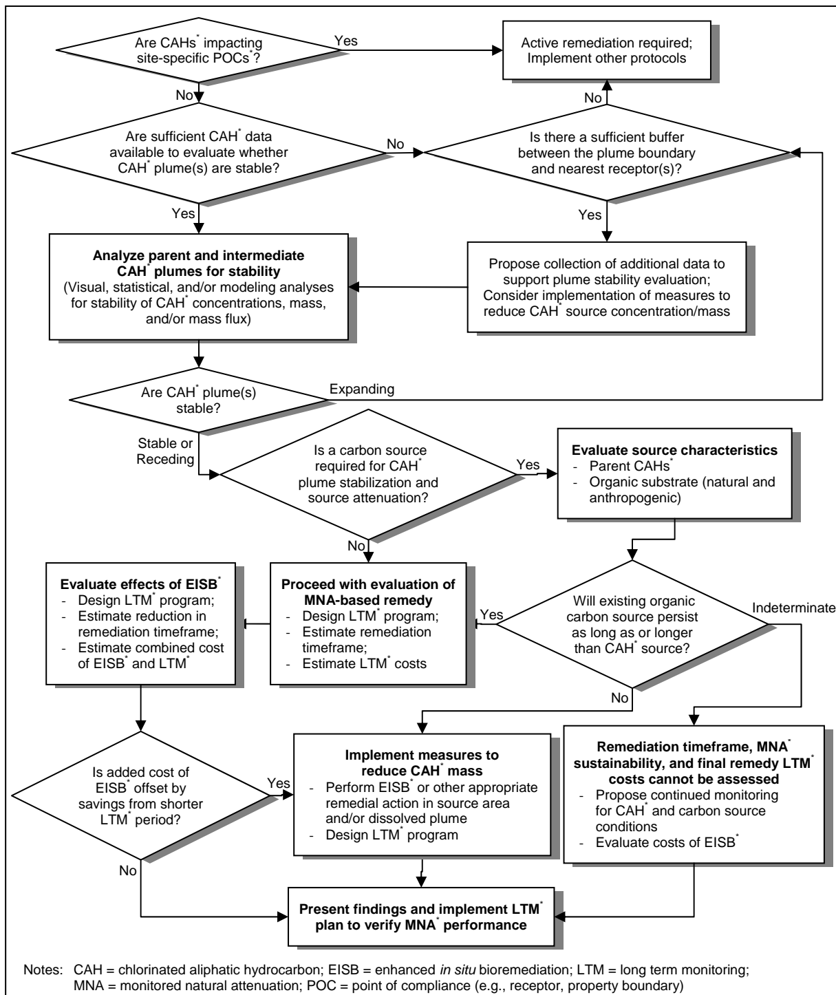
FIGURE 2.1 CONCEPTUAL FRAMEWORK FOR ASSESSING APPROPRIATENESS OF MNA- BASED REMEDIES AT CAH-IMPACTED SITES. FIELD-SCALE EVALUATION OF MNA FOR DISSOLVED CHLORINATED SOLVENT PLUMES
