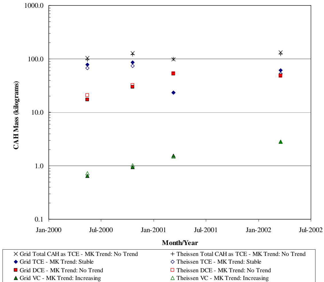
FIGURE 4.15 ESTIMATED DISSOLVED MASS OF CAH COMPOUNDS SITE SS-45 NORTHWEST PLUME, ENGLAND AFB, LOUISIANA FIELD-SCALE EVALUATION OF MNA FOR DISSOLVED CHLORINATED SOLVENT PLUMES
