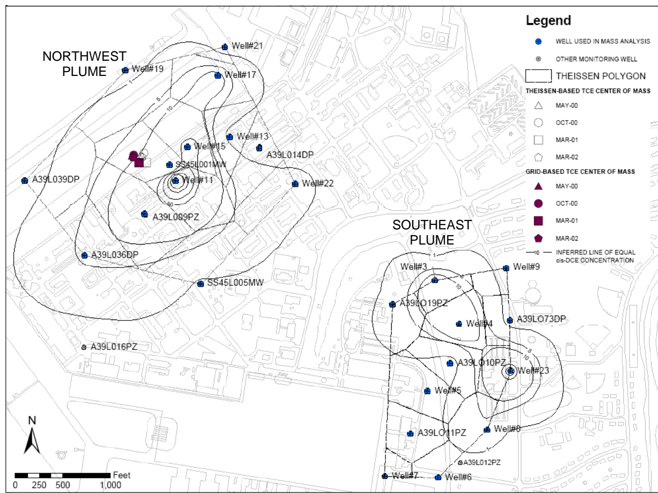
FIGURE 4.16 LOCATION OF CENTERS OF MASS FOR TCE SITE SS-45, ENGLAND AFB, LOUISIANA FIELD-SCALE EVALUATION OF MNA FOR DISSOLVED CHLORINATED SOLVENT PLUMES
