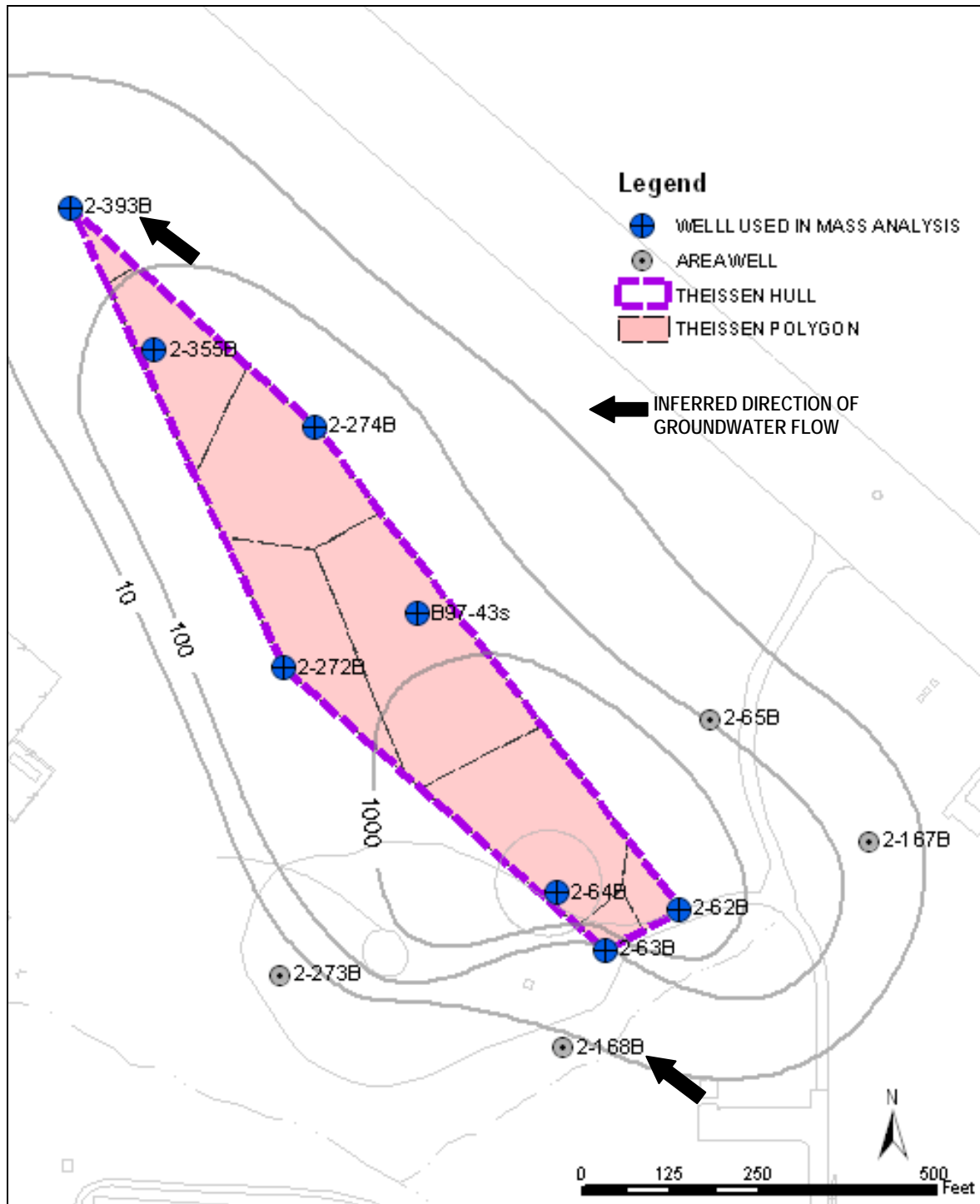
FIGURE 4.4 MODEL DOMAIN AND COMMON WELLS FOR MASS-BASED CALCULATIONS SITE FTA-2, TINKER AFB, OKLAHOMA FIELD-SCALE EVALUATION OF MNA FOR DISSOLVED CHLORINATED SOLVENT PLUMES
