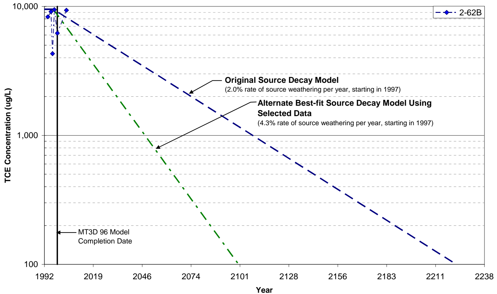
FIGURE 4.39 MEASURED AND PREDICTED TCE CONCENTRATIONS OVER TIME SITE FTA-2, TINKER AFB, OKLAHOMA FIELD-SCALE EVALUATION OF MNA FOR DISSOLVED CHLORINATED SOLVENT PLUMES
