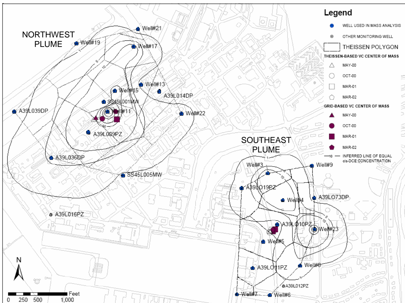
FIGURE 4.18 LOCATION OF CENTERS OF MASS FOR VC SITE SS-45, ENGLAND AFB, LOUISIANA FIELD-SCALE EVALUATION OF MNA FOR DISSOLVED CHLORINATED SOLVENT PLUMES
