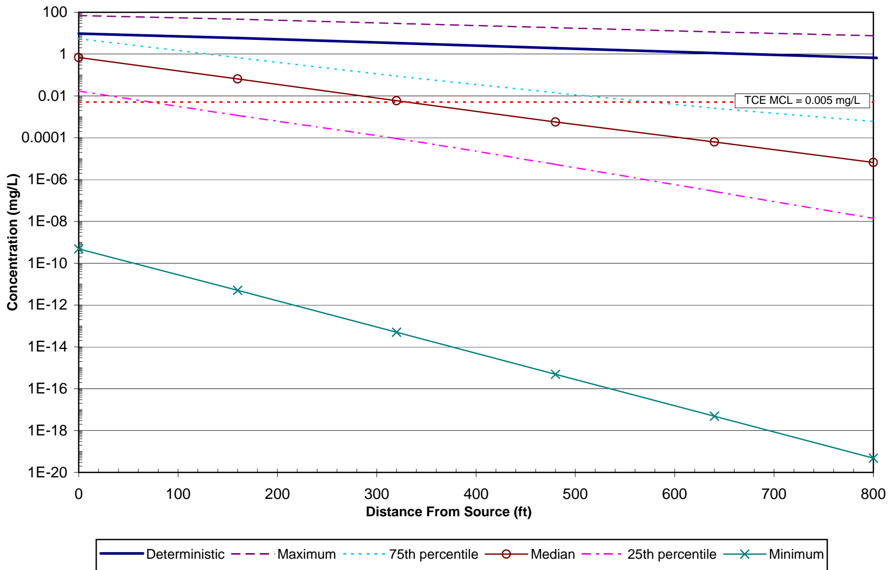
Figure 21: TCE Deterministic and Stochastic Modeled Concentrations in 1997 - Tinker AFB
