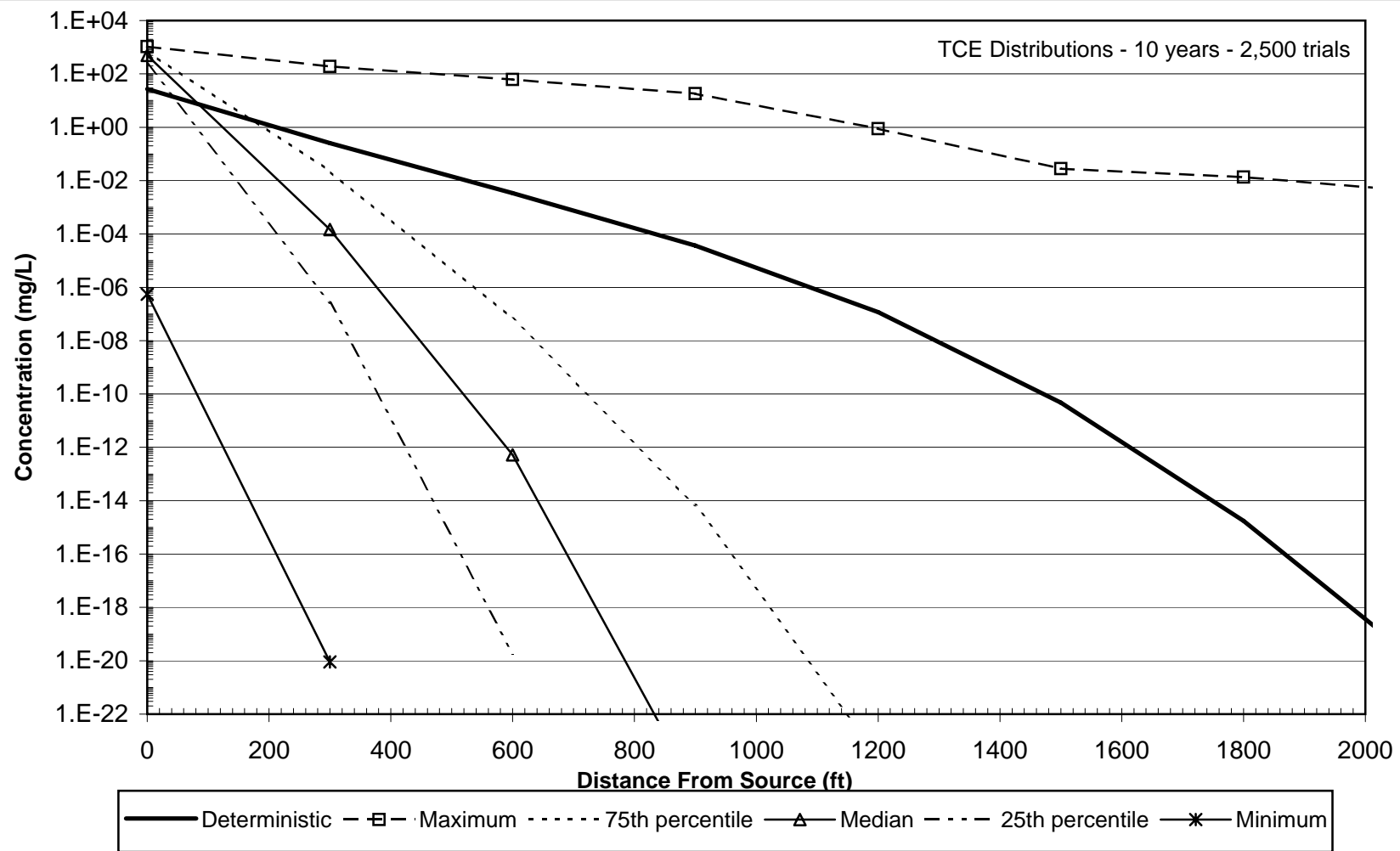
Figure 6b: Deterministic and Stochastic TCE Concentrations with Biodegradation Synthetic Case Study
