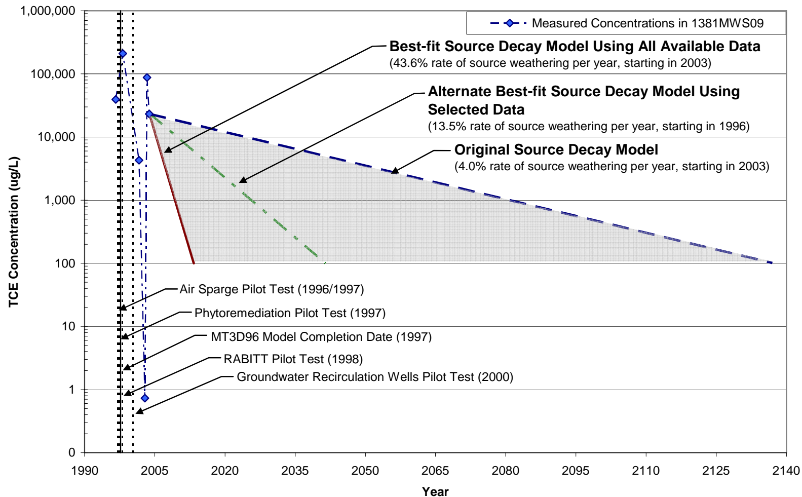
FIGURE 4.38 MEASURED AND PREDICTED TCE CONCENTRATIONS OVER TIME Facility 1381, Cape Canaveral AFS, Florida FIELD-SCALE EVALUATION OF MNA FOR DISSOLVED CHLORINATED SOLVENT PLUMES
