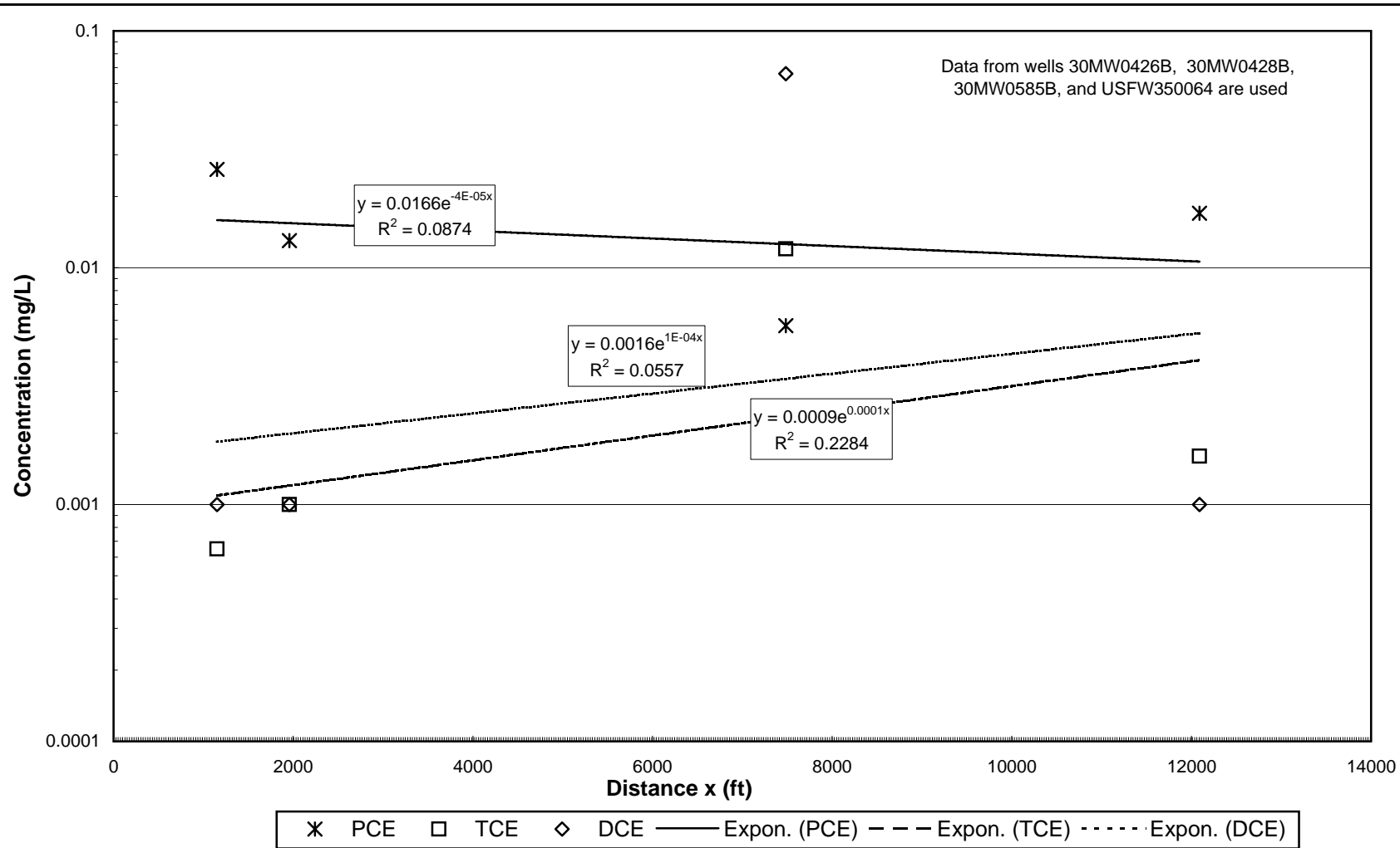
Figure 28b: 1999 Plume Centerline Concentrations - Ashumet, MMR
