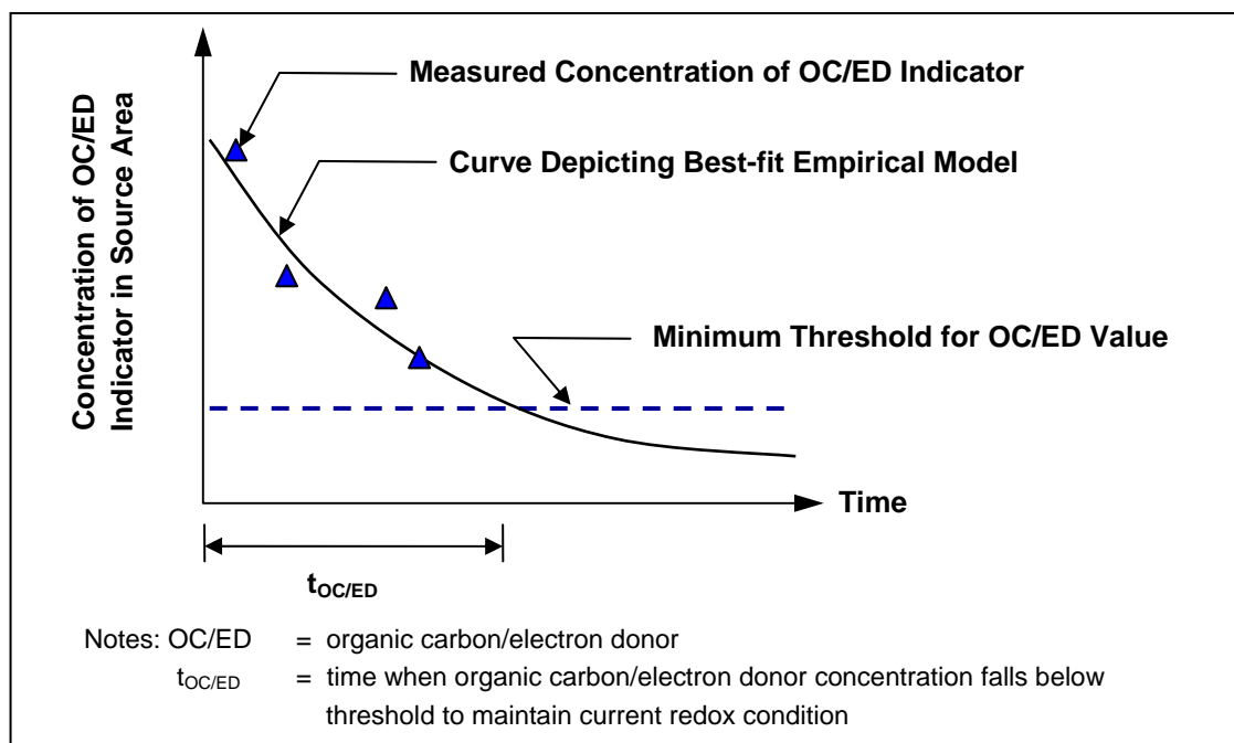
FIGURE 2.2 SCHEMATIC REPRESENTATION OF A METHOD FOR ESTIMATING DURATION OF ORGANIC CARBON/ELECTRON DONOR CONTROL OF LOCAL REDOX CONDITIONS FIELD-SCALE EVALUATION OF MNA FOR DISSOLVED CHLORINATED SOLVENT PLUMES
