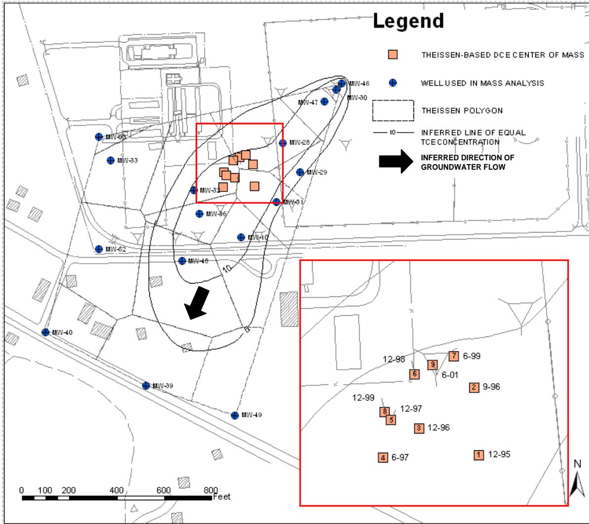
FIGURE 4.35 LOCATION OF CENTERS OF MASS FOR CIS-1,2-DCE FPTA-2, BROOKS CITY-BASE, TEXAS FIELD-SCALE EVALUATION OF MNA FOR DISSOLVED CHLORINATED SOLVENT PLUMES
