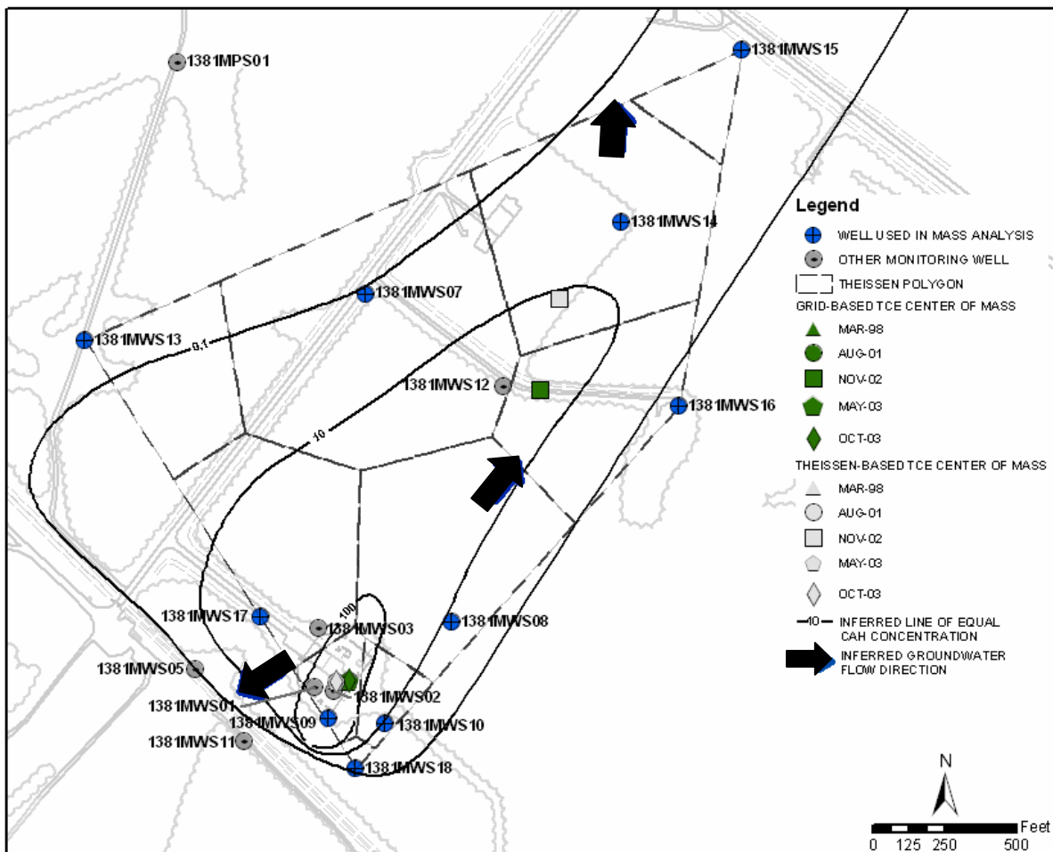
FIGURE 4.26 LOCATION OF CENTERS OF MASS FOR TCE FACILITY 1381, CAPE CANAVERAL AFS, FLORIDA FIELD-SCALE EVALUATION OF MNA FOR DISSOLVED CHLORINATED SOLVENT PLUMES
