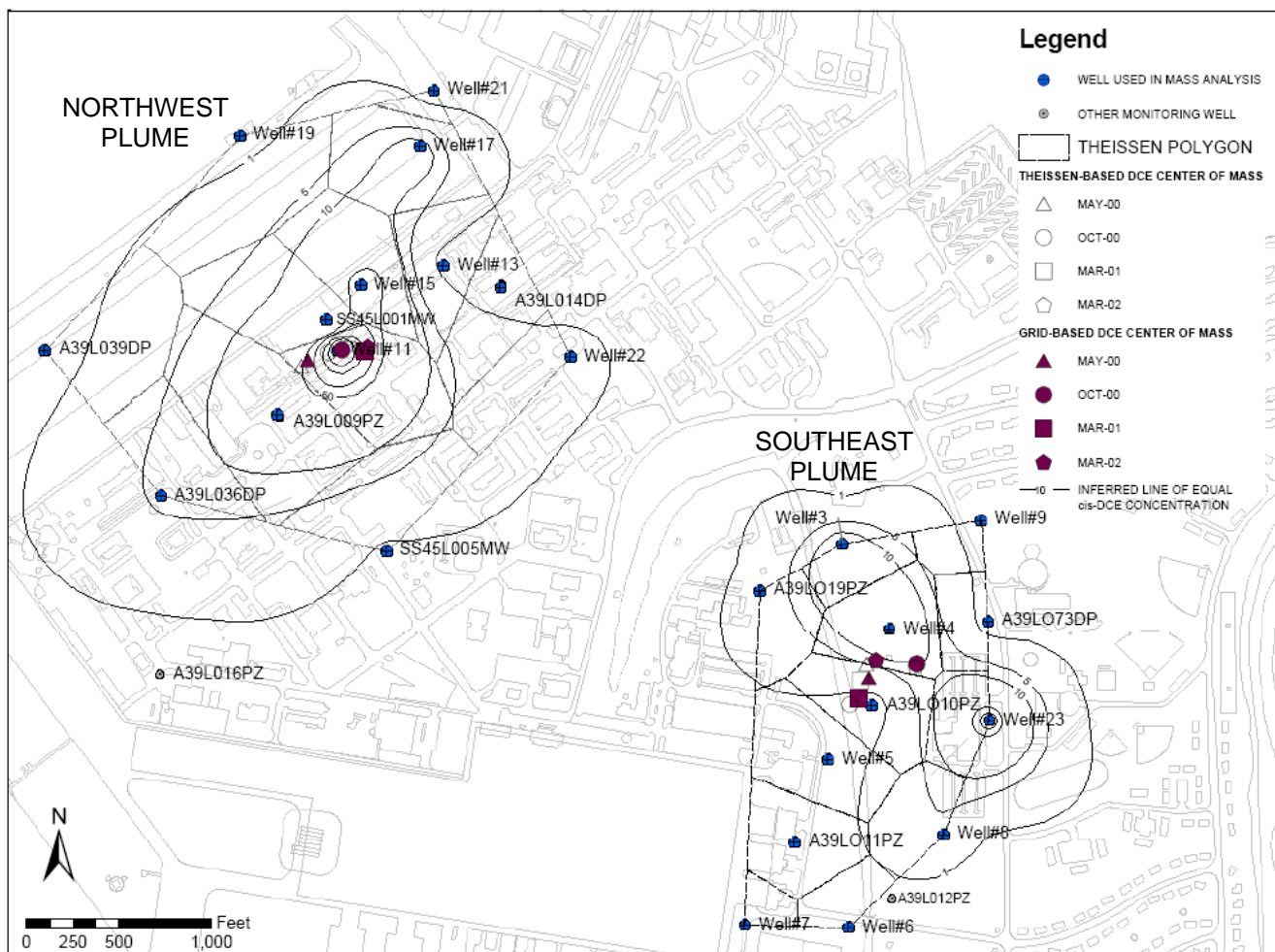
FIGURE 4.17 LOCATION OF CENTERS OF MASS FOR CIS-1,2-DCE SITE SS-45, ENGLAND AFB, LOUISIANA FIELD-SCALE EVALUATION OF MNA FOR DISSOLVED CHLORINATED SOLVENT PLUMES
