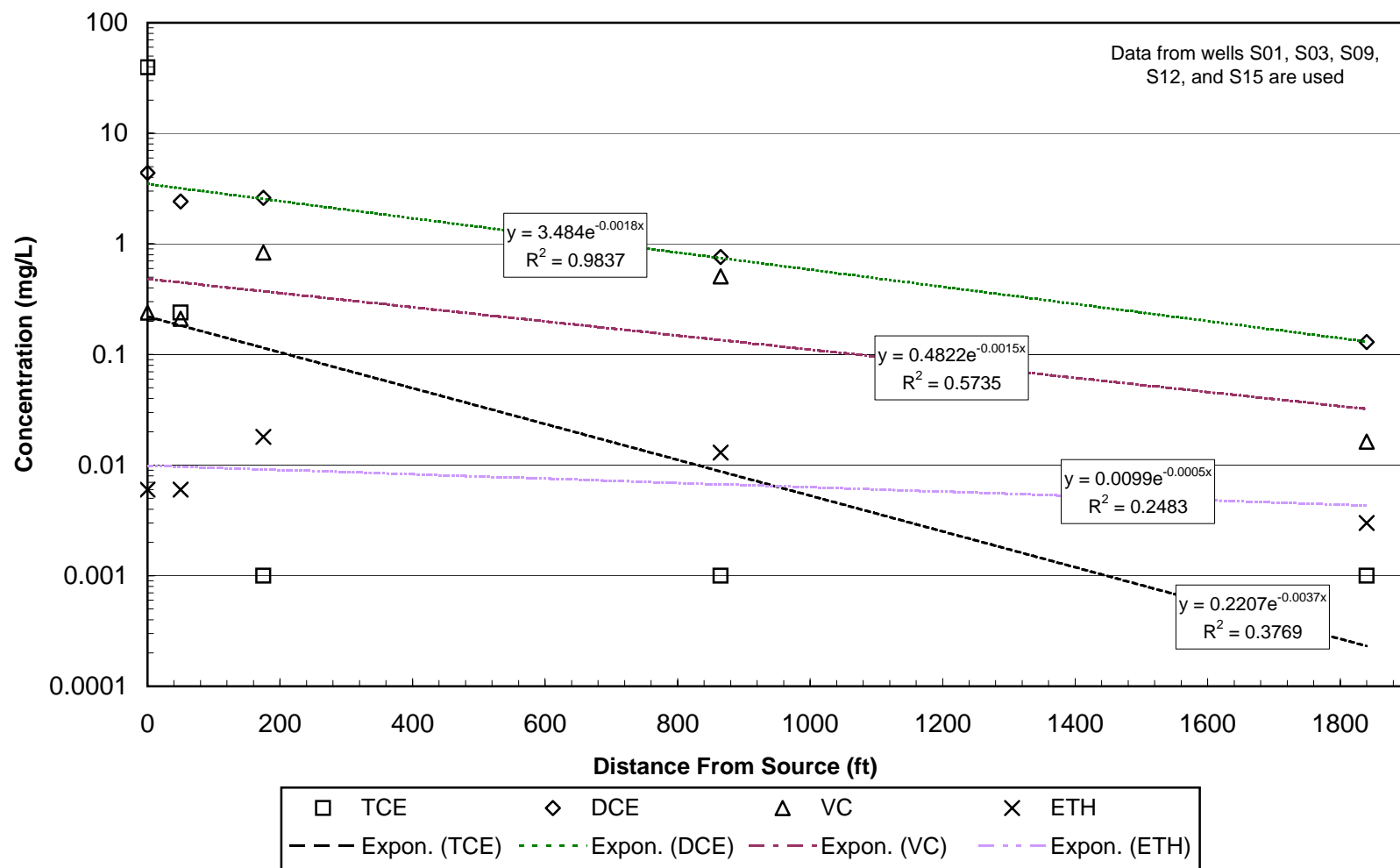
Figure 9a: 1996 Plume Centerline Concentrations - CCAS
