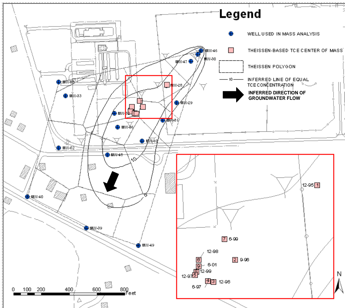
FIGURE 4.34 LOCATION OF CENTERS OF MASS FOR TCE FPTA-2, BROOKS CITY-BASE, TEXAS FIELD-SCALE EVALUATION OF MNA FOR DISSOLVED CHLORINATED SOLVENT PLUMES
