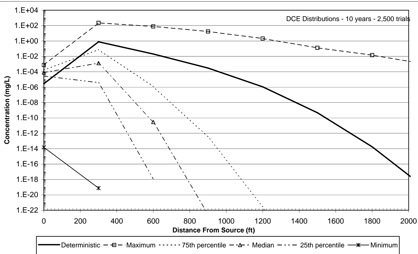
Figure 6c: Deterministic and Stochastic DCE Concentrations with Biodegradation Synthetic Case Study
