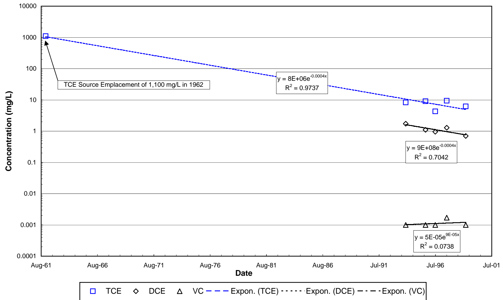
Figure 20: Source Decay Rates in well 2-62B - Tinker AFB
