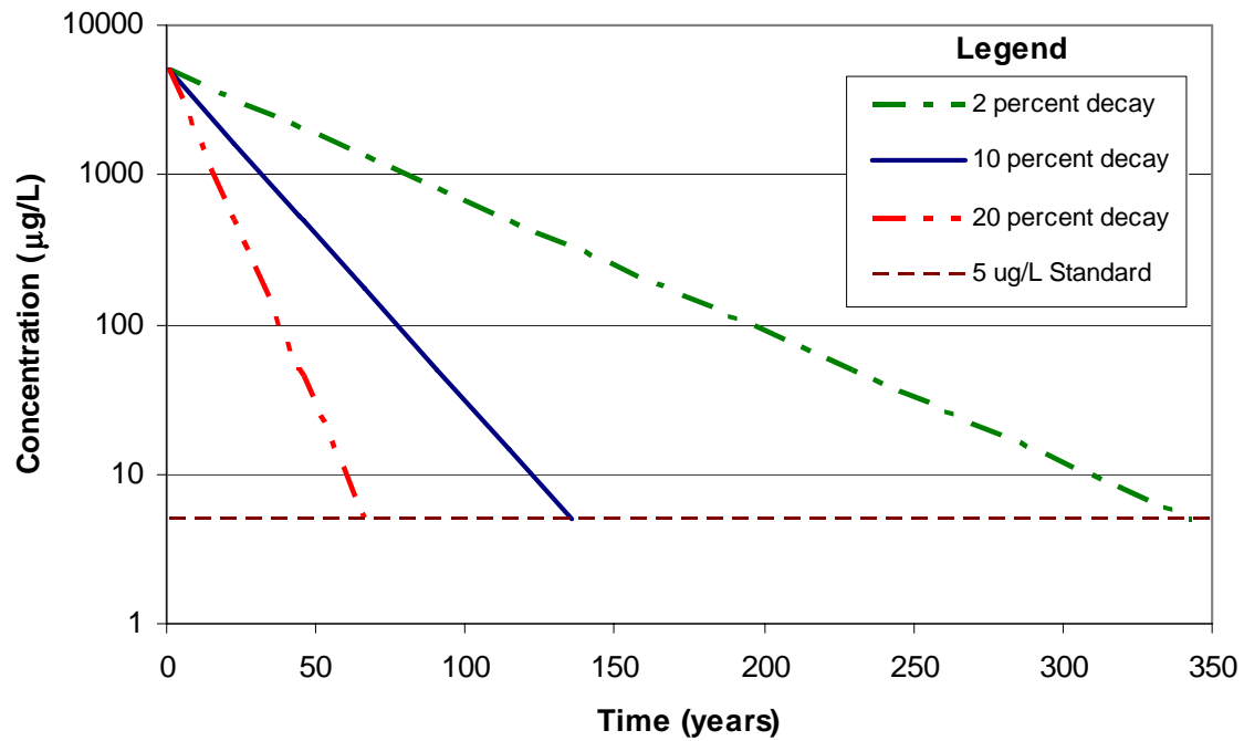
FIGURE 4.40 TEMPORAL CHANGES IN CAH CONCENTRATION FOR VARYING FIRST-ORDER WEATHERING RATES FIELD-SCALE EVALUATION OF MNA FOR DISSOLVED CHLORINATED SOLVENT PLUMES
