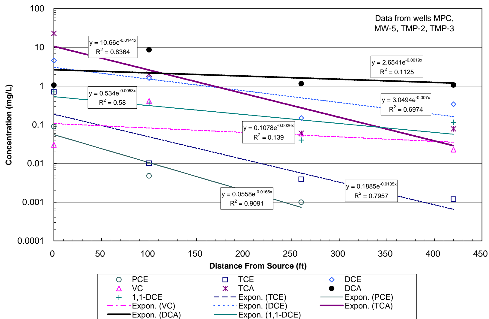
Figure 14: 1997 Centerline Concentrations - Shaw AFB
