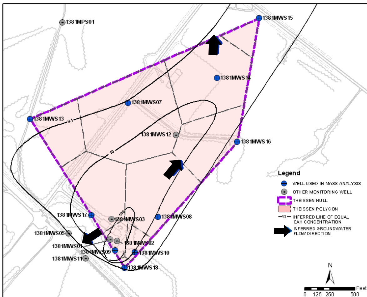
FIGURE 4.24 MODEL DOMAIN AND COMMON WELLS FOR MASS-BASED CALCULATIONS FACILITY 1381, CAPE CANAVERAL AFS, FLORIDA FIELD-SCALE EVALUATION OF MNA FOR DISSOLVED CHLORINATED SOLVENT PLUMES
