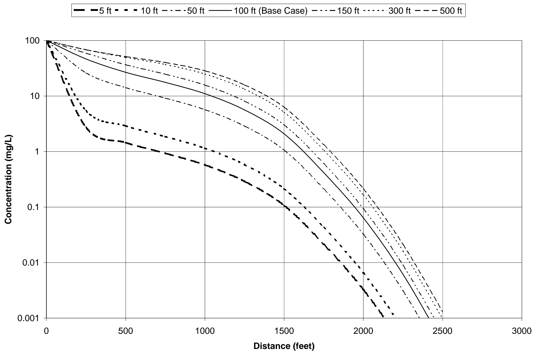
Figure 3a: Source Width Effects
