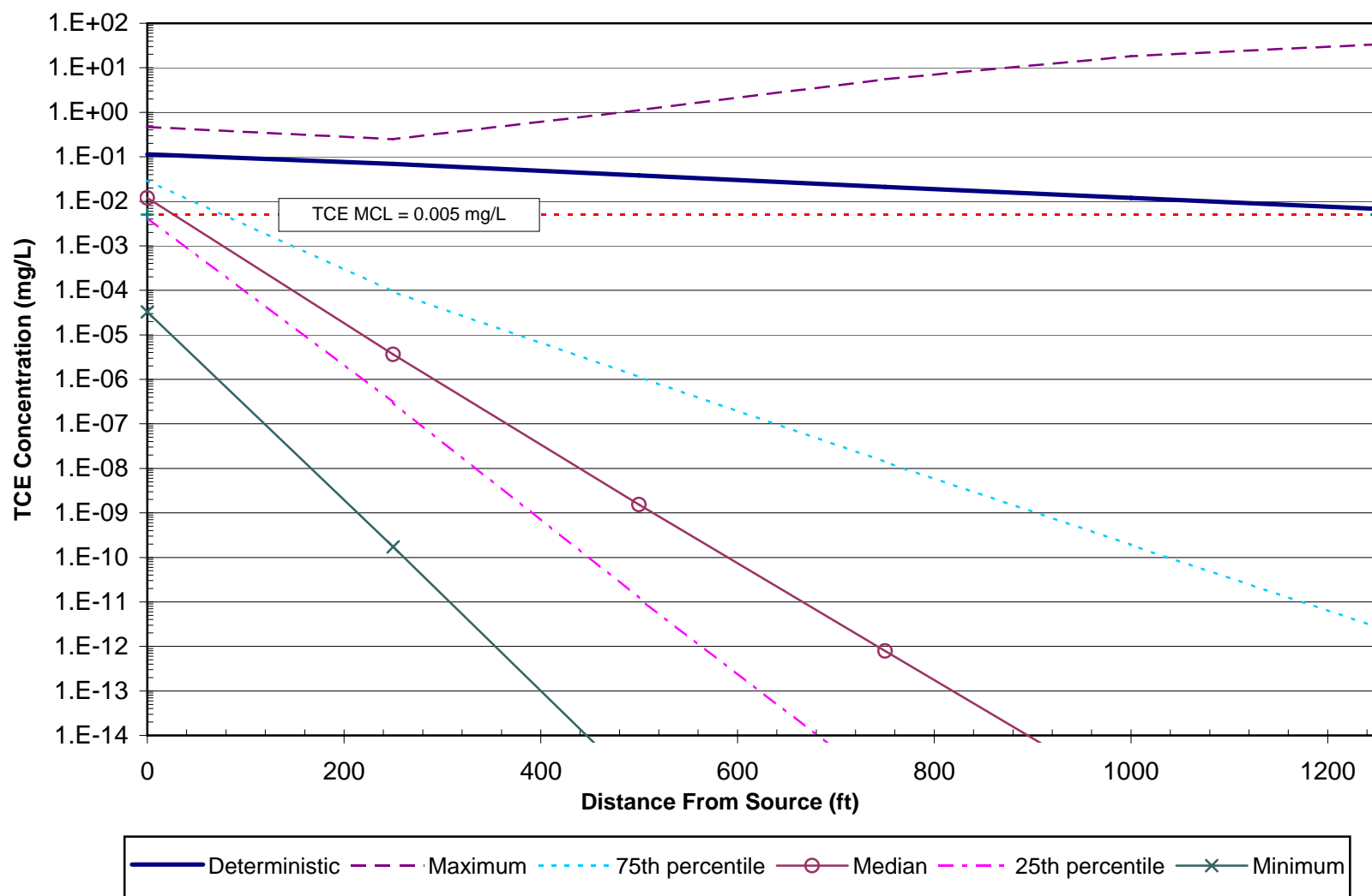
Figure 25a: TCE Deterministic and Stochastic Modeled Concentrations in 1993 - Warren AFB
