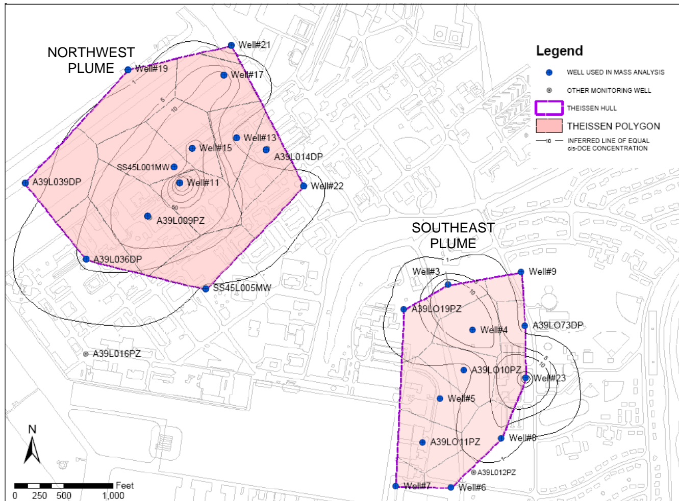
FIGURE 4.14 MODEL DOMAIN AND COMMON WELLS FOR MASS-BASED CALCULATIONS SITE SS-45, ENGLAND AFB, LOUISIANA FIELD-SCALE EVALUATION OF MNA FOR DISSOLVED CHLORINATED SOLVENT PLUMES
