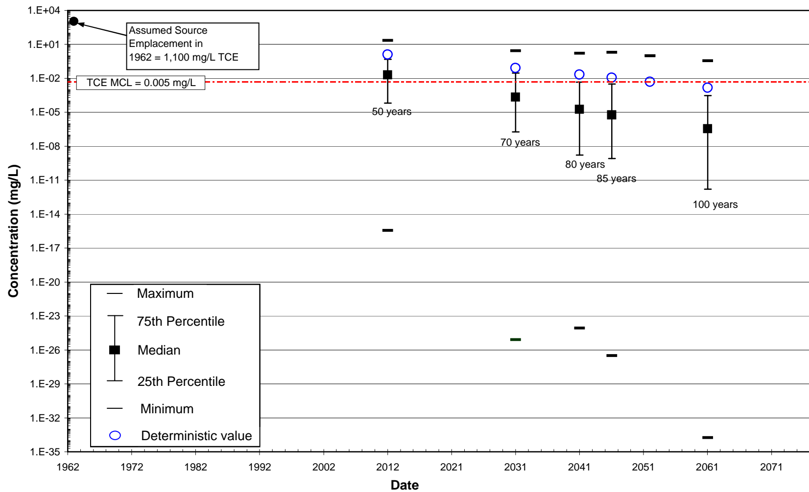
Figure 23: BIOCHLOR Deterministic and Stochastic Model TCE Predictions at the Source Over Time - Tinker AFB
