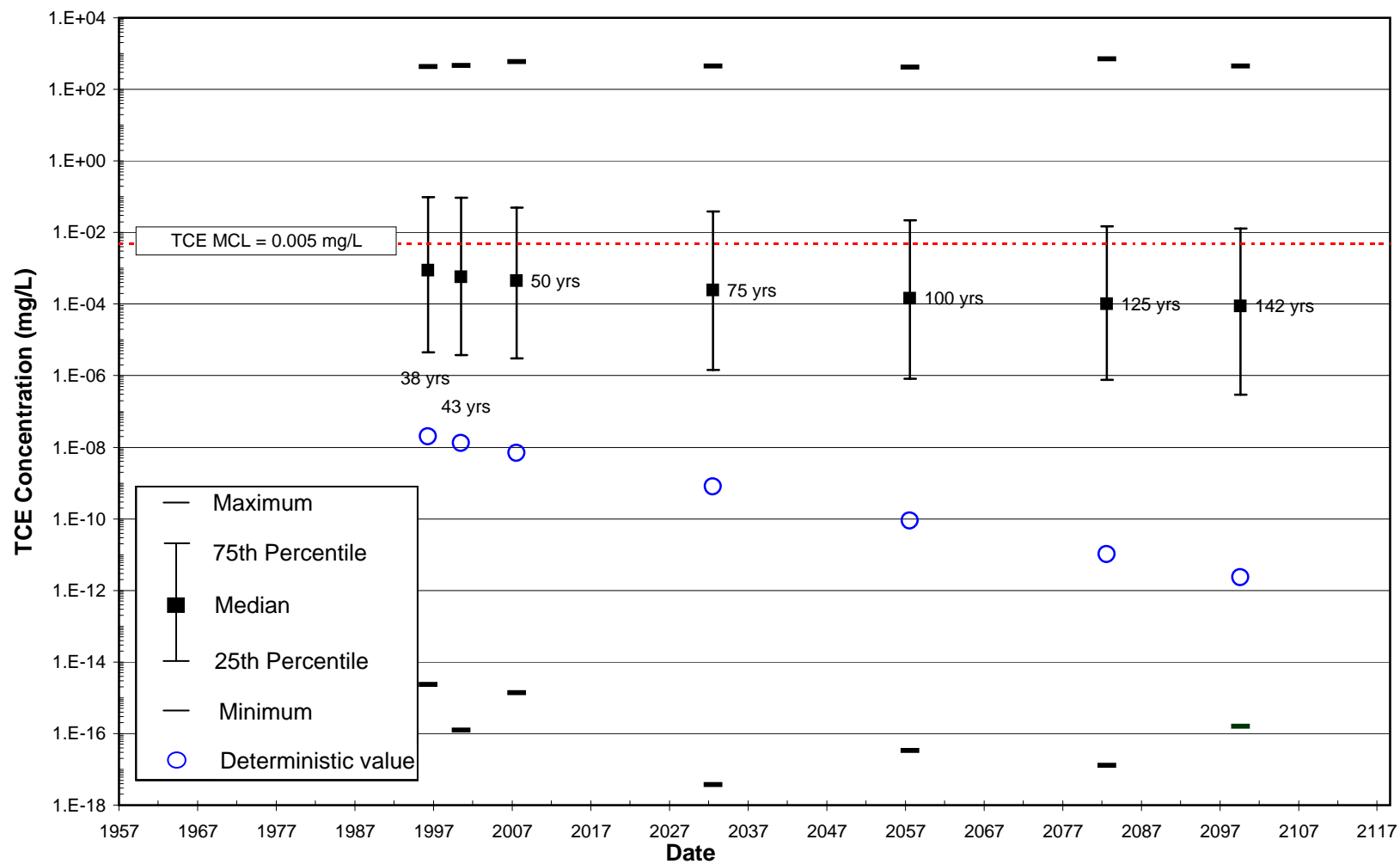
Figure 13b: BIOCHLOR Deterministic and Stochastic Model TCE Predictions at 300 ft Downgradient of the Source Over Time - CCAS
