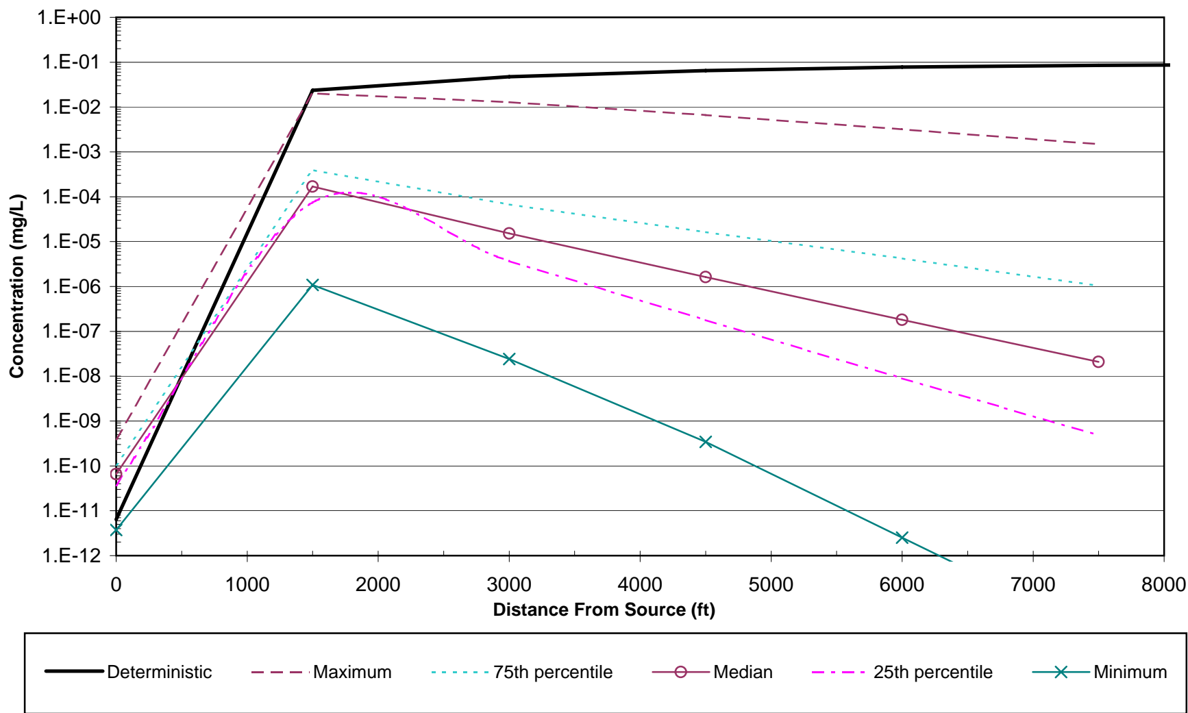
Figure 29c: DCE Deterministic and Stochastic Modeled Concentrations in 1998 - Ashumet Valley, MMR
