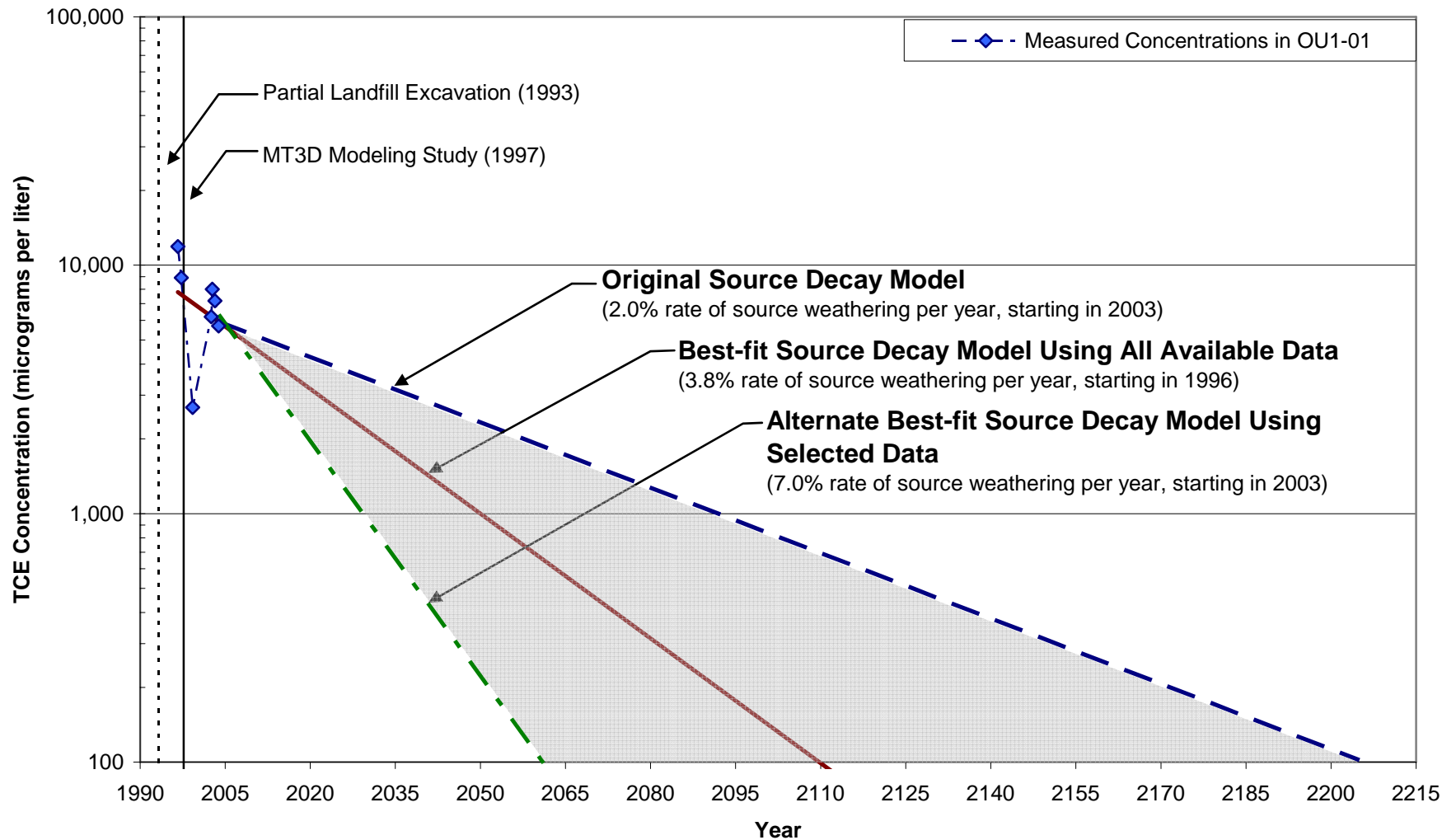
FIGURE 4.37 MEASURED AND PREDICTED TCE CONCENTRATIONS OVER TIME OU1, ALTUS AFB, OKLAHOMA FIELD-SCALE EVALUATION OF MNA FOR DISSOLVED CHLORINATED SOLVENT PLUMES
