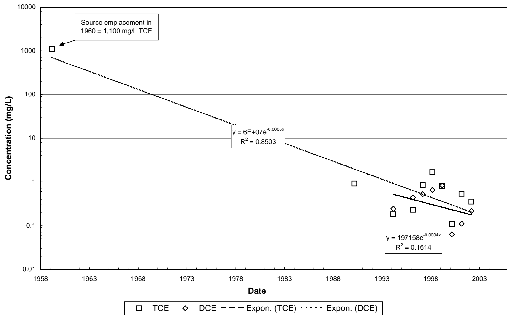
Figure 32: Source Decay Rate in well H127S - Wurtsmith AFB
