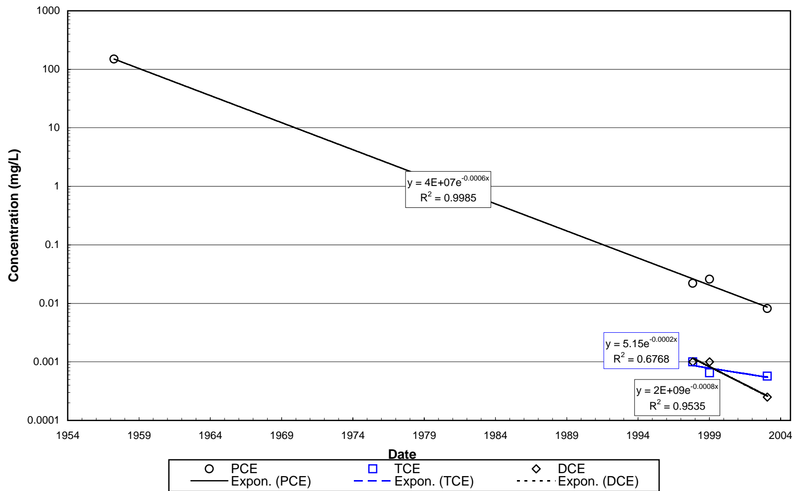
Figure 28d: Source Decay Rate in well 30MW0426B - Ashumet, MMR
