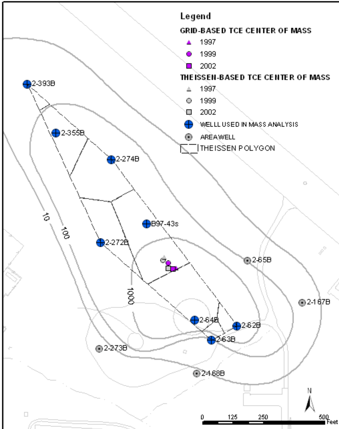
FIGURE 4.6 LOCATION OF CENTER OF MASS FOR TCE SITE FTA-2, TINKER AFB, OKLAHOMA FIELD-SCALE EVALUATION OF MNA FOR DISSOLVED CHLORINATED SOLVENT PLUMES
