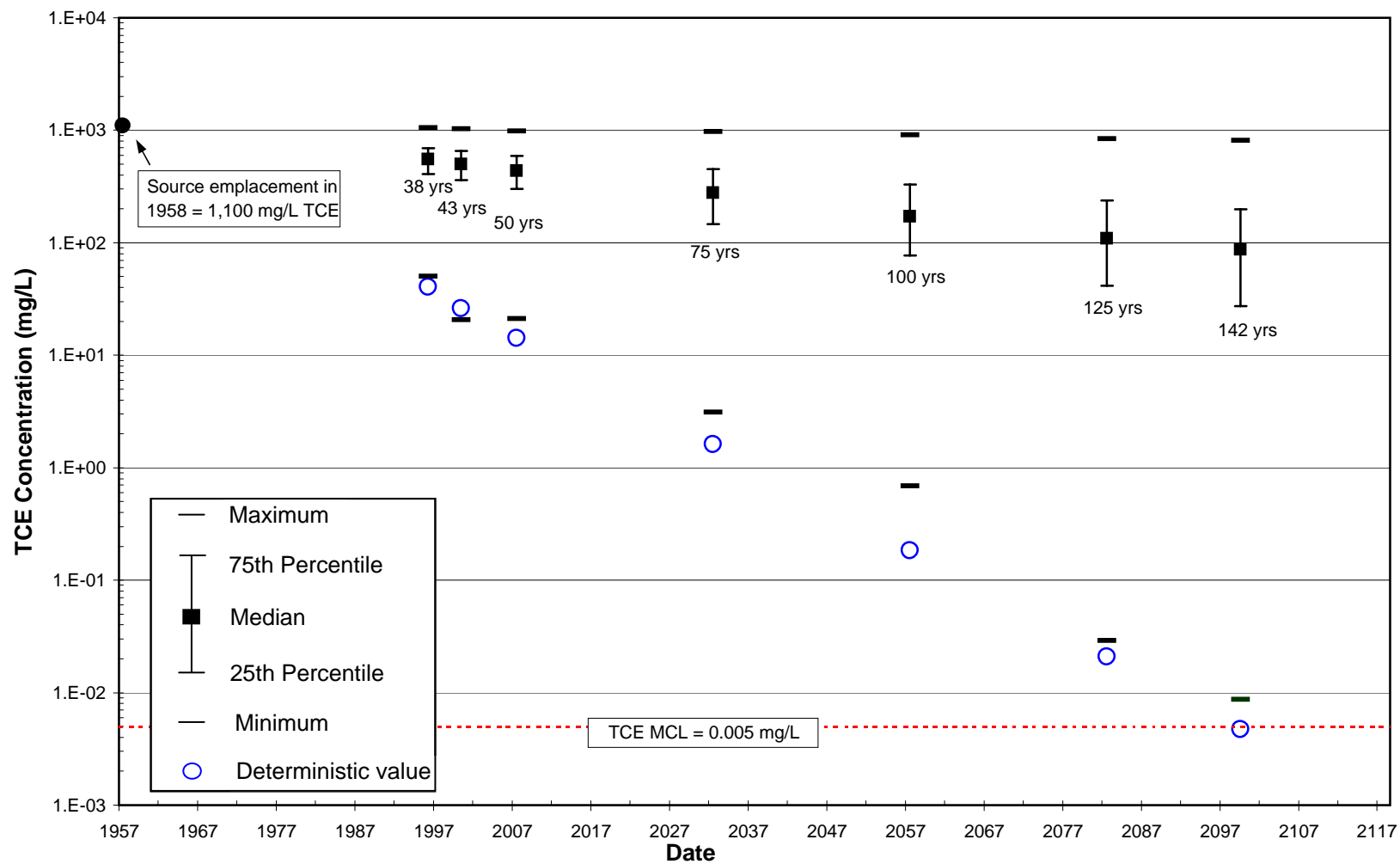
Figure 13a: BIOCHLOR Deterministic and Stochastic Model TCE Predictions at the Source Over Time - CCAS
