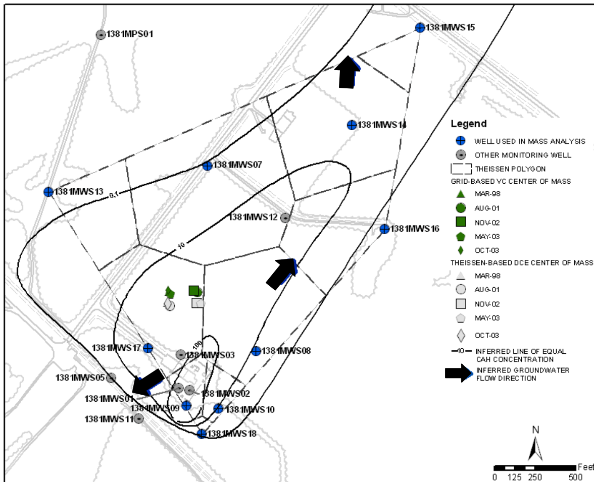
FIGURE 4.28 LOCATION OF THE CENTERS OF MASS FOR VC FACILITY 1381, CAPE CANAVERAL AFS, FLORIDA FIELD-SCALE EVALUATION OF MNA FOR DISSOLVED CHLORINATED SOLVENT PLUMES
