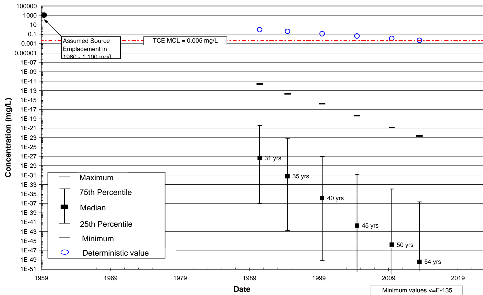
Figure 34a: BIOCHLOR Deterministic and Stochastic Model TCE Predictions at the Source Over Time - Wurtsmith AFB
