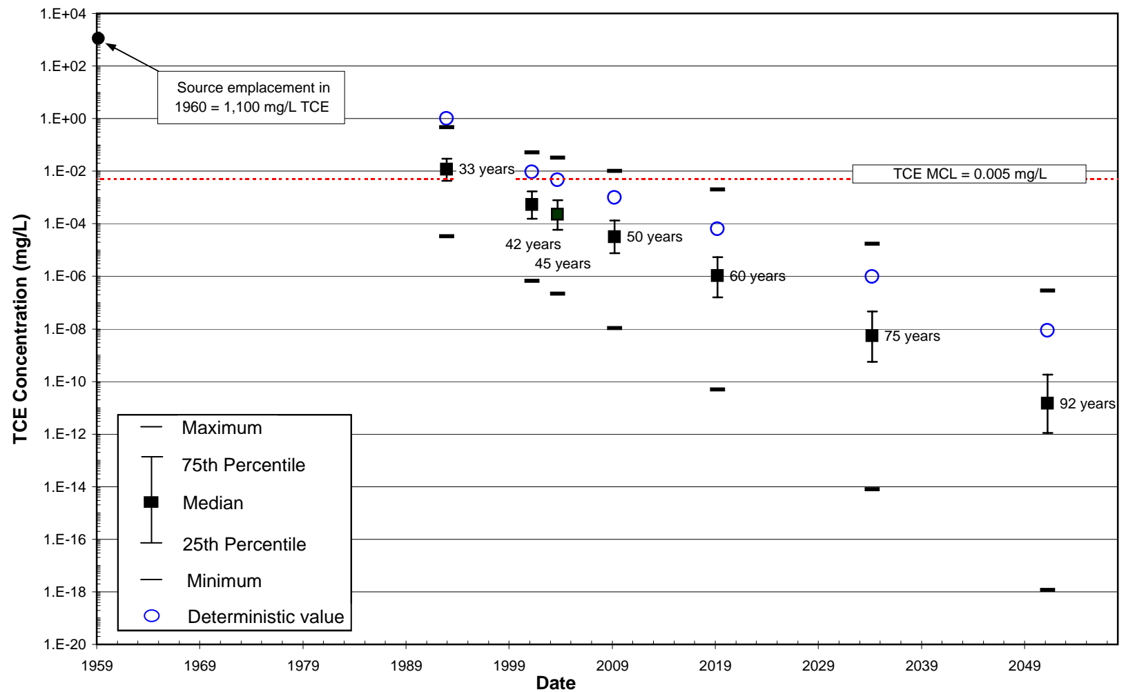
Figure 26: BIOCHLOR Deterministic and Stochastic Model TCE Predictions at the Source Over Time - Warren AFB
