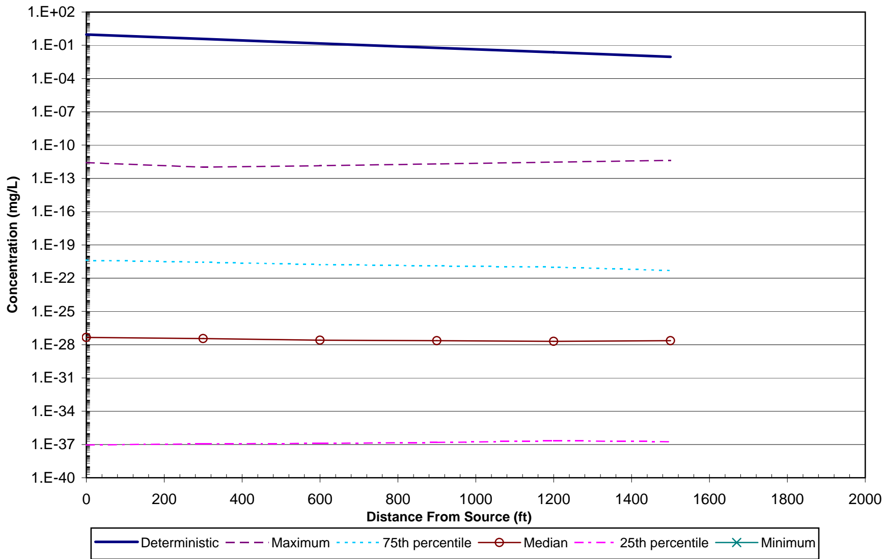
Figure 33a: TCE Deterministic and Stochastic Modeled Concentrations in 1991 - Wurtsmith AFB
