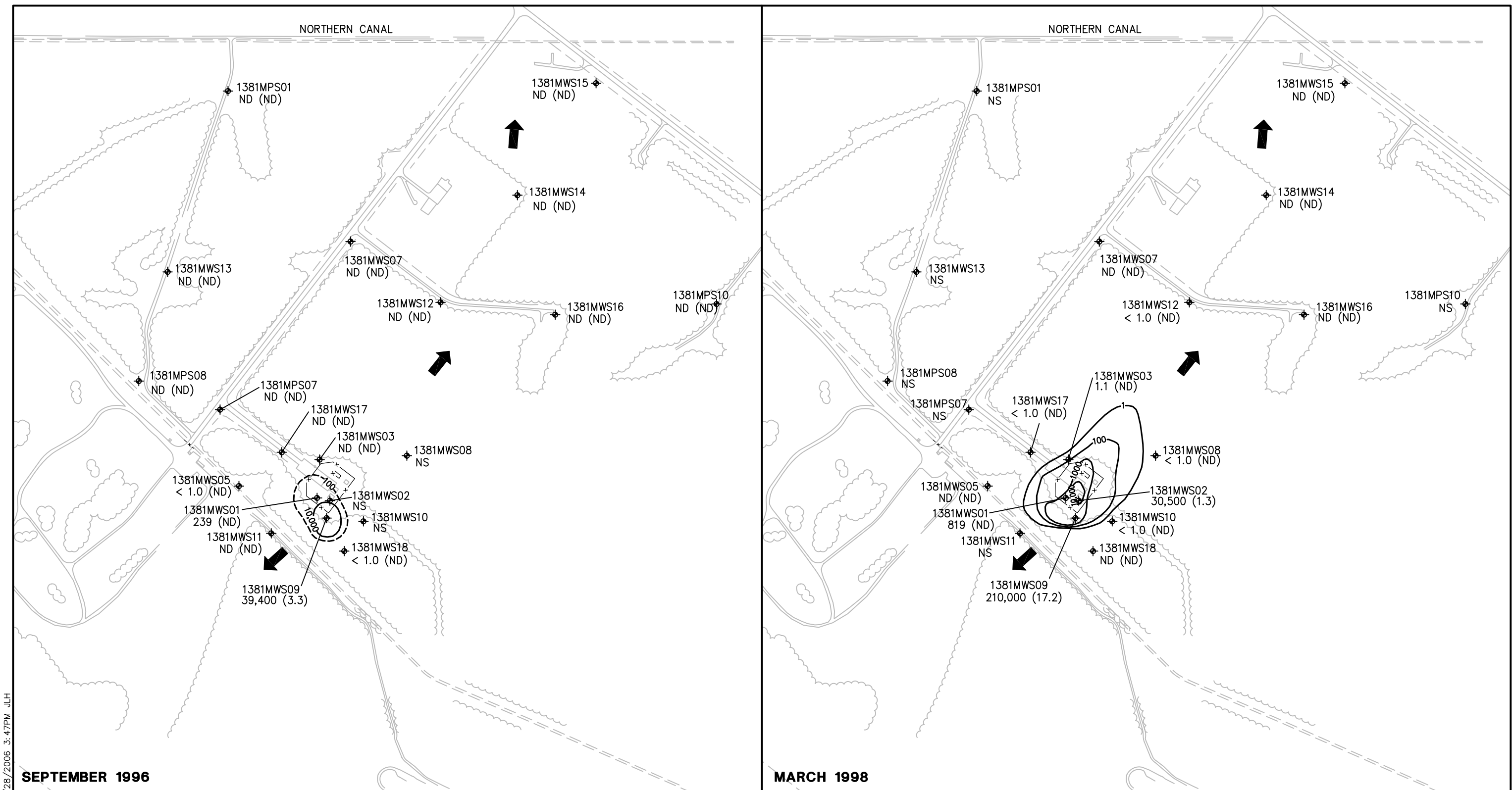
FIGURE 4.20 PCE AND TCE CONCENTRATIONS MEASURED AT SHALLOW MONITORING WELLS/POINTS FACILITY 1381, CAPE CANAVERAL AFS, FL Field-scale Evaluation of MNA for Dissolved Chlorinated Solvent Plumes PARSONS Denver, Colorado
