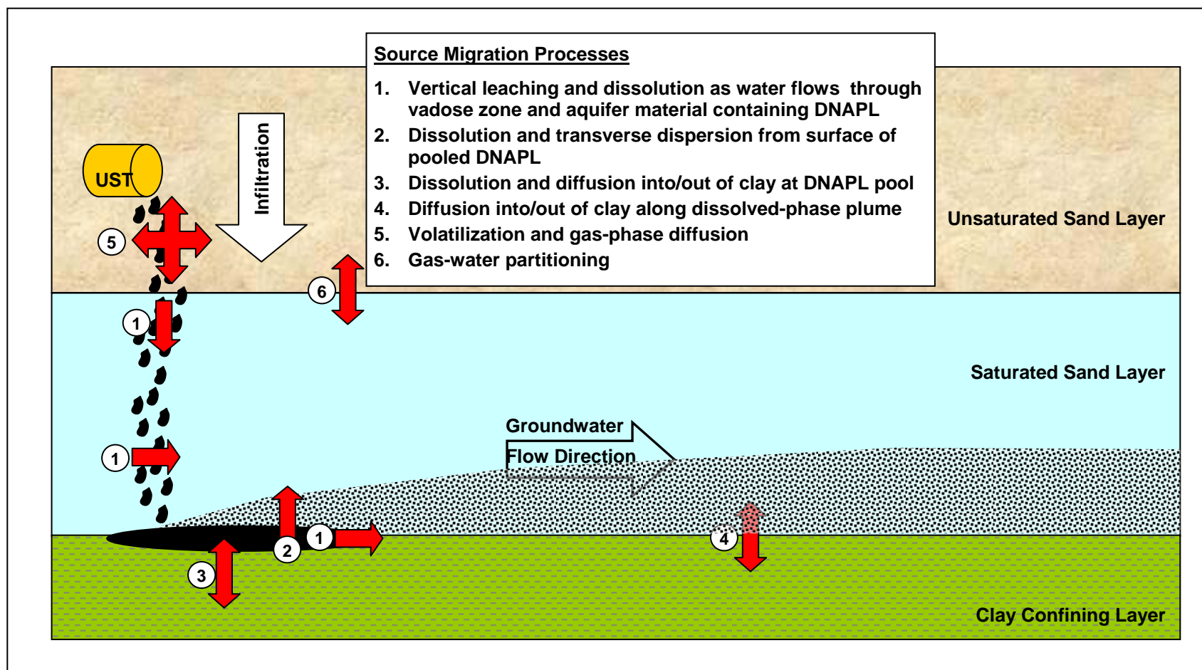
FIGURE 3.1 CONCEPTUAL MODEL OF MECHANISMS AFFECTING DNAPL MIGRATION AND DISSOLUTION FIELD-SCALE EVALUATION OF MNA FOR DISSOLVED CHLORINATED SOLVENT PLUMES
