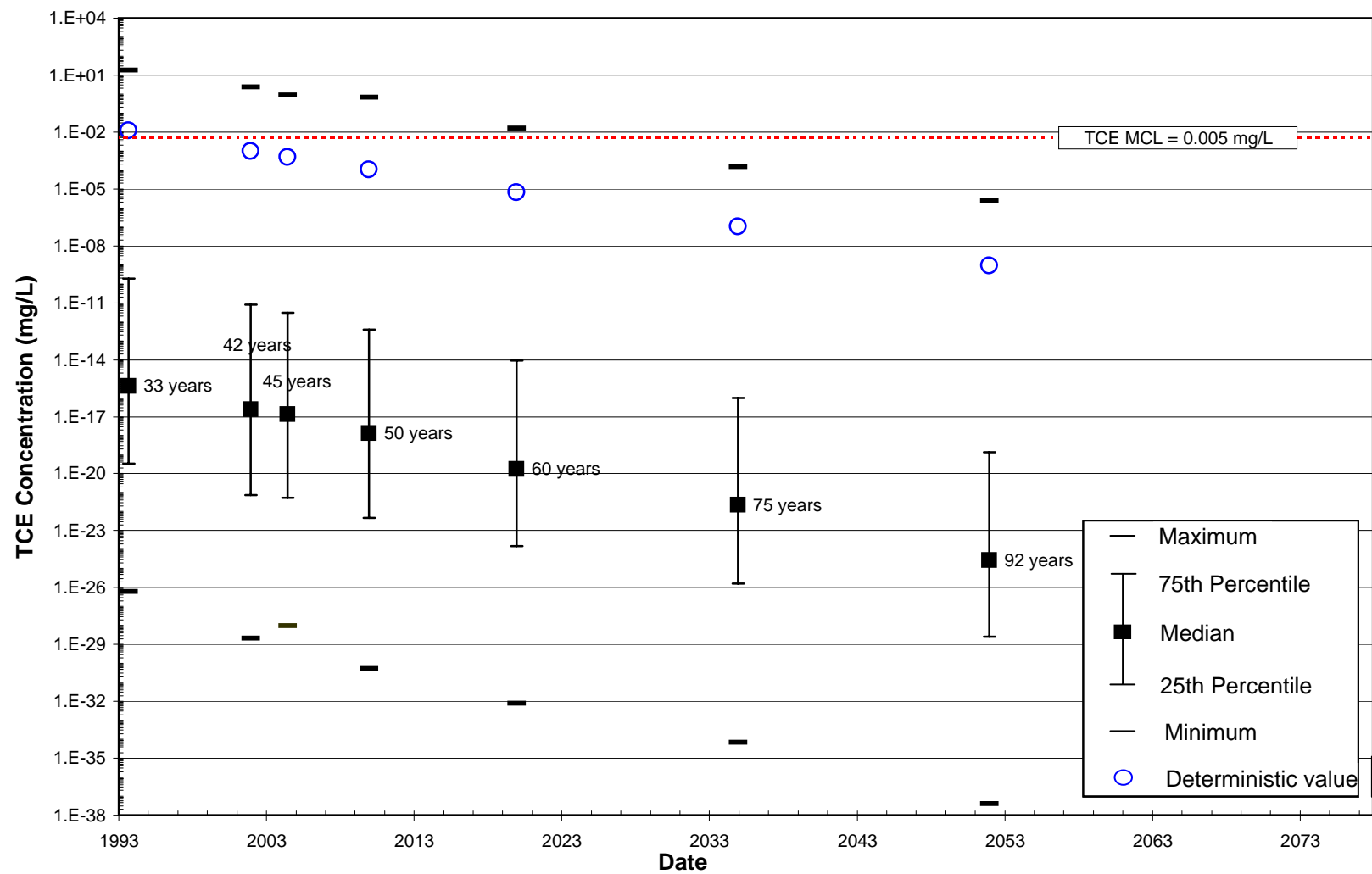
Figure 27: BIOCHLOR Deterministic and Stochastic Model TCE Predictions 1,000 ft Downgradient of the Source Over Time - Warren AFB
