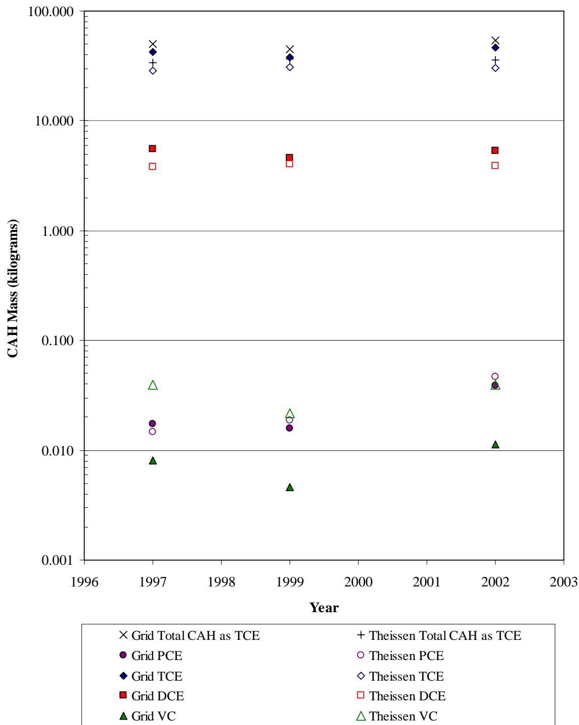
FIGURE 4.5 ESTIMATED DISSOLVED MASS OF CAH COMPOUNDS SITE FTA-2, TINKER AFB, OKLAHOMA FIELD-SCALE EVALUATION OF MNA FOR DISSOLVED CHLORINATED SOLVENT PLUMES
