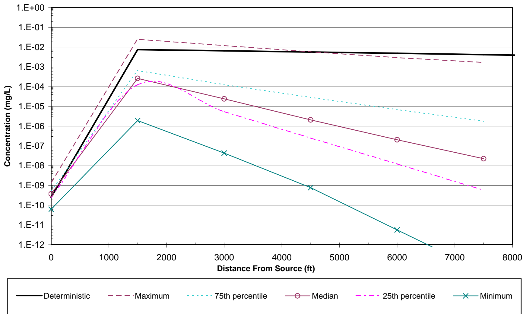
Figure 29b: TCE Deterministic and Stochastic Modeled Concentrations in 1998 - Ashumet Valley, MMR
