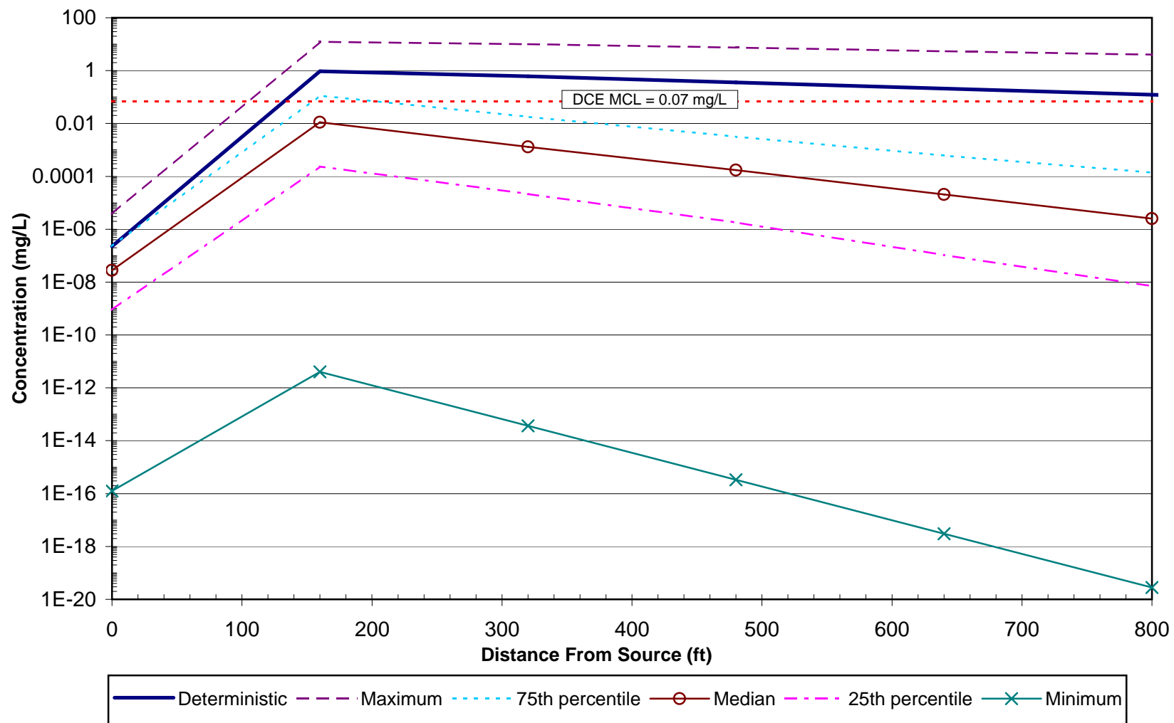
Figure 22: DCE Deterministic and Stochastic Modeled Concentrations in 1997 - Tinker AFB
