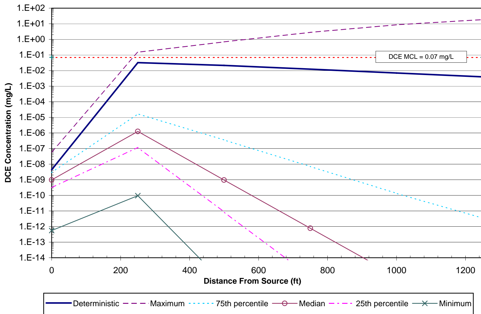
Figure 25b: DCE Deterministic and Stochastic Modeled Concentrations in 1993 - Warren AFB
