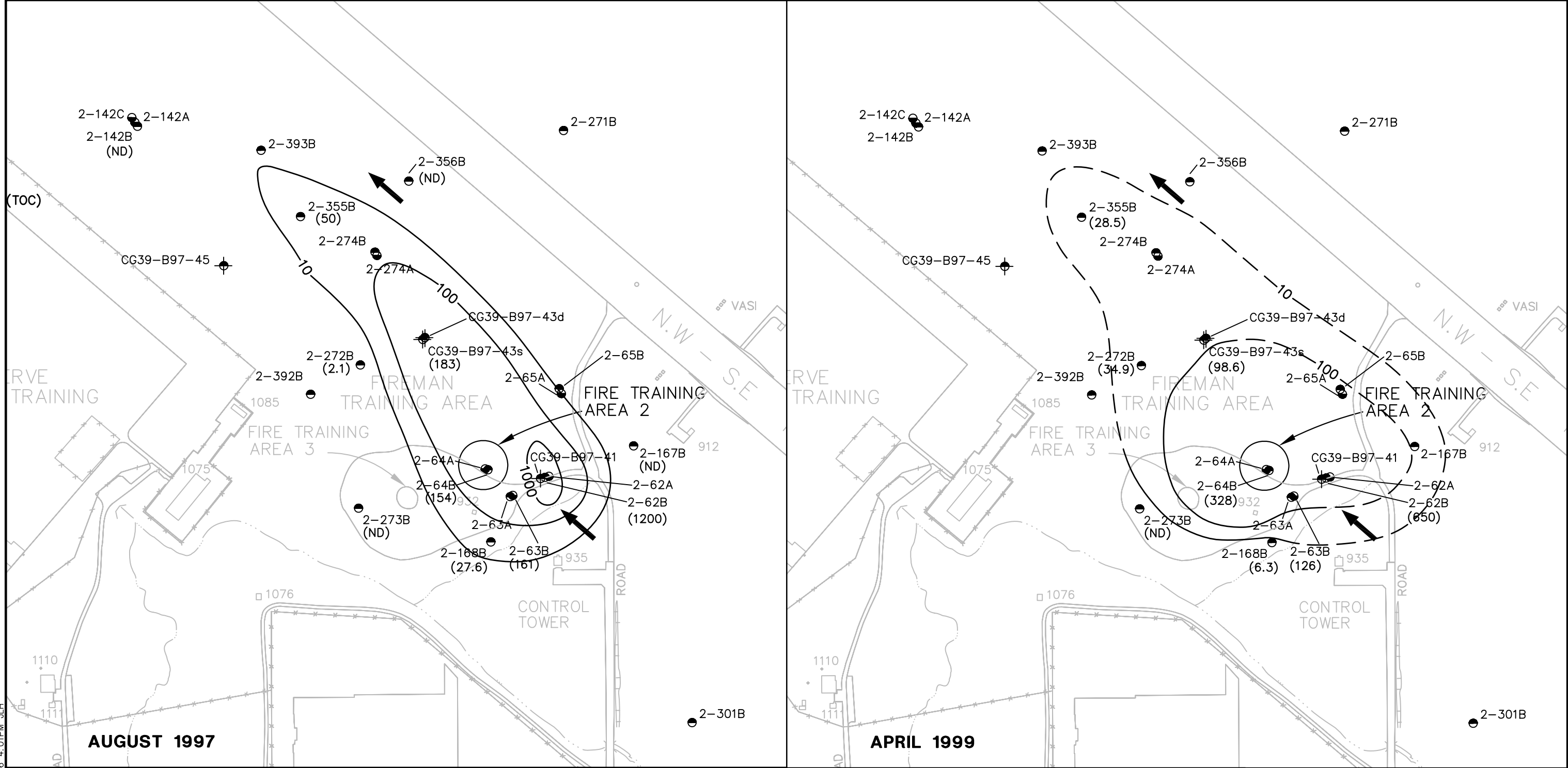
FIGURE 4.2 CONCENTRATION OF cis-1,2-DCE IN UPPER USZ GROUNDWATER AUGUST 1997 AND APRIL 1999 SITE FTA-2, TINKER AFB, OK
