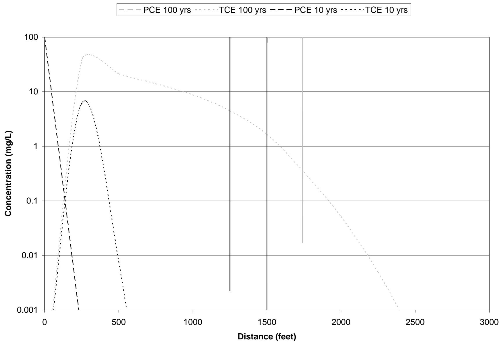
Figure 4c: Biodegradation of PCE to TCE for 3.65 1/yr
