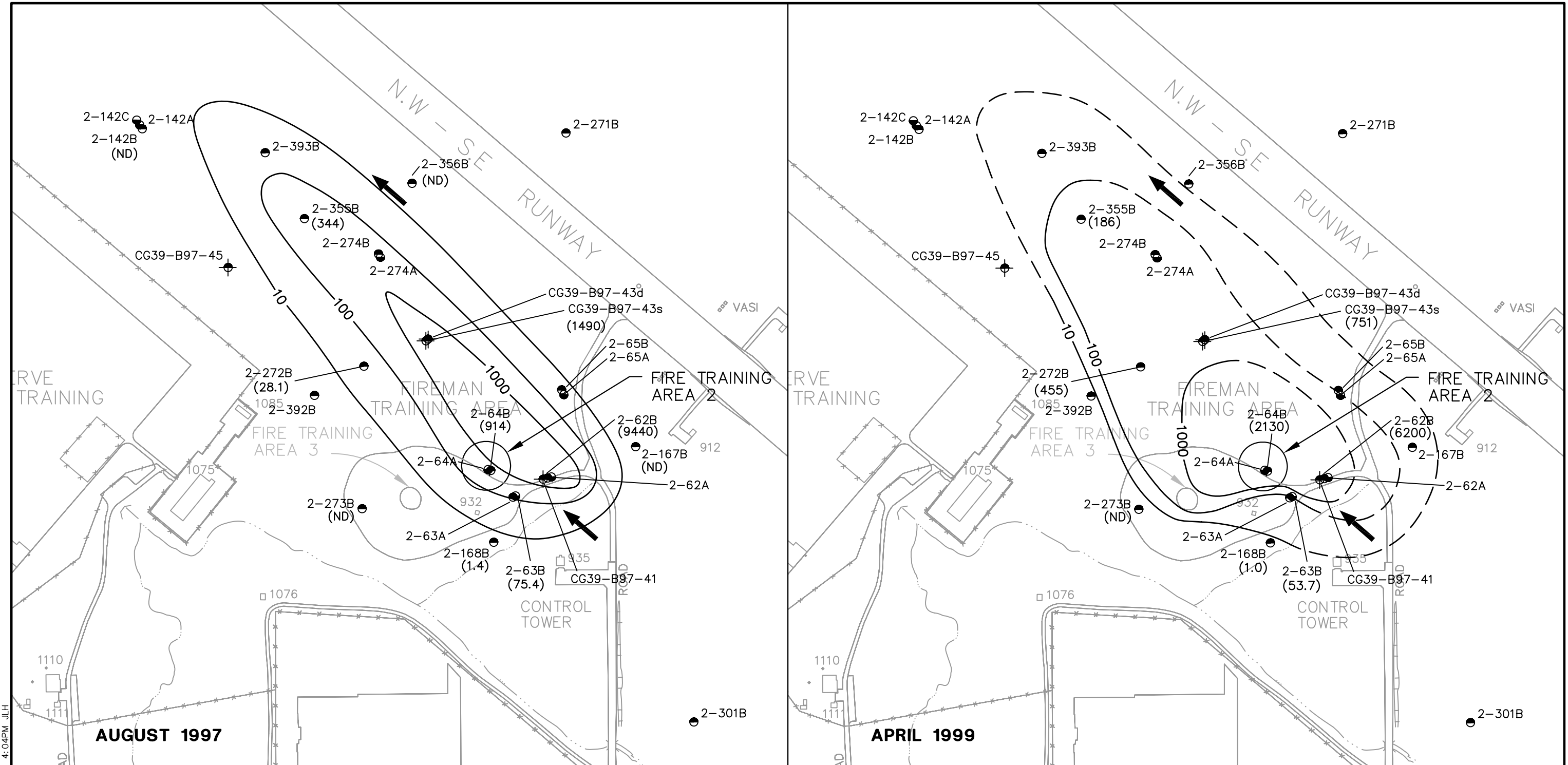
FIGURE 4.1 CONCENTRATION OF TCE IN UPPER USZ GROUNDWATER AUGUST 1997 AND APRIL 1999 SITE FTA-2, TINKER AFB, OK
