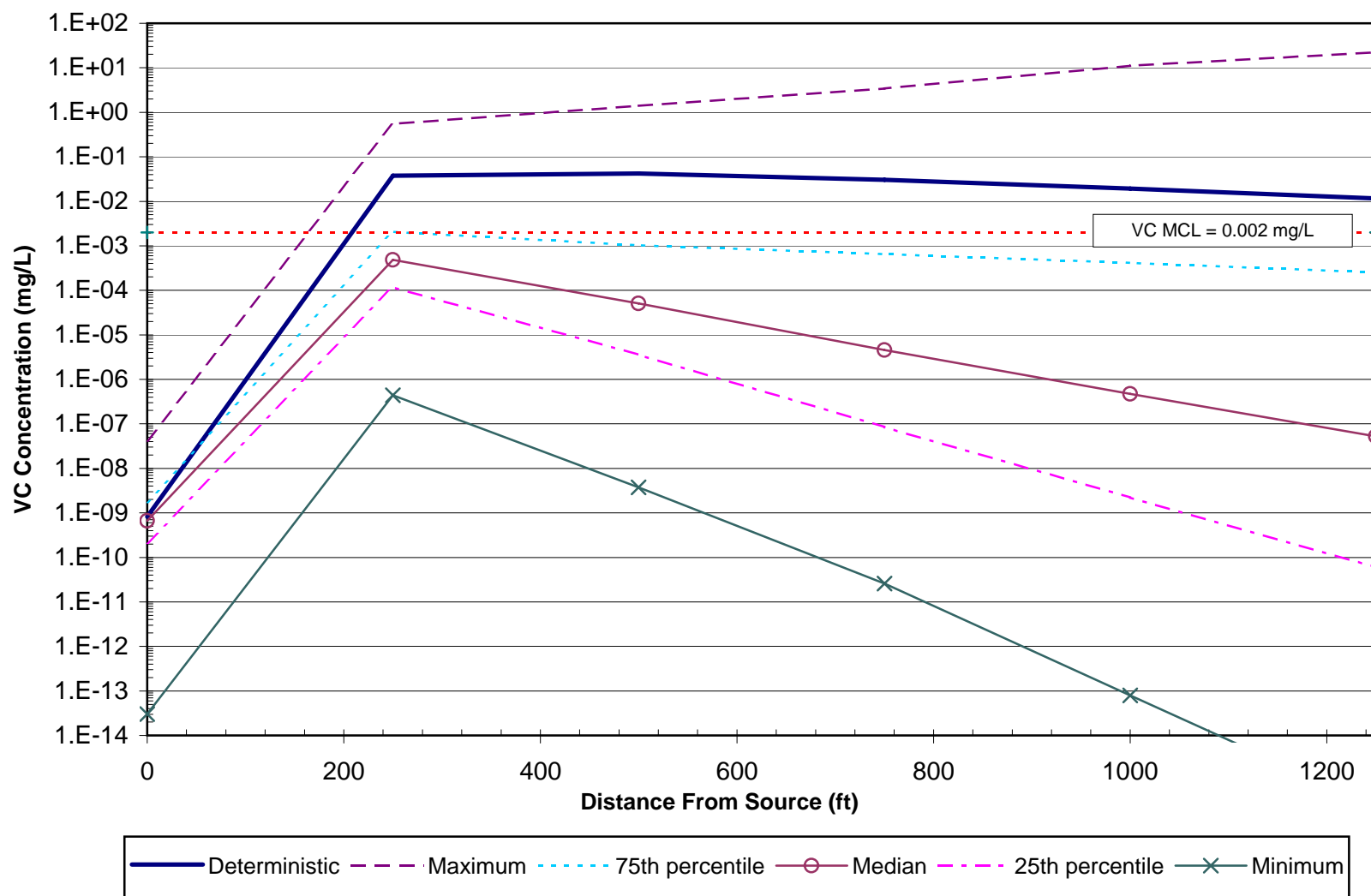
Figure 25c: VC Deterministic and Stochastic Modeled Concentrations in 1993 - Warren AFB
