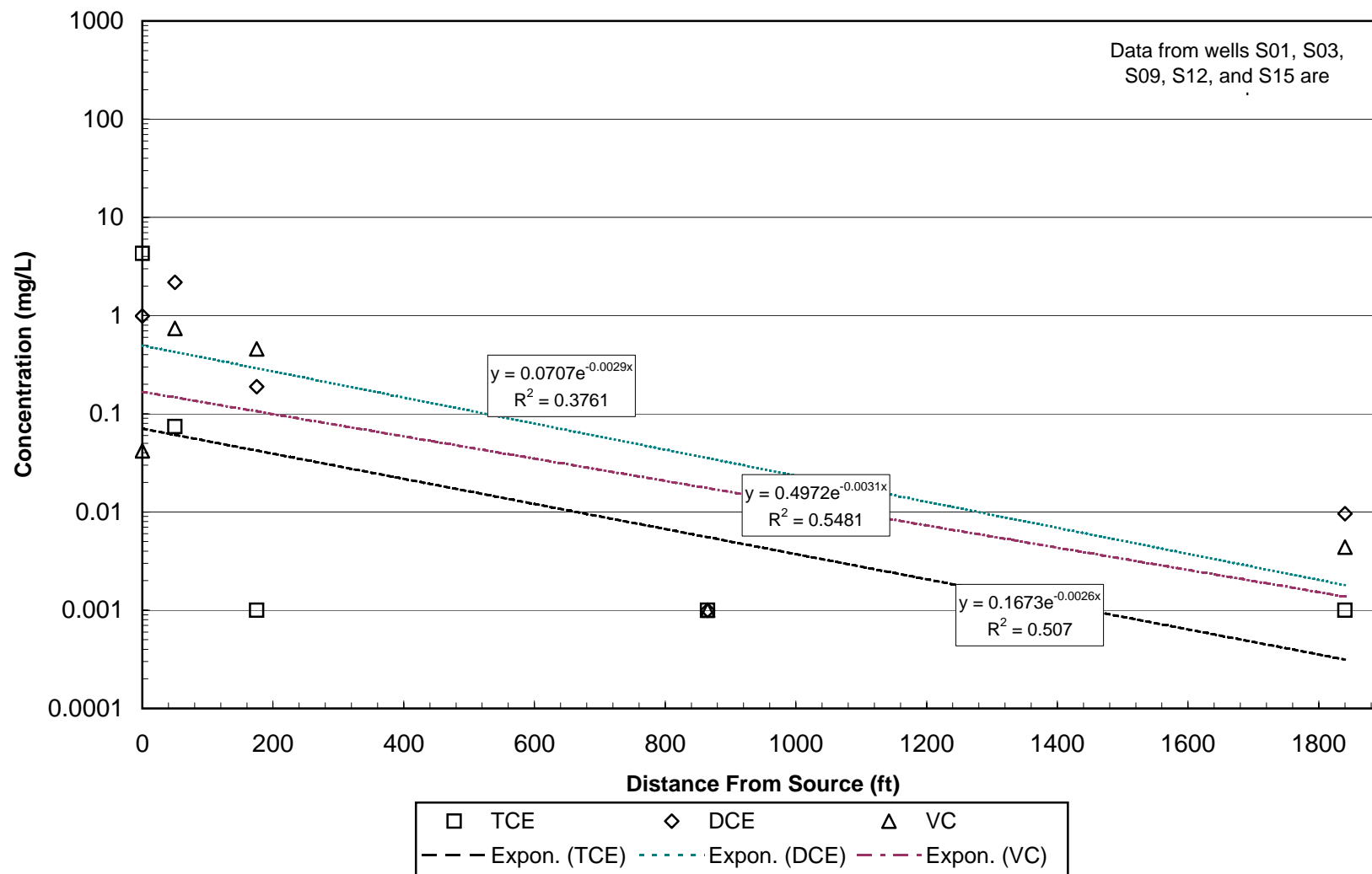
Figure 9c: 2001 Plume Centerline Concentrations - CCAS
