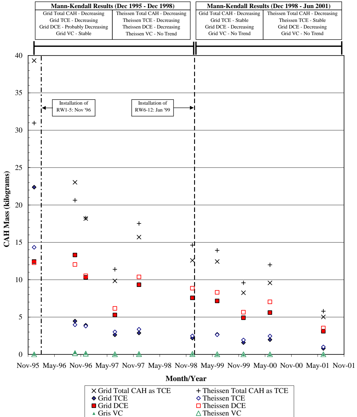
FIGURE 4.33 ESTIMATED DISSOLVED MASS OF CAH COMPOUNDS FPTA-2, BROOKS CITY-BASE, TEXAS FIELD-SCALE EVALUATION OF MNA FOR DISSOLVED CHLORINATED SOLVENT PLUMES
