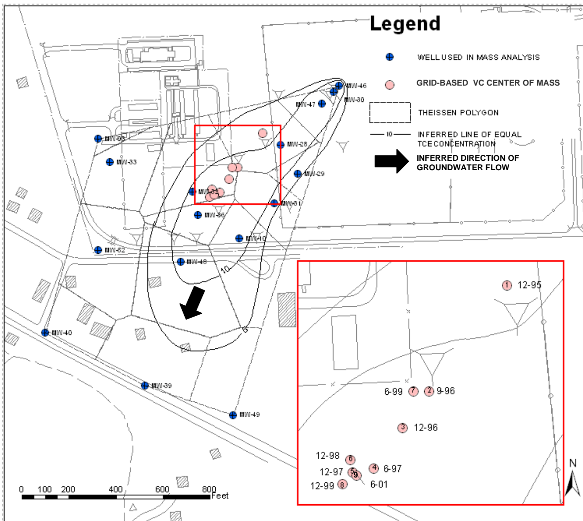
FIGURE 4.36 LOCATION OF CENTERS OF MASS FOR VC FPTA-2, BROOKS CITY-BASE, TEXAS FIELD-SCALE EVALUATION OF MNA FOR DISSOLVED CHLORINATED SOLVENT PLUMES
