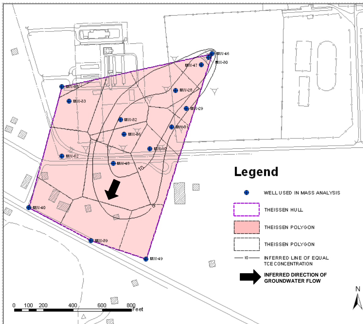
FIGURE 4.32 MODEL DOMAIN AND COMMON WELLS FOR MASS-BASED CALCULATIONS FPTA-2, BROOKS CITY-BASE, TEXAS FIELD-SCALE EVALUATION OF MNA FOR DISSOLVED CHLORINATED SOLVENT PLUMES
