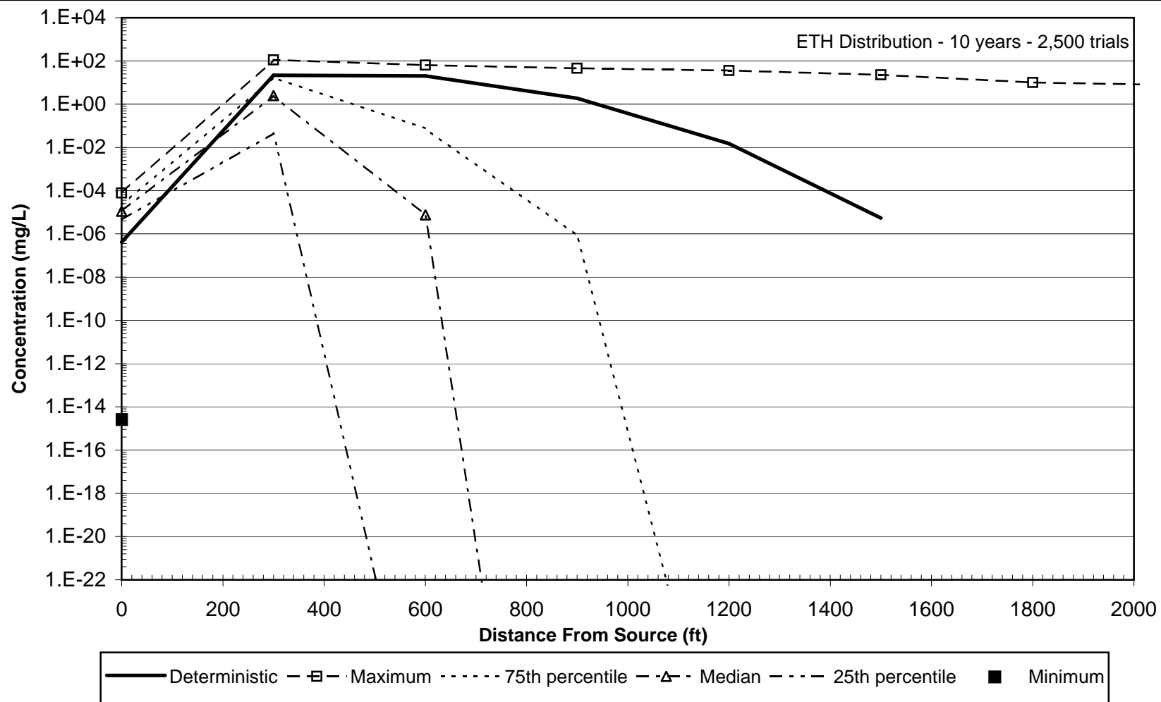
Figure 6e: Deterministic and Stochastic ETH Concentrations with Biodegradation Synthetic Case Study
