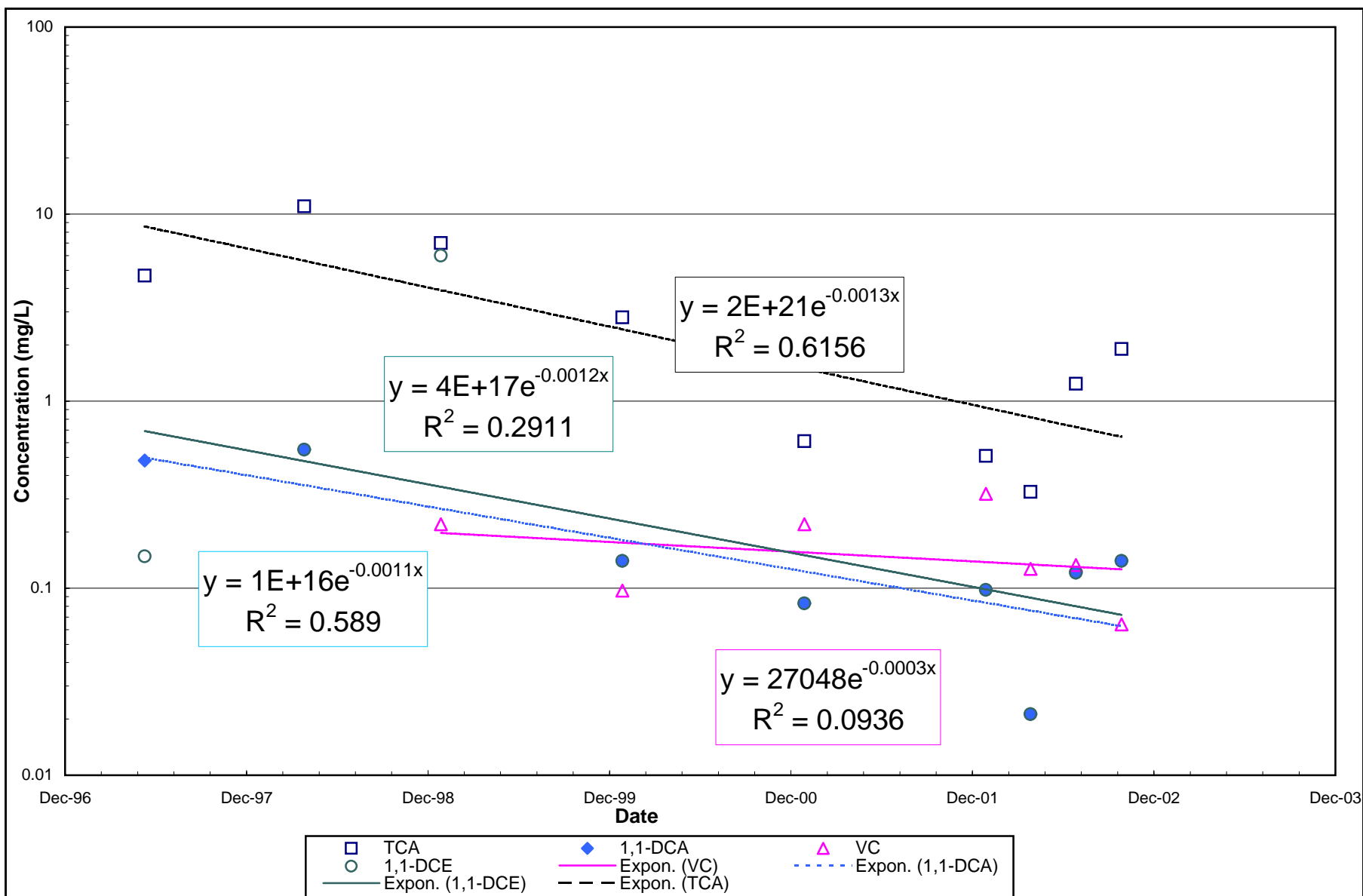
Figure 15b: Source Decay Rates in well MW-117 - Shaw AFB
