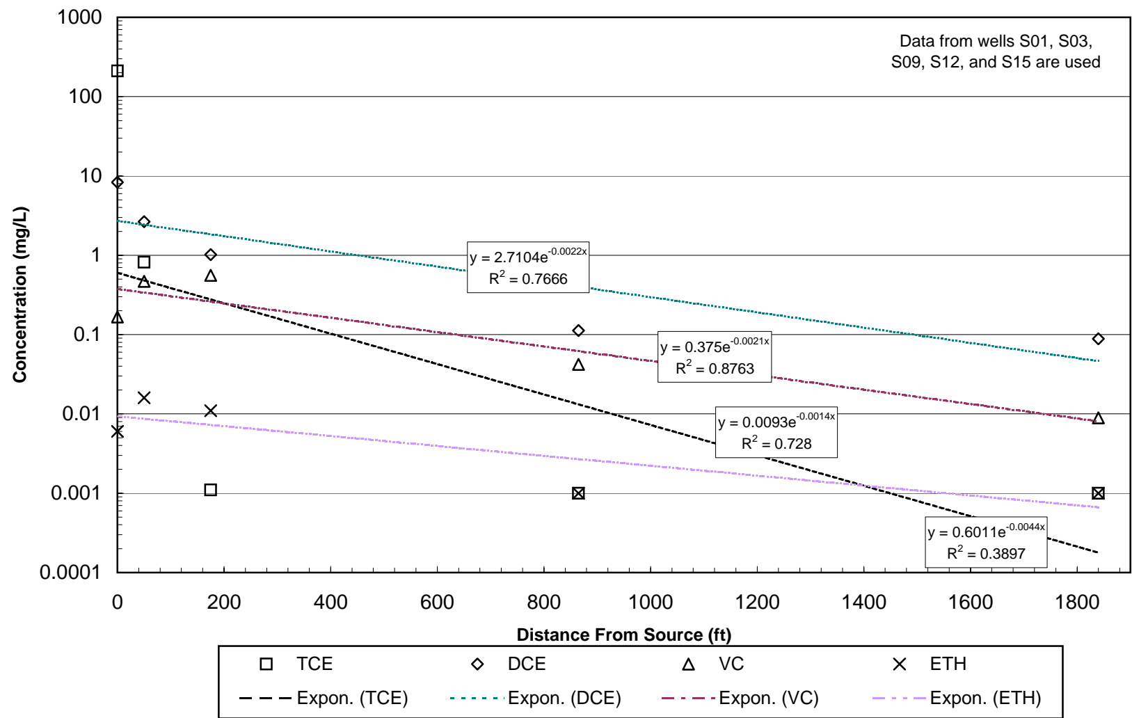
Figure 9b: 1998 Plume Centerline Concentrations - CCAS
