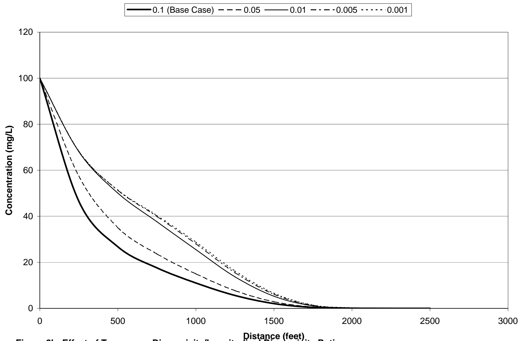
Figure 2b: Effect of Transverse Dispersivity/Longitudinal Dispersivity Ratio
