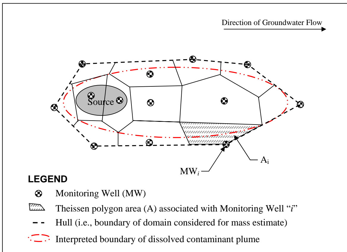
FIGURE A.1 SCHEMATIC OF THE THEISSEN POLYGON APPROACH FOR ESTIMATING CONTAMINANT MASS USING DISCRETE MONITORING POINT CONCENTRATION DATA.
