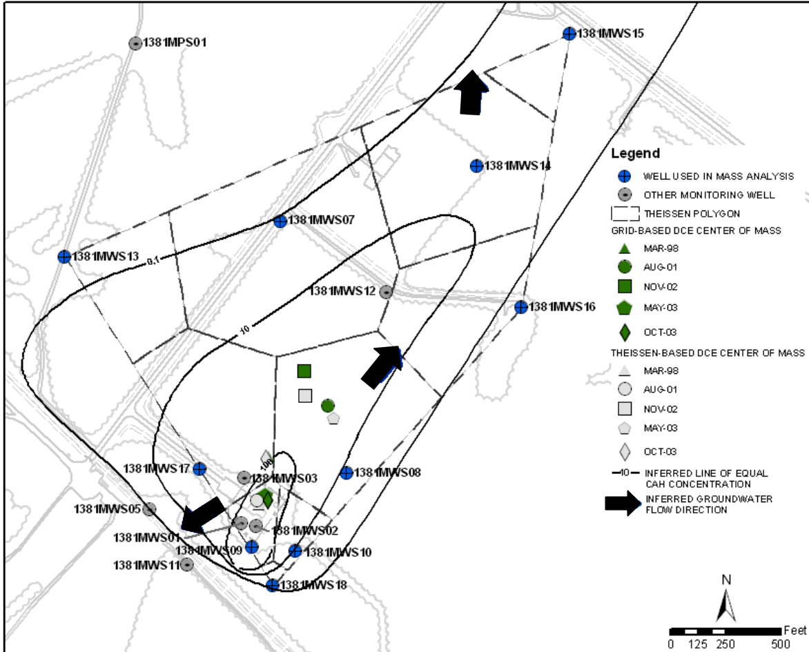
FIGURE 4.27 LOCATION OF CENTERS OF MASS FOR CIS-1,2-DCE FACILITY 1381, CAPE CANAVERAL AFS, FLORIDA FIELD-SCALE EVALUATION OF MNA FOR DISSOLVED CHLORINATED SOLVENT PLUMES
