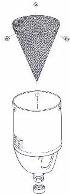
Figure 23. Components of a mosquito concentrator
