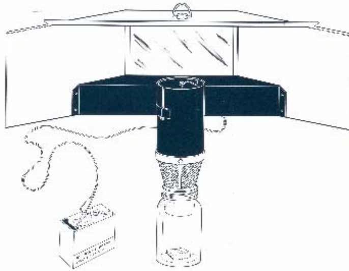
Figure 13. CDC Fay-Prince trap with gel-cell battery and collection jar
