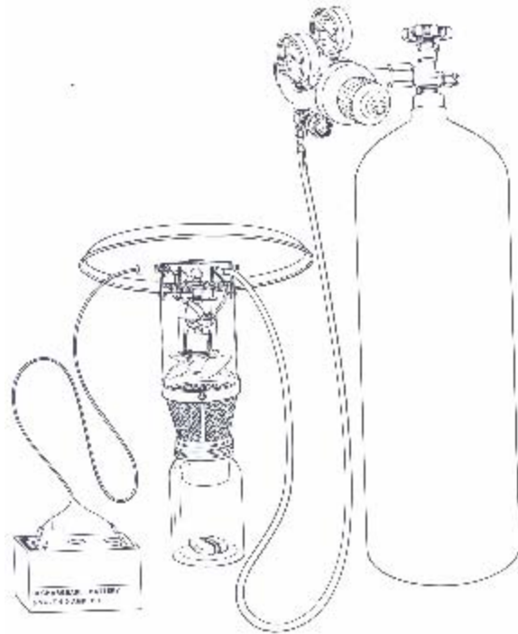
Figure 6. SSAM trap with collection net shown suspended from tree limb
