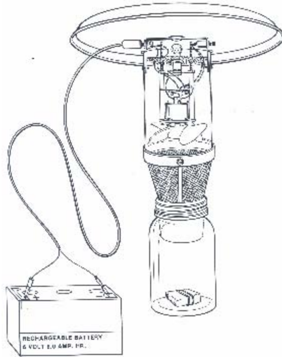
Figure 2. Illustration of SSAM trap with gel-cell battery and collection jar
