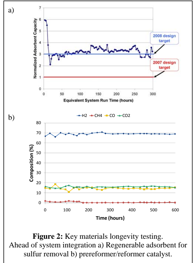
Figure 2: Key materials longevity testing. Ahead of system integration a) Regenerable adsorbent for sulfur removal b) prereformer/reformer catalyst.
