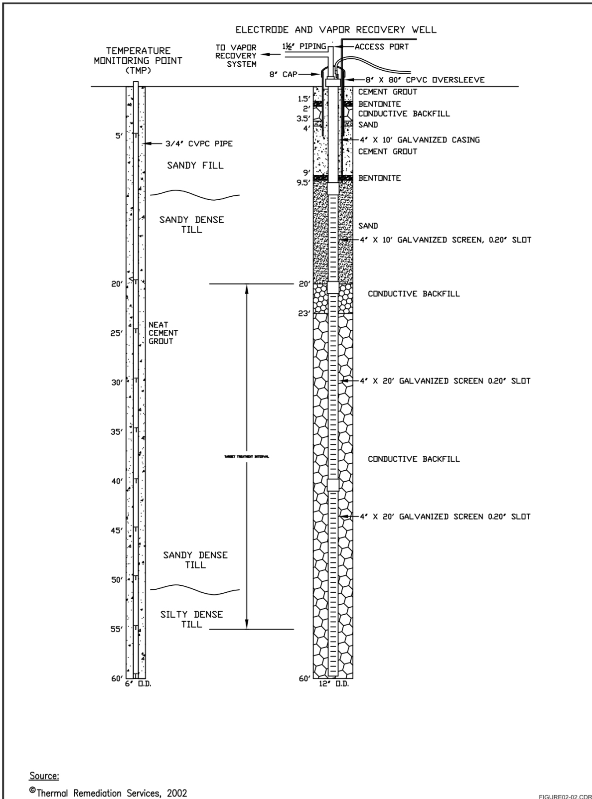
Figure 2-3. Electrode Construction and Geologic Stratification Detail
