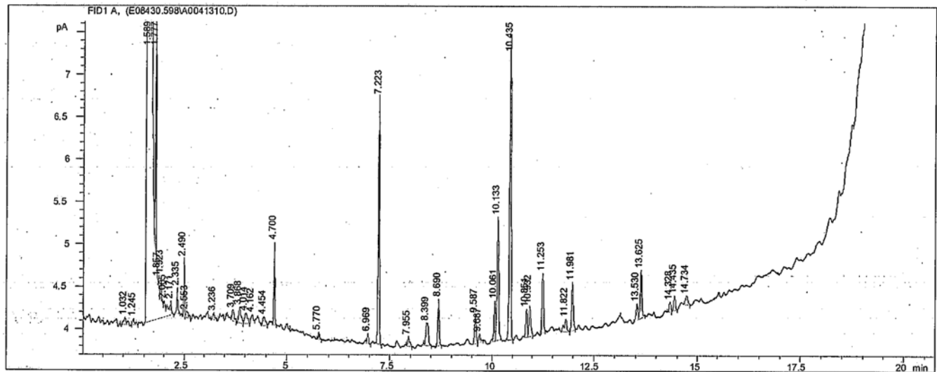
Figure 2. Gas chromatography fatty acid analysis of parent strain (top) and cpnit-1 (bottom).
