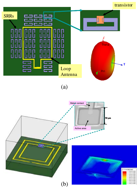
Figure 1. (a) SRRs and HPTs enabled tuneable loop antenna and its radiation pattern, (b) tunable SRR unit cell with an embedded HPT and simulated E-field pattern using HFSS
