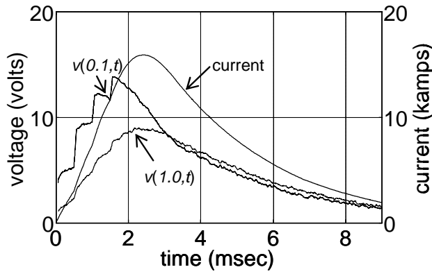
Fig. 5. Rail-to-rail voltages at breech and muzzle with current trace superimposed. Data is shown for 0.5 ms staging.
