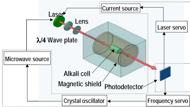
Fig. 1: Schematic of Coherent Population Trapping architecture used in CSAC
