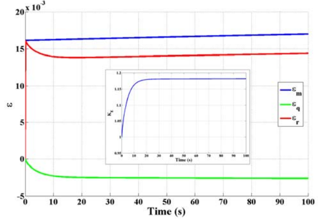
Figure 8. This plot shows the system response for a 1 MPa stress step input. The mechanical strain, \epsilon_m , is offset by the charge driven strain, \epsilon_q , to give a resultant strain of \epsilon_r . The programmable material increases the apparent stiffness by 18% (inset).
