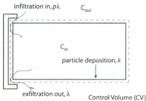
Figure 1. Schematic representation of the air exchange (infiltration and exfiltration), as well as particle deposition loss components in the mechanistic model.
