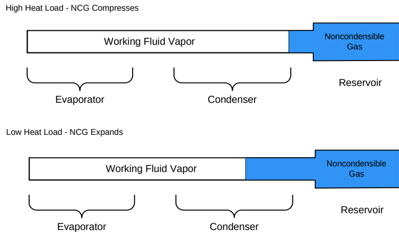
Figure 3 VCHP Operation
