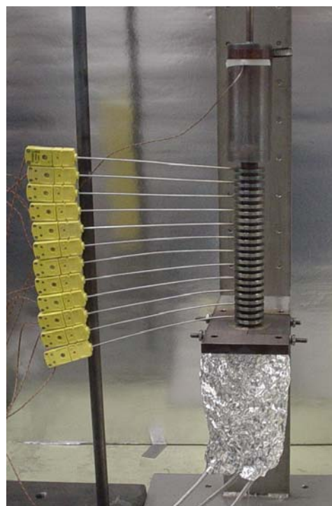
Figure 9: Stainless Steel/Cesium VCHP test apparatus.
