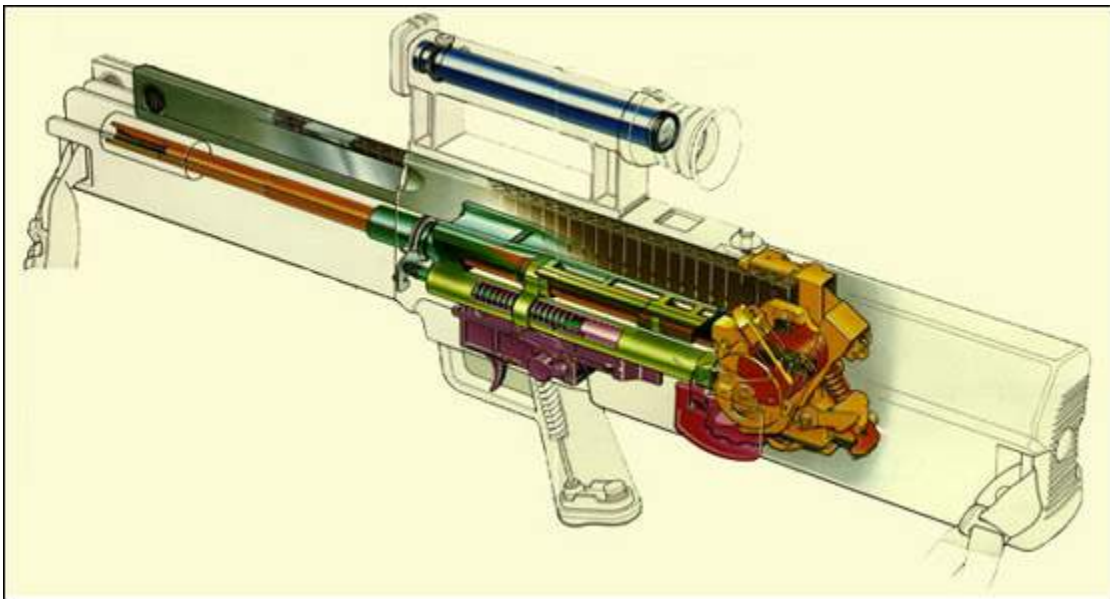
Figure 1B Heckler and Kock 4.7mm G11 automatic weapon system, internal view
