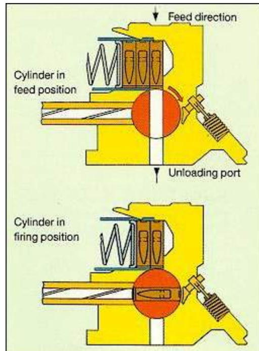
Figure 2 Schematic of 4.7mm H&K G11 bolt and feeding system.
