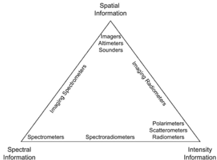
Figure 9. Remote Sensing Instruments and Information (Elachi & Van Zyl, 2006)
