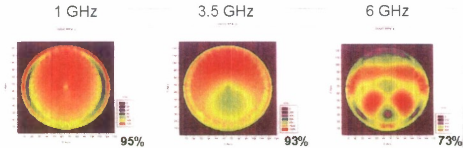
Figure 2. Electric field distributions in the near field at 1, 3.5 and 6 GHz, where % refers to the area of the GFF homogeneous to within 30%.
