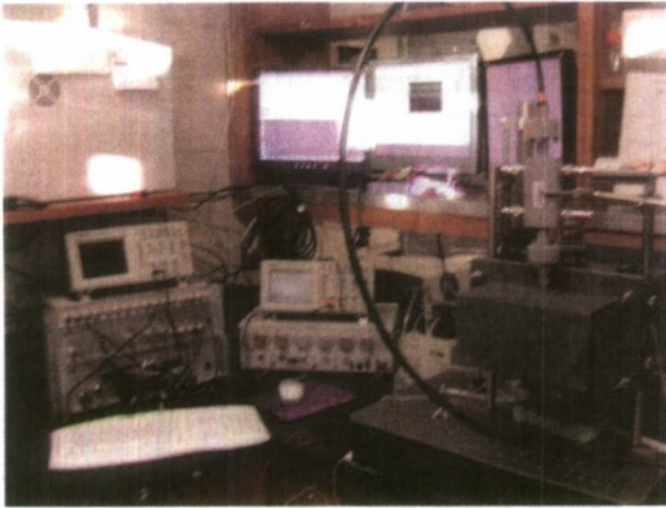
Figure 9. Photograph of the waveguide-based exposure system for assessing RF effects on skeletal muscle contraction (left) and of the RF generating equipment (right).
