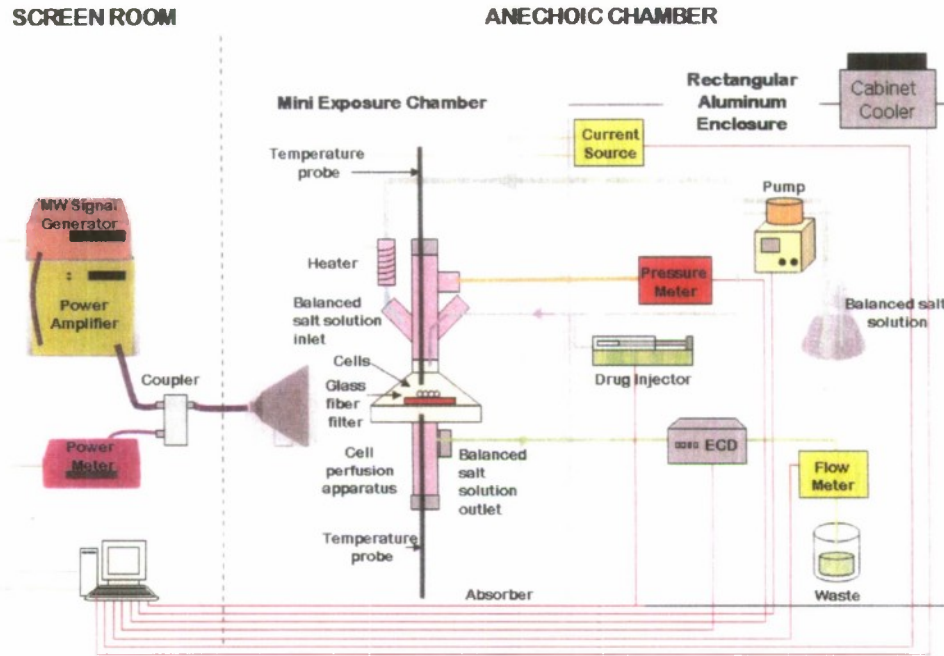
Figure 1. Schematic of the modified free space MW exposure system showing the experimental arrangements inside the anechoic chamber and adjacent screen room.
