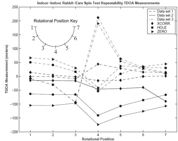
Fig. 1. Variation in analog television TDOA measurement as a function of rotational position for indoor, short-baseline test using "rabbit ears" antennas.
