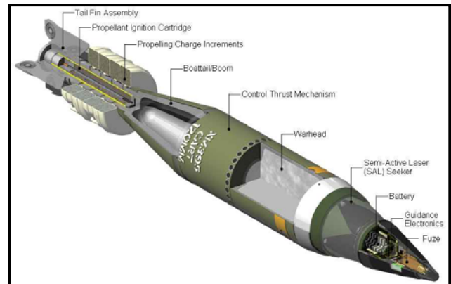
Figure 3. Final PGMM design at conclusion of program.
