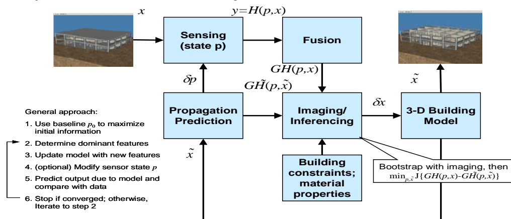
Figure 1 Model-based imaging architecture
