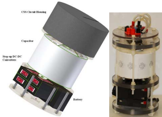
Fig. 3. Seed Source, artist rendering (left) and implementation (right), cf. Fig. 1, part A. [5]
