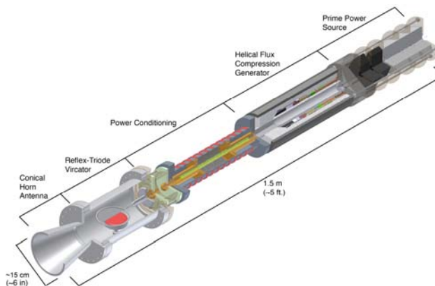
Fig. 2. Cutaway view of the overall explosive-driven HPM system [4].
