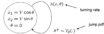
Figure 1B: Stochastic hybrid system (SHS) model for the tumble-and-run motion used by E. Coli. The partial integro-differential equation below the SHS describes the time evolution of the probability density function for the position of the bacteria p .
