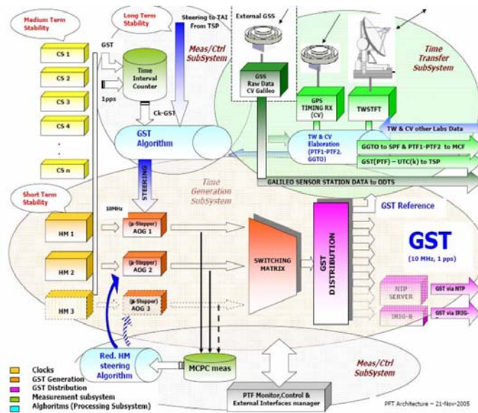
Figure 8. PTF architecture [13].
