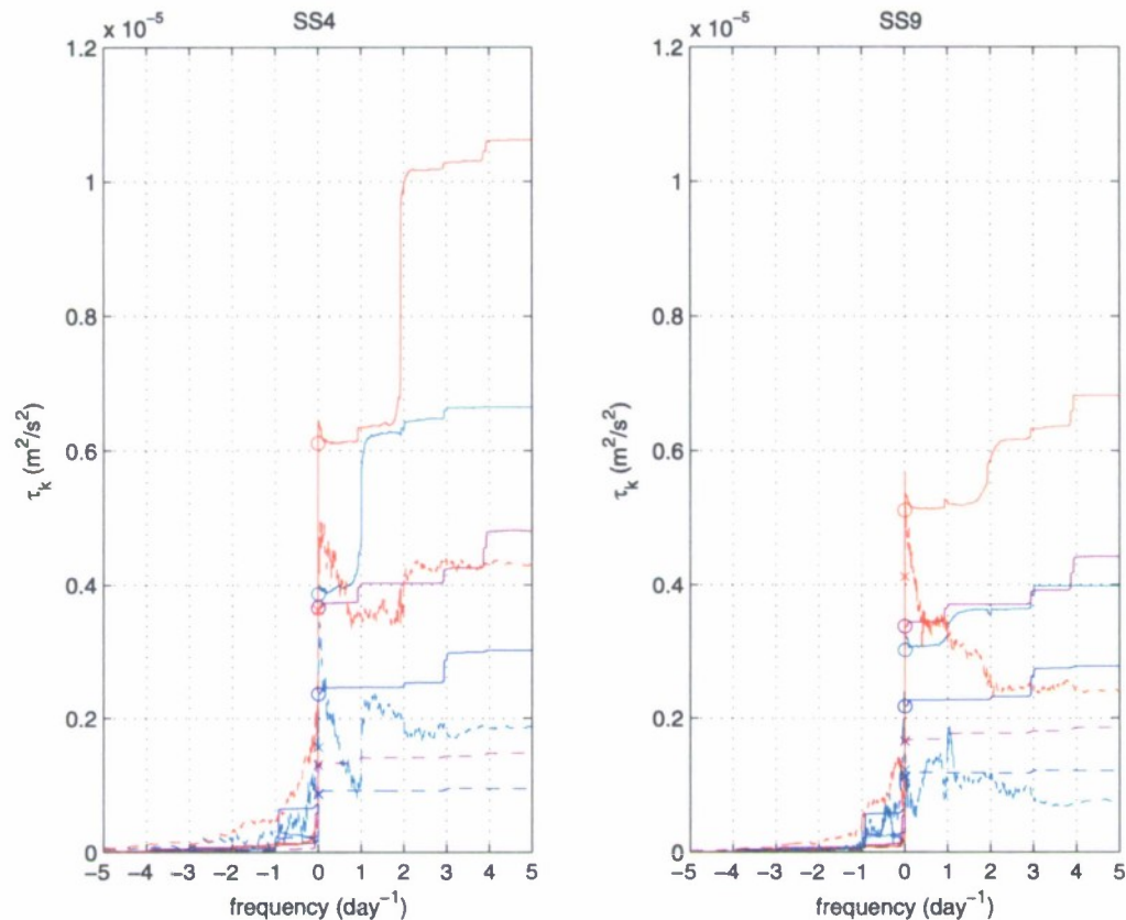
Figure 17. Cumulative sum versus frequency for the convolution integral between the Discrete Fourier Transform of A_z and the Discrete Fourier Transform of \frac{\partial \mathbf{u}}{\partial z} at sites SS4 and SS9. The colors indicate NCOM M_2 (red), NCOM K_1 (cyan), Quoddy M_2 (magenta), and Quoddy K_1 (blue). The solid lines are from the level closest to 1.5 m off the bottom (circles mark the zero frequency values), and the dashed lines are from the level closest to 15 m off the bottom (crosses mark the zero frequency values). In each case, the component of \tau_k with the strongest stress is the one shown.
