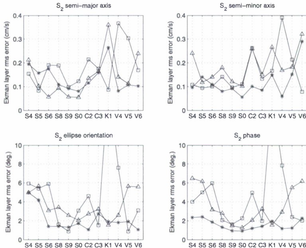
Figure 14. As in Figure 12 but for S_2 tidal currents. The off-scale RMS errors for K1 ellipse orientation and phase are 16.5^\circ and 15.4^\circ , respectively.
