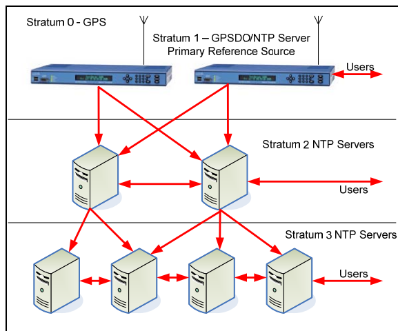
Figure 2. NTP hierarchy.
