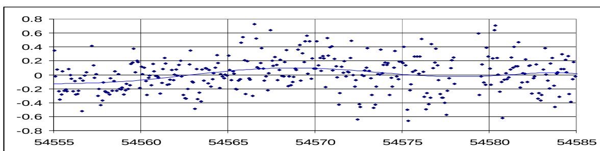
Figure 5.2.2a. Triangle closure \Delta PTB – OP – SP in the data set UTC 0804 (MJD 54555-54585) corresponding to Figure 2.2.6; N = 364 , \text{Std} = 245 ps. The blue curve is a 6 th -order polynomial fit.
