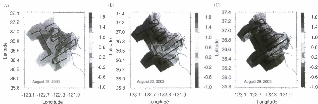
Fig. 17. Chlorophyll- a distributions as sensed from the hyperspectral sensor on board the TWIN OTTER aircraft for (A) August 15, (B) August 20, and (C) August 29, 2003.
