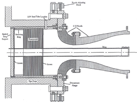
Figure 2. Wind Tunnel Setup
