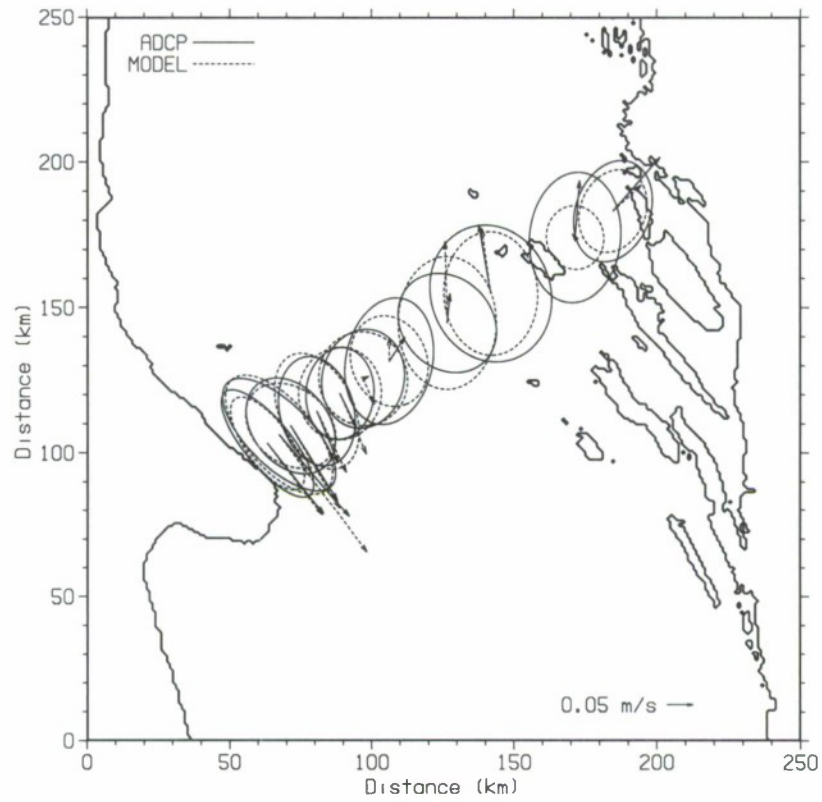
Figure 7. Detided model and ADCP mean current vectors and STD current ellipses at 20 m for period November 2005 through January 2006.
