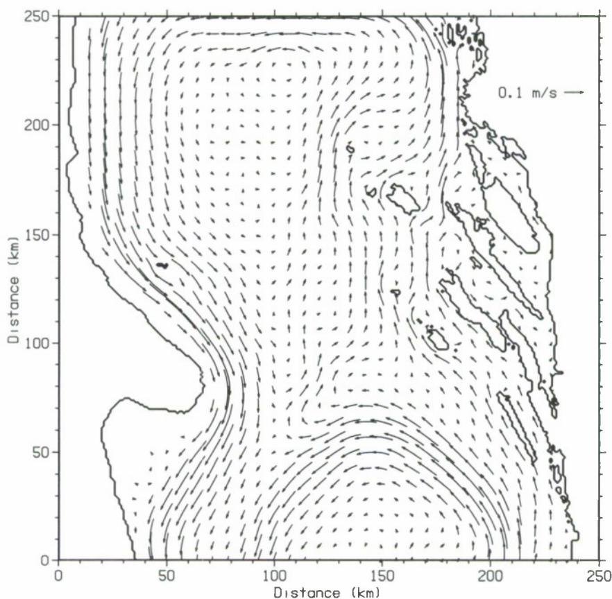
Figure 11. Time-averaged model current at 20-m depth for period February through August 2006.
