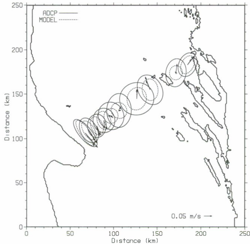
Figure 6. Detided model and ADCP mean current vectors and STD current ellipses at 50 m for period November 2005 through August 2006.
