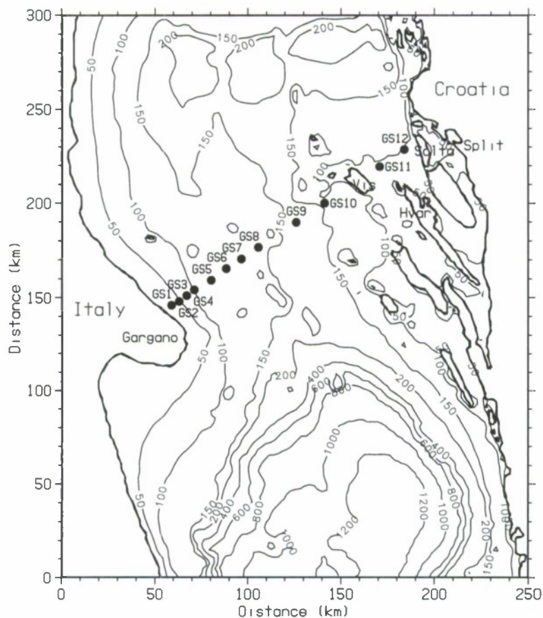
Figure 2. Model bathymetry in central Adriatic and GS mooring locations (black dots).
