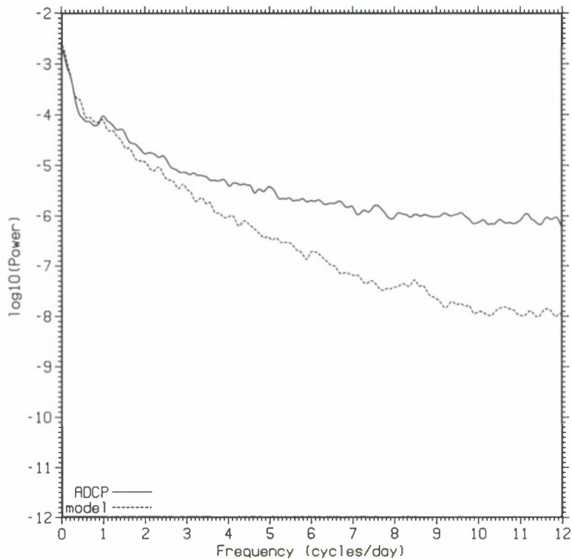
Figure 12. Power spectrum of detided model and ADCP current at GS2 at 20 m for period November 2005 through August 2006.
