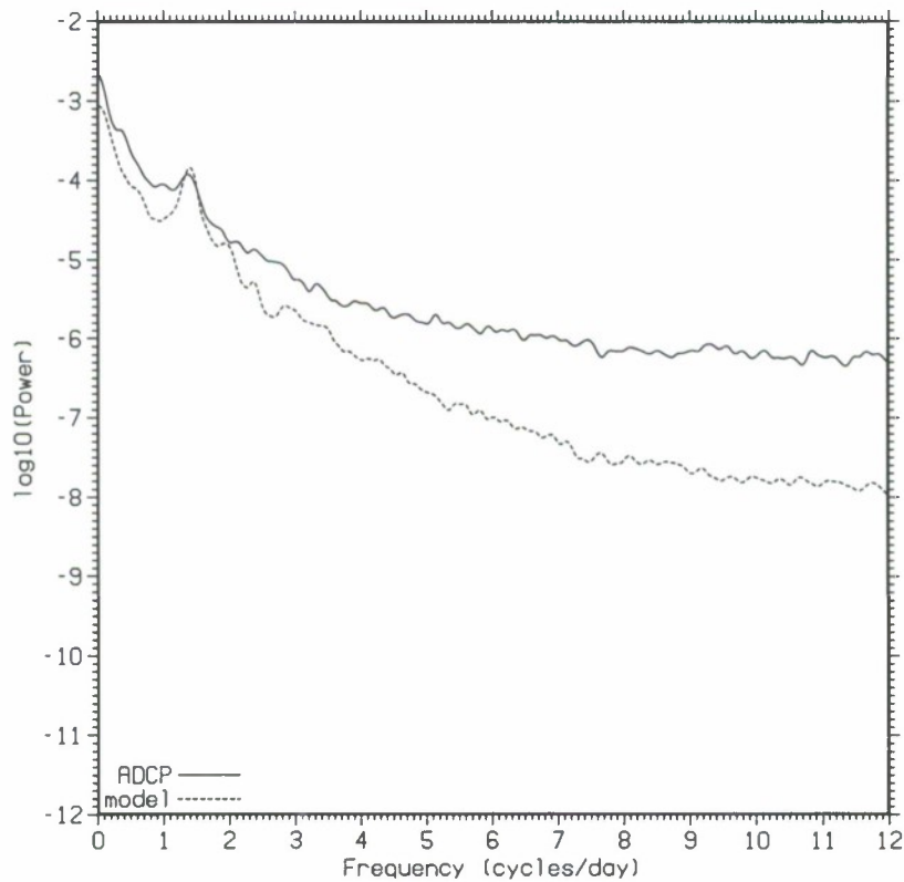
Figure 13. Power spectrum of detided model and ADCP current at GS10 at 20 m for period November 2005 through August 2006.
