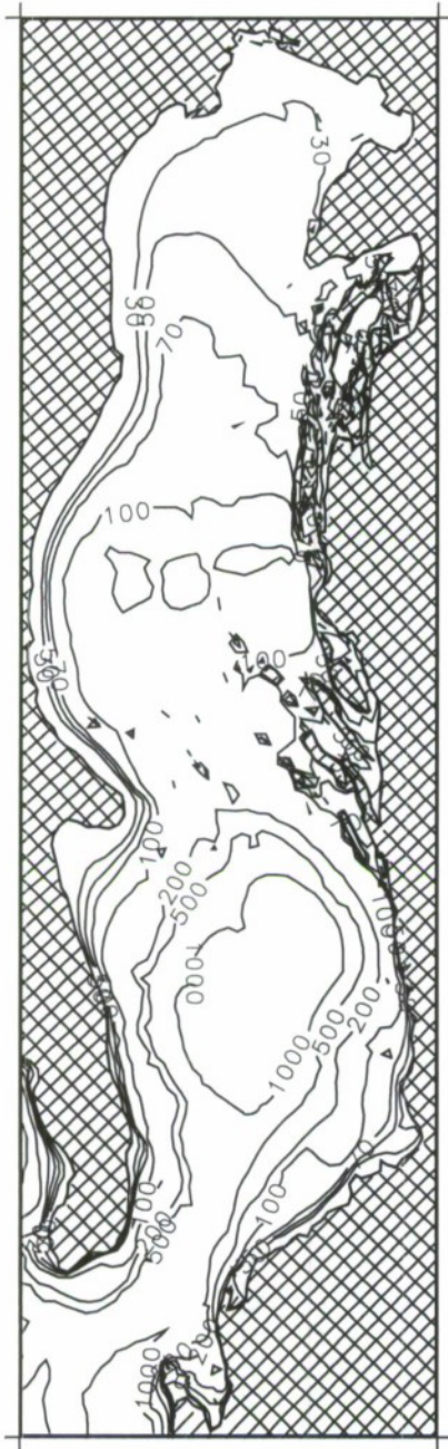
Figure 1. Model domain and bathymetry.
