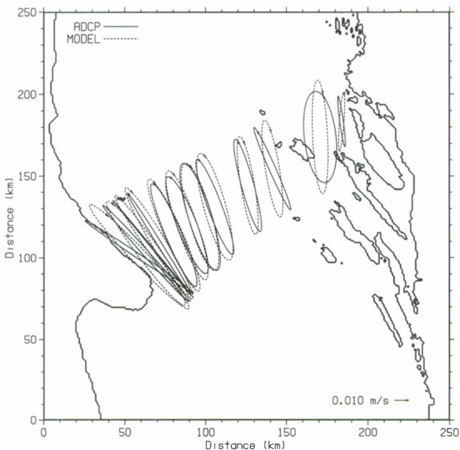
Figure 4. Model and ADCP K_1 tidal ellipses for depth-averaged current.
