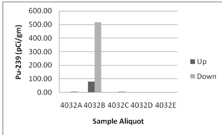
Figure 17. 4032 Aliquot Ratios
