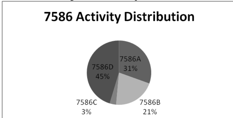
Figure 6. 7586 Activity Distribution
