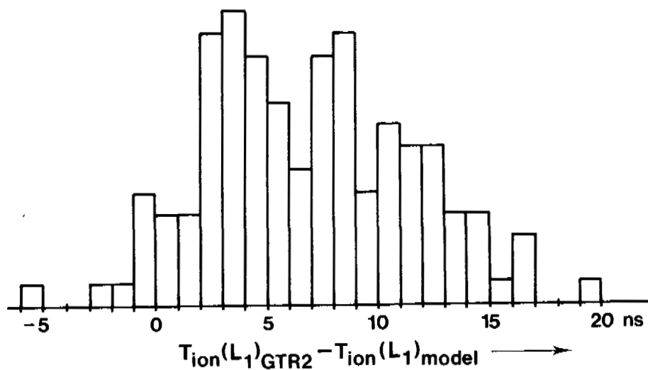
figure 3. Histogram of the values T_{ion(L_1)GTR2} - T_{ion(L_1)model} , obtained from 130 trackings for a five days period (no vertical conversion is applied) • T_{ion(L_1)GTR2} are GTR2 measurement • T_{ion(L_1)model} are the ionospheric compensation model estimations.
