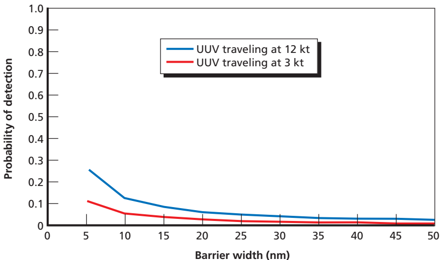
Figure 4.4 UUV Effectiveness in Hold at Risk
