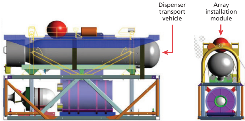
Figure 4.2 Array Installation Module and Dispenser Transport Vehicle
