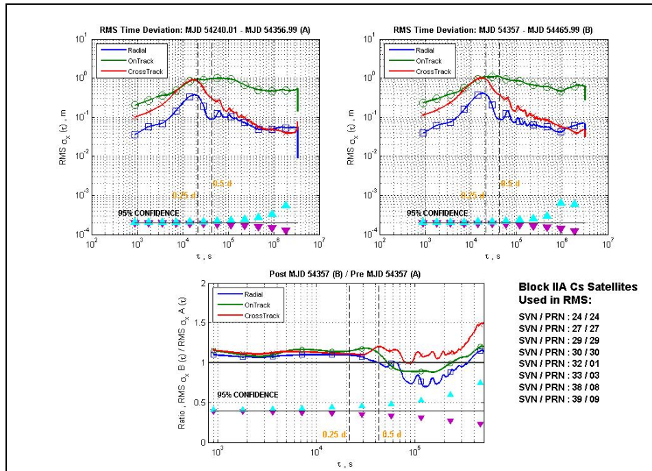
Figure 7. RMS TDEV ephemerides values taken over Block IIA satellites with Cs clocks. The upper left plot is before AEP, MJD 54357. The upper right plot is after. In the bottom plot, we have the ratio of TDEV values after AEP, divided by TDEV values from before.
