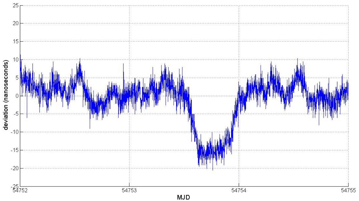
Figure 7. Ensemble response to failed cesium oscillator relative to UTC via GPS. To simulate the failure, the #1 cesium oscillator's internal phase microstepper was set to -2318 \times 10^{-15} (~200 ns/day).
