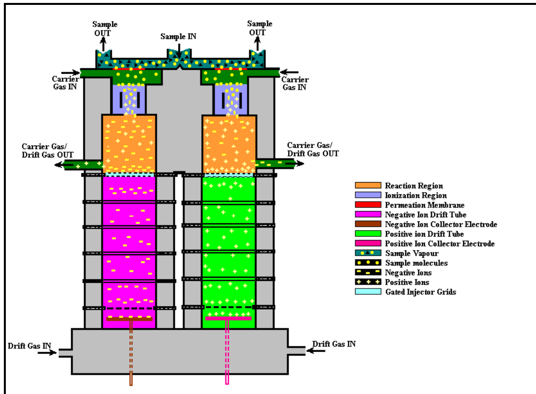
Figure 9: GID-3 schematic 61
