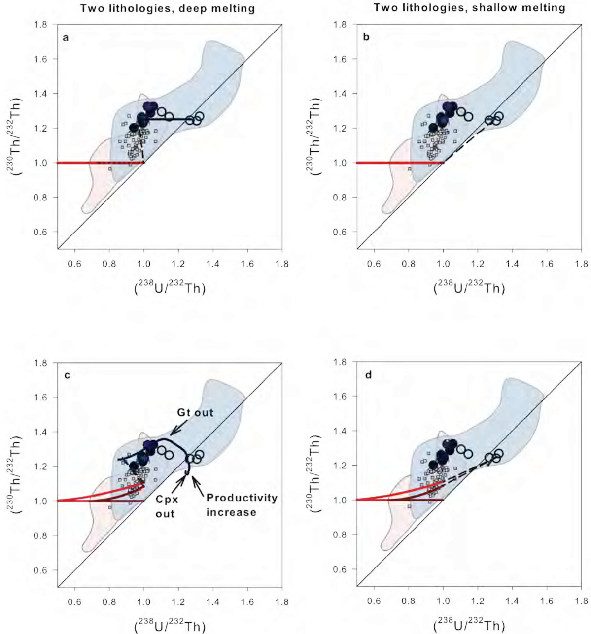
Appendix Figure 4. Equiline diagrams for the Kolbeinsey Ridge basalts, showing modeled melt trajectories for two mantle lithologies and binary melt mixing curves, as described in the Appendix. Garnet peridotite melting trajectories are shown in dark blue, spinel peridotite trajectories are green, eclogite melts are bright red lines, the trajectories for garnet pyroxenite are dark red lines, and binary mixtures are shown as dashed black lines; data symbols and fields as in Figure 6. (a) Deep melting column with time-independent melting; (b) shallow melting column with time-independent melting; (c) Deep melting column with time-dependent melting; (d) Shallow melting column with time-independent melting.
