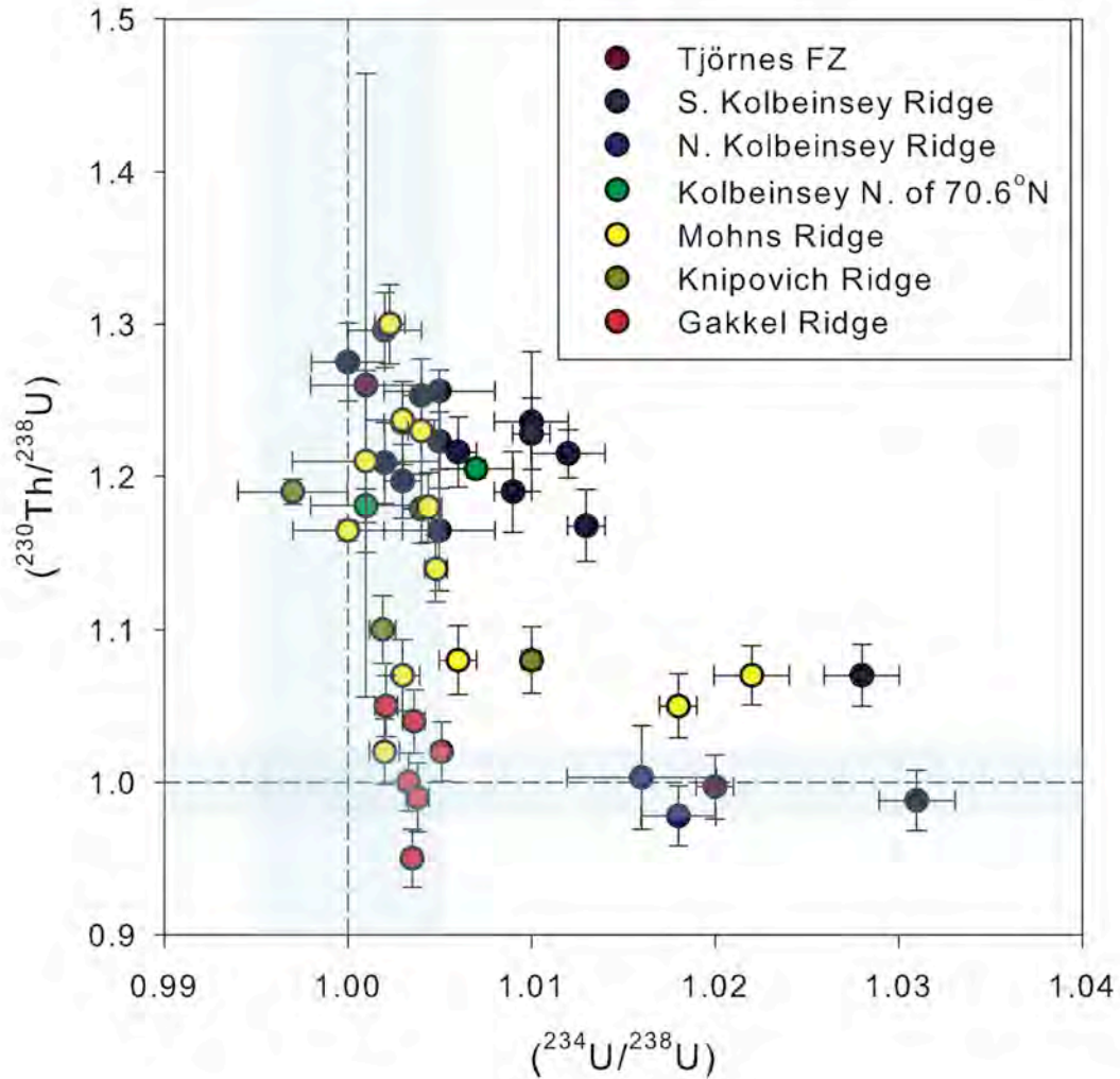
Figure 4. (^{234}\text{U}/^{238}\text{U}) vs. (^{230}\text{Th}/^{238}\text{U}) diagram showing results from Chapters 3 and 4. Unlike the Kolbeinsey Ridge (Chapter 3), the more northern ridges show less systematic patterns of seawater alteration.
