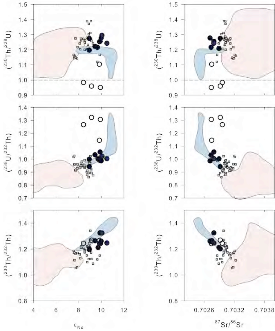
Figure 6. ( ^{230}\text{Th}/^{238}\text{U} ) (top panels), ( ^{232}\text{Th}/^{230}\text{Th} ) (middle panels), and ( ^{238}\text{U}/^{232}\text{Th} ) (bottom panels) for Kolbeinsey Ridge basalts, plotted versus radiogenic isotope ratios ^{87}\text{Sr}/^{86}\text{Sr} (left) and \epsilon_{\text{Nd}} (right). Data symbols and fields as in Figure 3, with potentially altered samples as open circles (Section 3.3.1.1). Kolbeinsey MORB are relatively homogeneous in ( ^{230}\text{Th}/^{232}\text{Th} ), ^{87}\text{Sr}/^{86}\text{Sr} , and \epsilon_{\text{Nd}} , but not ( ^{238}\text{U}/^{232}\text{Th} ) or ( ^{230}\text{Th}/^{238}\text{U} ), indicating that while ( ^{230}\text{Th}/^{232}\text{Th} ) reflects source composition, the amount of ^{238}\text{U} - ^{230}\text{Th} disequilibrium is not source-controlled. Overall, radiogenic isotopes vary very little along the Kolbeinsey Ridge.
