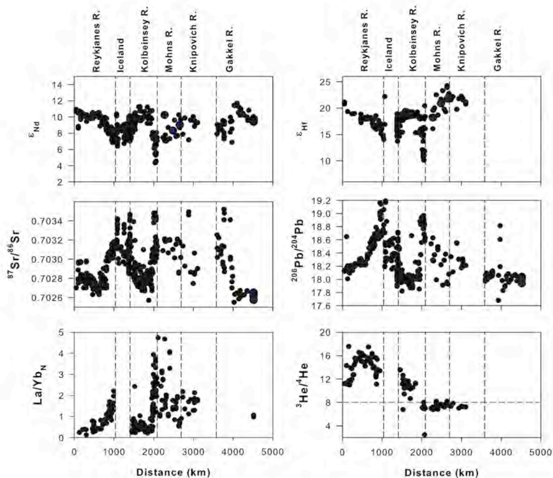
Figure 2. Distance along the Arctic ridge system vs. isotopic and trace element data in MORB (BLICHERT-TOFT et al., 2005; COHEN et al., 1980; CONDOMINES et al., 1981; DEVEY et al., 1994; DUPRE and ALLEGRE, 1980; FURMAN et al., 1991; GOLDSTEIN et al., 2008; HAASE et al., 2003; HANAN et al., 2000; HARDARSON and FITTON, 1997; HARDS et al., 1995; HEMOND et al., 1993; HILTON et al., 2000; MERTZ et al., 1991; MERTZ and HAASE, 1997; MURTON et al., 2002; NEUMANN and SCHILLING, 1984; O'NIONS and PANKHURS.RJ, 1973; PEATE et al., 2001; POREDA et al., 1986; SALTERS and WHITE, 1998; SCHILLING, 1975; SCHILLING et al., 1999; SCHILLING et al., 1983; SIGURDSSON, 1981; STECHER et al., 1999; STRACKE et al., 2006; STRACKE et al., 2003a; STRACKE et al., 2003b; SUN and JAHN, 1975; THIRLWALL et al., 2004; WAGGONER, 1989). New data from this study are shown as blue data points.
