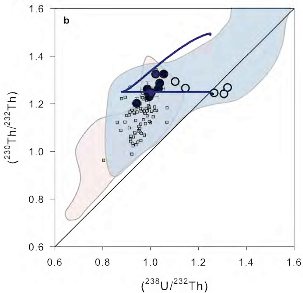
Appendix Figure 3. Equiline diagram for the Kolbeinsey Ridge basalts with a modeled garnet peridotite, continuously melting, dynamic melt trajectory (blue line), as described in the Appendix; data symbols and fields as in Figure 6.
