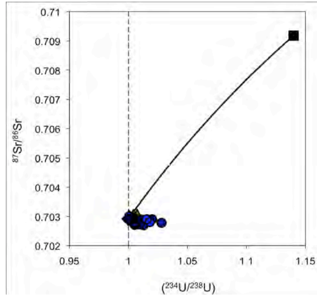
Figure 4. (a) (^{234}\text{U}/^{238}\text{U}) vs. (^{230}\text{Th}/^{238}\text{U}) for Kolbeinsey Ridge samples. Blue shaded regions are considered in equilibrium within analytical capabilities. The dotted black line shows a mixing trajectory between the average, unaltered Kolbeinsey Ridge sample and seawater with (^{230}\text{Th}/^{238}\text{U}) = 1.0 and (^{234}\text{U}/^{238}\text{U}) = 1.14 , as described in the text. A simple linear fit to the Kolbeinsey data, as described in the text, is shown with a widely dashed line. (b) (^{234}\text{U}/^{238}\text{U}) vs. ^{87}\text{Sr}/^{86}\text{Sr} , showing samples from this study. The black square data point represents seawater, using isotopic compositions from Faure and Mensing (2005). The heavy black line shows a mixing trajectory between sample 1093 (the Kolbeinsey sample with (^{234}\text{U}/^{238}\text{U}) nearest to equilibrium) and seawater. U and Sr concentrations in seawater also from Faure and Mensing (2005).
