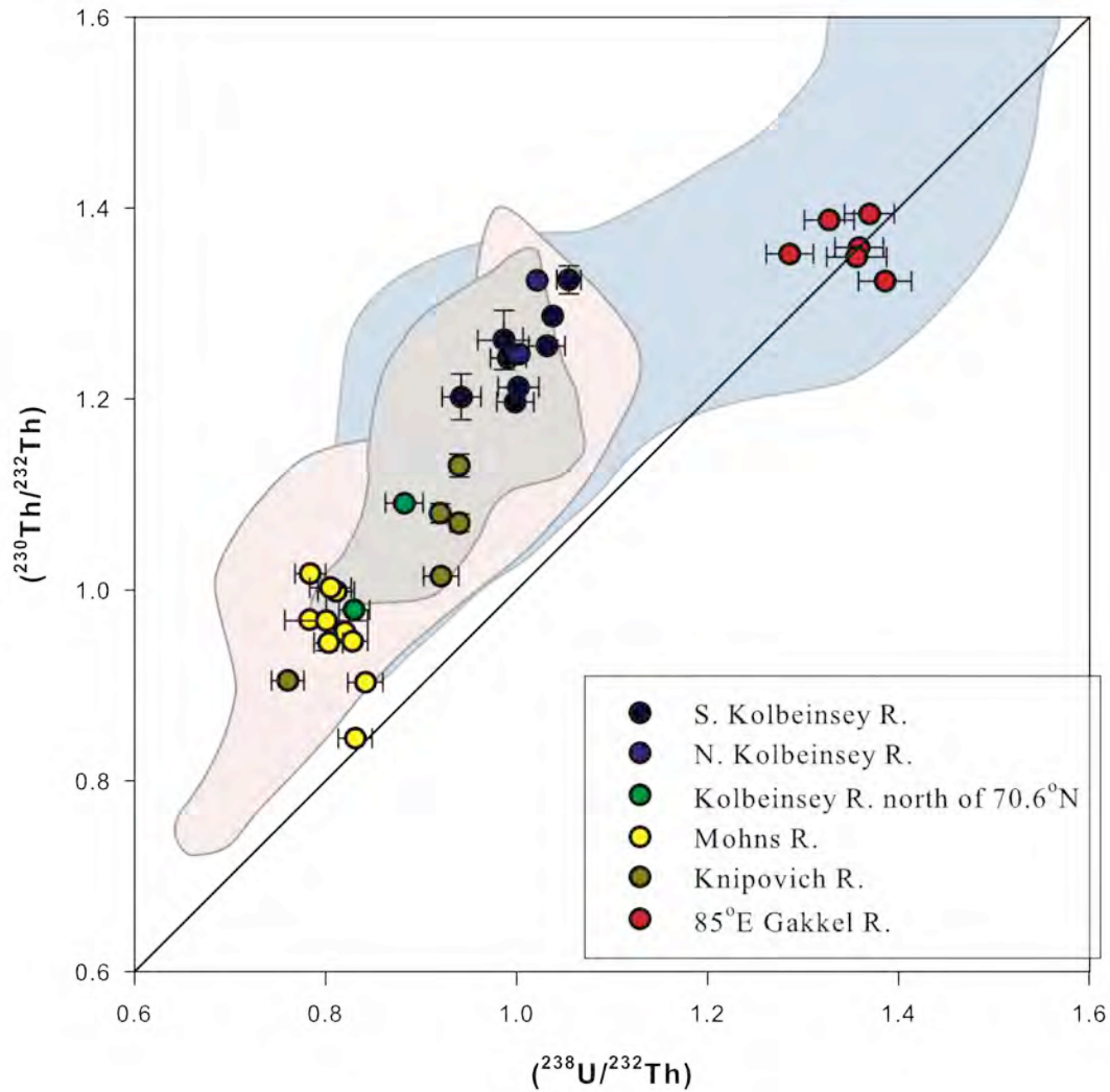
Figure 3. (^{238}\text{U}/^{232}\text{Th}) vs. (^{230}\text{Th}/^{232}\text{Th}) "equiline" diagram showing data from Chapter 3 (Kolbeinsey Ridge data points) and this study (Mohns Ridge, Knipovich Ridge, and Gakkel Ridge data), with global MORB (BOURDON et al., 1996a; GOLDSTEIN et al., 1989; GOLDSTEIN et al., 1992; GOLDSTEIN et al., 1993; LUNDSTROM et al., 1999; PEATE et al., 2001; SIMS et al., 1995; SIMS et al., 2002; STURM et al., 2000; TEPLY et al., 2004), OIB (BOURDON et al., 1998; CLAUDE-IVANAJ et al., 1998; CLAUDE-IVANAJ et al., 2001; PIETRUSZKA et al., 2001; SIGMARSSON et al., 1998; SIMS et al., 1999a; SIMS et al., 1995; SIMS and HART, 2006; SIMS et al., 2008; TURNER et al., 1997; WIDOM et al., 1997), and Iceland (KOKFELT et al., 2003; STRACKE et al., 2003a; STRACKE et al., 2003b) fields in blue, red, and gray for comparison, respectively. Samples from north of 70.6^\circ\text{N} on the Kolbeinsey Ridge, which are enriched and isotopically distinct, are separated from the rest of the Kolbeinsey data and more closely resemble Mohns Ridge and Knipovich Ridge samples. These northern Kolbeinsey samples and the Knipovich Ridge data both form sloped arrays. Age-constrained Mohns Ridge ^{238}\text{U} - ^{230}\text{Th} data (Table 2; see Section 4.4) cluster tightly at the enriched end of these arrays. Gakkel Ridge samples are highly depleted and homogeneous and range from 5% ^{230}\text{Th} excess to 5% ^{238}\text{U} excess.
