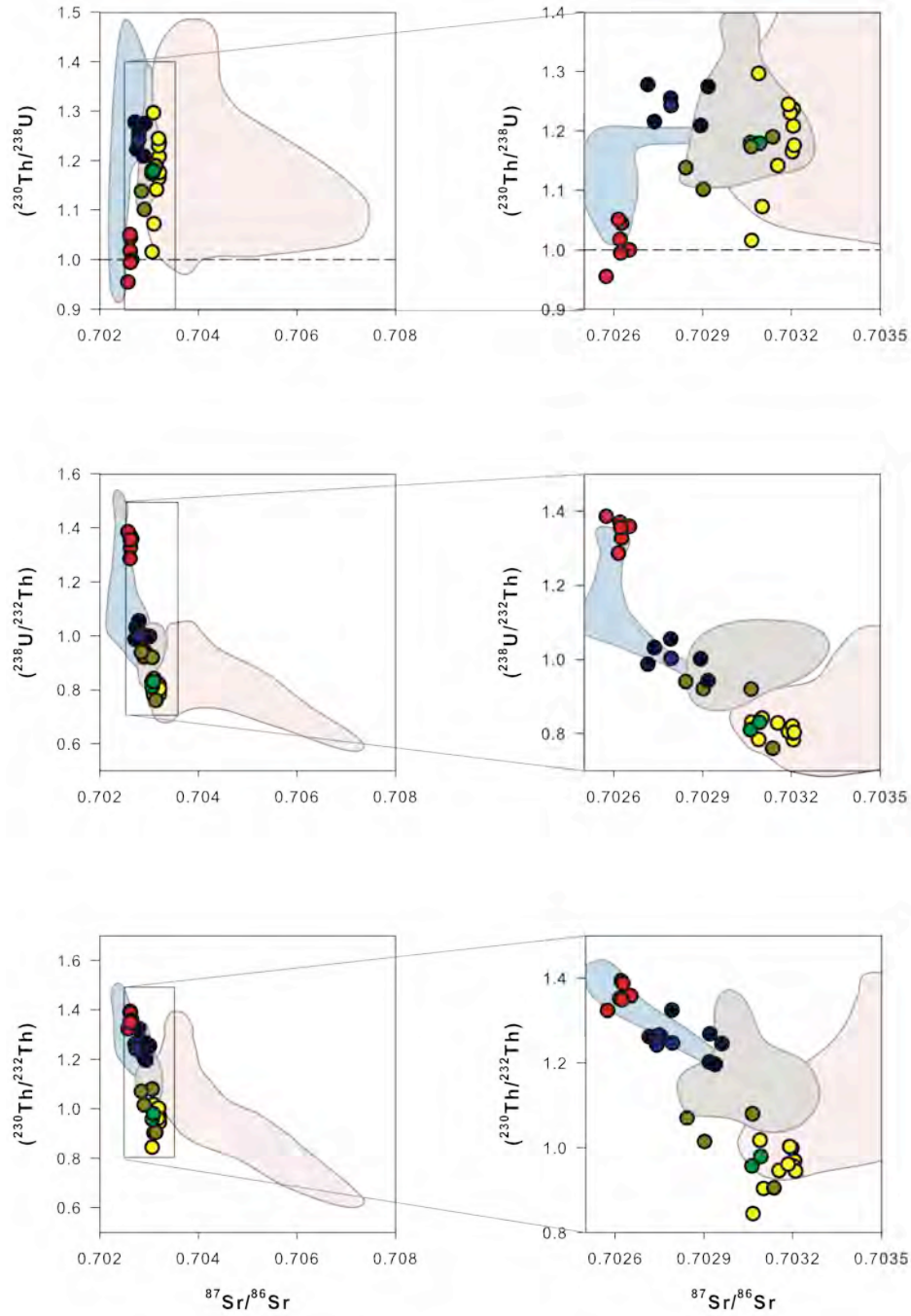
Figure 7. ^{87}\text{Sr}/^{86}\text{Sr} vs. (^{230}\text{Th}/^{232}\text{Th}) (top panels), (^{238}\text{U}/^{232}\text{Th}) (middle panels), and (^{230}\text{Th}/^{238}\text{U}) (bottom panels), with symbols as in Figure 3; radiogenic isotope data from this study and the literature (BLICHERT-TOFT et al., 2005; HANAN et al., 2000; NEUMANN and SCHILLING, 1984; SCHILLING et al., 1999; SCHILLING et al., 1983; SIGURDSSON, 1981; WAGGONER, 1989). The position on the sloped array for Knipovich Ridge (e.g. (^{238}\text{U}/^{232}\text{Th}) ) does form a correlation, indicating that source composition may control the slope of the array shown in Figure 3. Gakkel Ridge samples are universally isotopically depleted.
