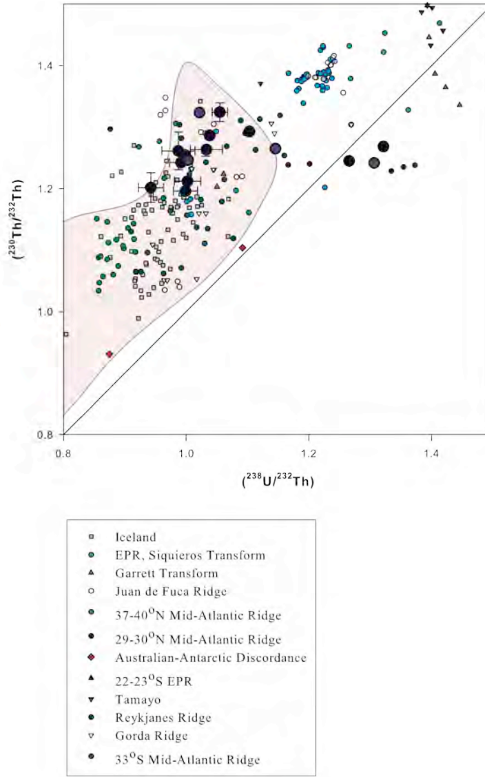
Figure 3. (^{230}\text{Th}/^{232}\text{Th}) versus (^{238}\text{U}/^{232}\text{Th}) “equiline” diagram for measured basalts from Kolbeinsey Ridge, with the exception of sample TR139 1D-1g ( (^{238}\text{U}/^{232}\text{Th}) = 1.00 , (^{230}\text{Th}/^{232}\text{Th}) = 1.25 ), because its large error bars make it difficult to view the rest of the data. For comparison we show (a) fields for global MORB data in blue (BOURDON et al., 1996a; GOLDSTEIN et al., 1989; GOLDSTEIN et al., 1992; GOLDSTEIN et al., 1993; LUNDSTROM et al., 1999; PEATE et al., 2001; SIMS et al., 1995; SIMS et al., 2002; STURM et al., 2000; TEPLEY et al., 2004), global ocean island basalt (OIB) data in red (except for Iceland) (BOURDON et al., 1998; CLAUDE-IVANAJ et al., 1998; CLAUDE-IVANAJ et al., 2001; PIETRUSZKA et al., 2001; SIGMARSSON et al., 1998; SIMS et al., 1999a; SIMS et al., 1995; SIMS and HART, 2006; SIMS et al., 2008b; TURNER et al., 1997; WIDOM et al., 1997), and Icelandic data in gray (KOKFELT et al., 2003; STRACKE et al., 2003a; STRACKE et al., 2003b), (b) the same data, broken down by determination of seawater alteration from measurements of (^{234}\text{U}/^{238}\text{U}) , and (c) a field for global OIB data, with individual data points for Iceland and global MORB. The Kolbeinsey Ridge data form a horizontal array that overlaps with Icelandic samples at the high (^{230}\text{Th}/^{238}\text{U}) end and extends to (^{230}\text{Th}/^{238}\text{U}) < 1 .
