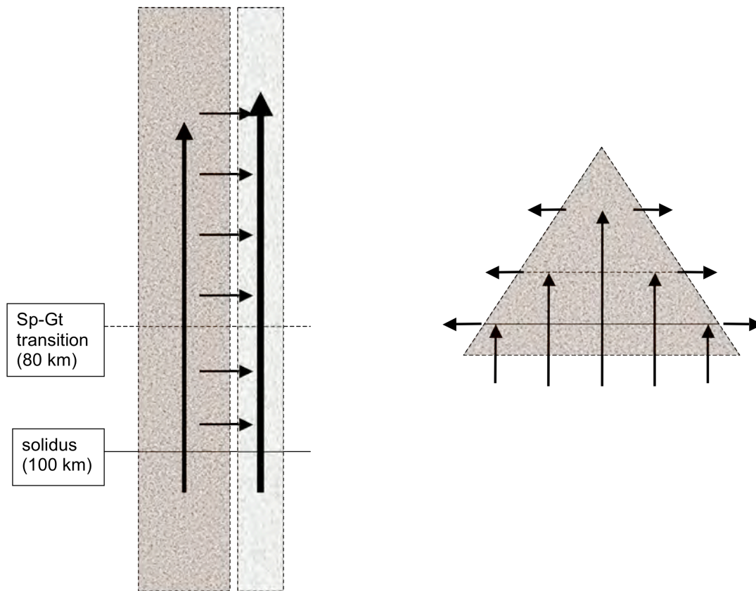
Appendix Figure 1. Schematic conceptual diagrams for two-porosity and two-dimensional melt transport regimes. On the left is a two-column melt regime, where equilibrium melts are produced in a low-porosity upwelling regime and then extracted into an adjacent, higher-porosity column, where they experience disequilibrium transport. On the right is a two-dimensional, triangular melting regime for a mid-ocean ridge setting, after Langmuir et al. (1992).
