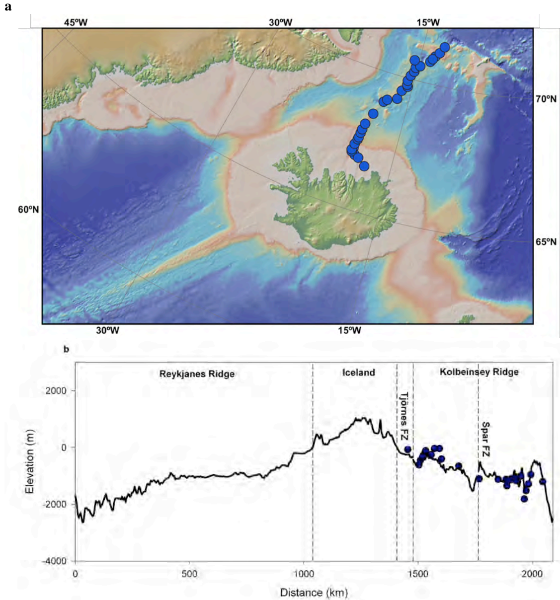
Figure 1. (a) Map of the field area, showing the locations of all samples examined in this study, with bathymetry from Smith and Sandwell (1997) and Jakobsson et al. (2008). (b) A depth profile for the Reykjanes Ridge, Iceland, and the Kolbeinsey Ridge, with Kolbeinsey Ridge sample locations as bold blue circles.
