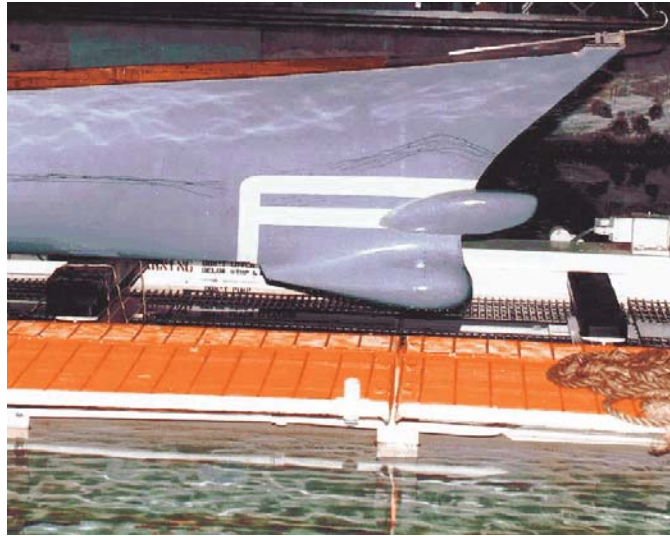
Figure D-I. Near-Surface Bow Bulb Design for DDG-51
