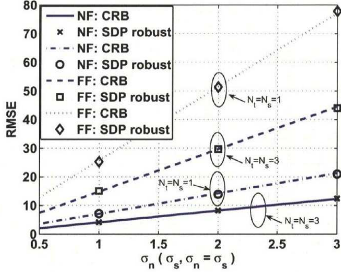
Figure 3. RMSE of target location estimation versus the measurement noise and node location error in the near and far field cases, where ‘NF’ stands for ‘near field case’, and ‘FF’ stands for ‘far field case’.
