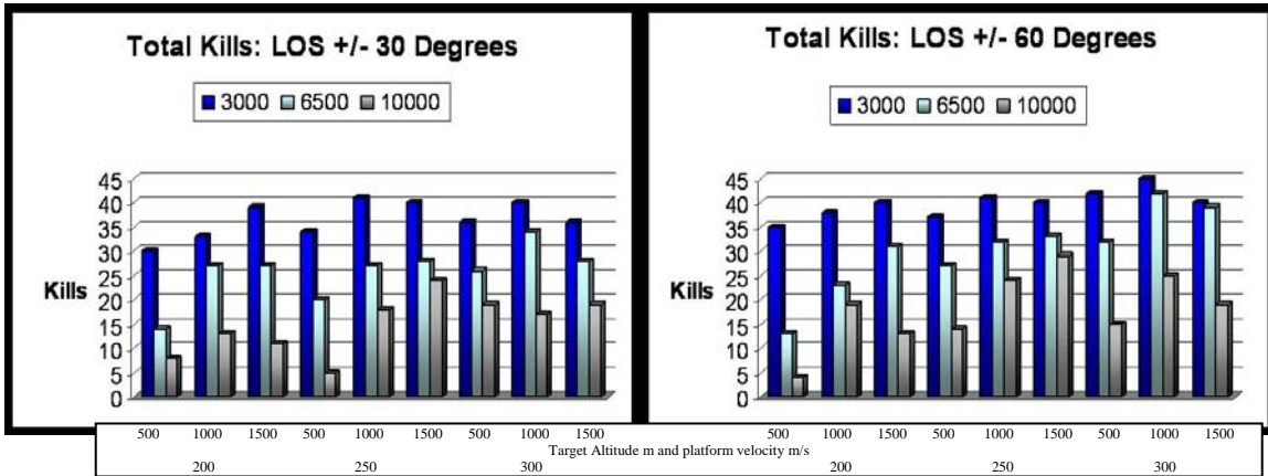
Figure 19. Total Kills over all Factor Settings
