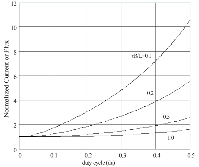
Fig.3: Normalized Maximum Current or Flux vs Duty Cycle for Values of \tau R/L
