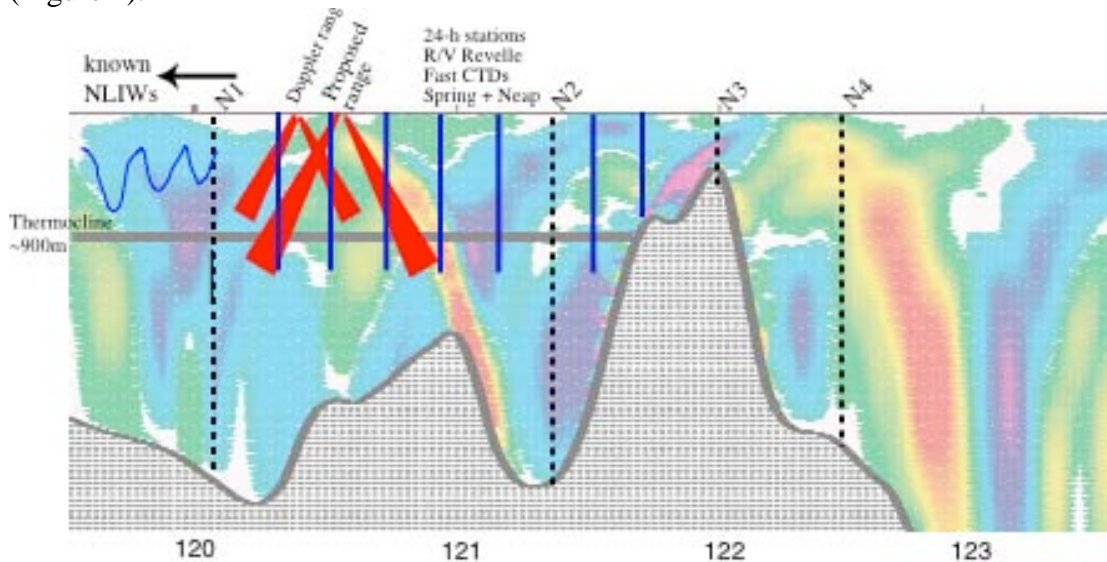
Figure 2. A cross section of the SCS, showing an instantaneous velocity pattern from the baroclinic tide, as generated by barotropic flow over the topography. The reach of the Revelle FCTD and sonar is shown to approximate scale. The depth-time reach of the system was appropriate to the scale of the phenomenon studied.
